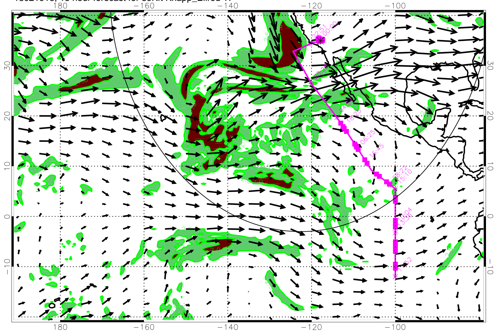
13021918, 18 hour forecast for 39Kft Knapp_Ellrod TI
