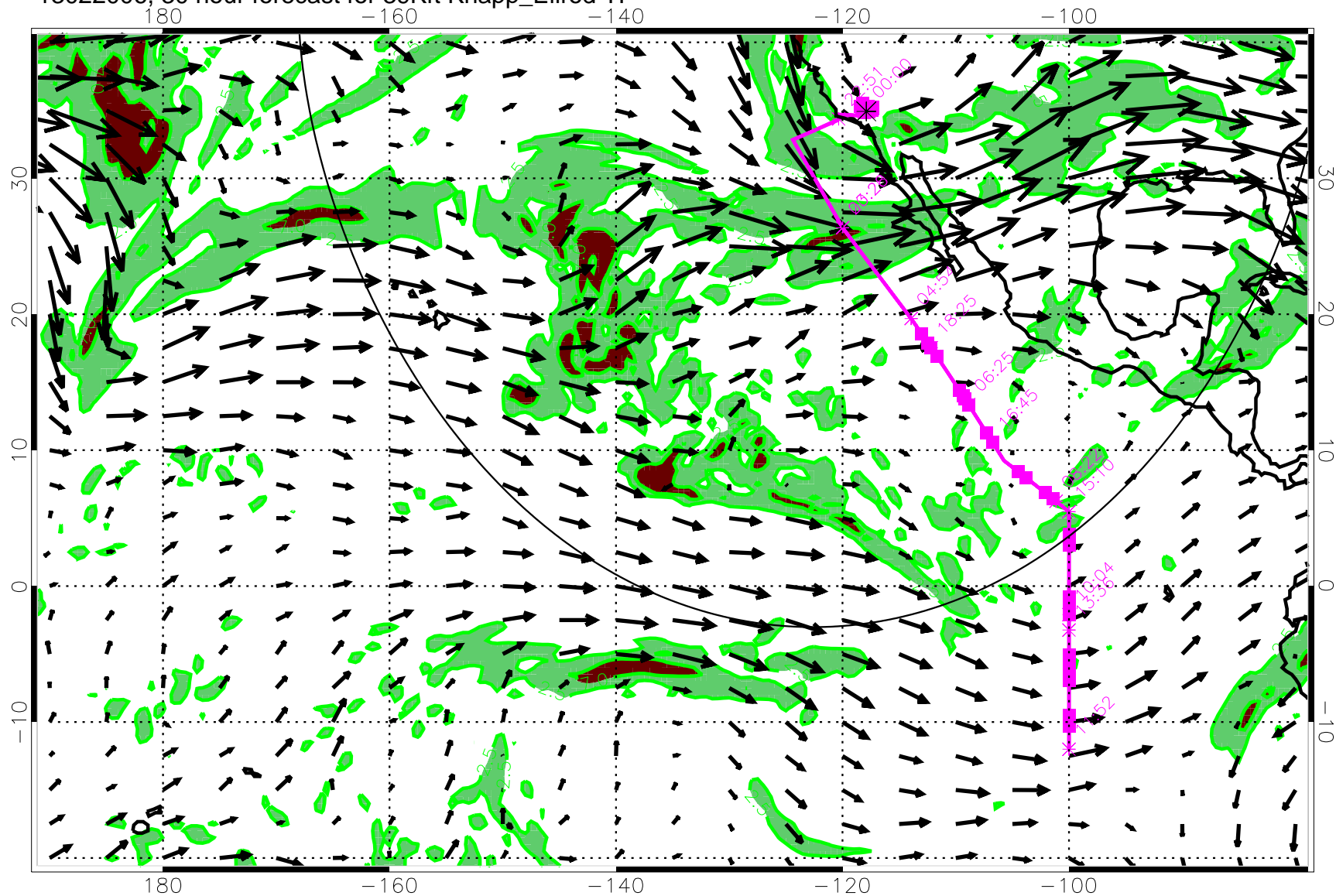
13022006, 30 hour forecast for 39Kft Knapp_Ellrod TI
