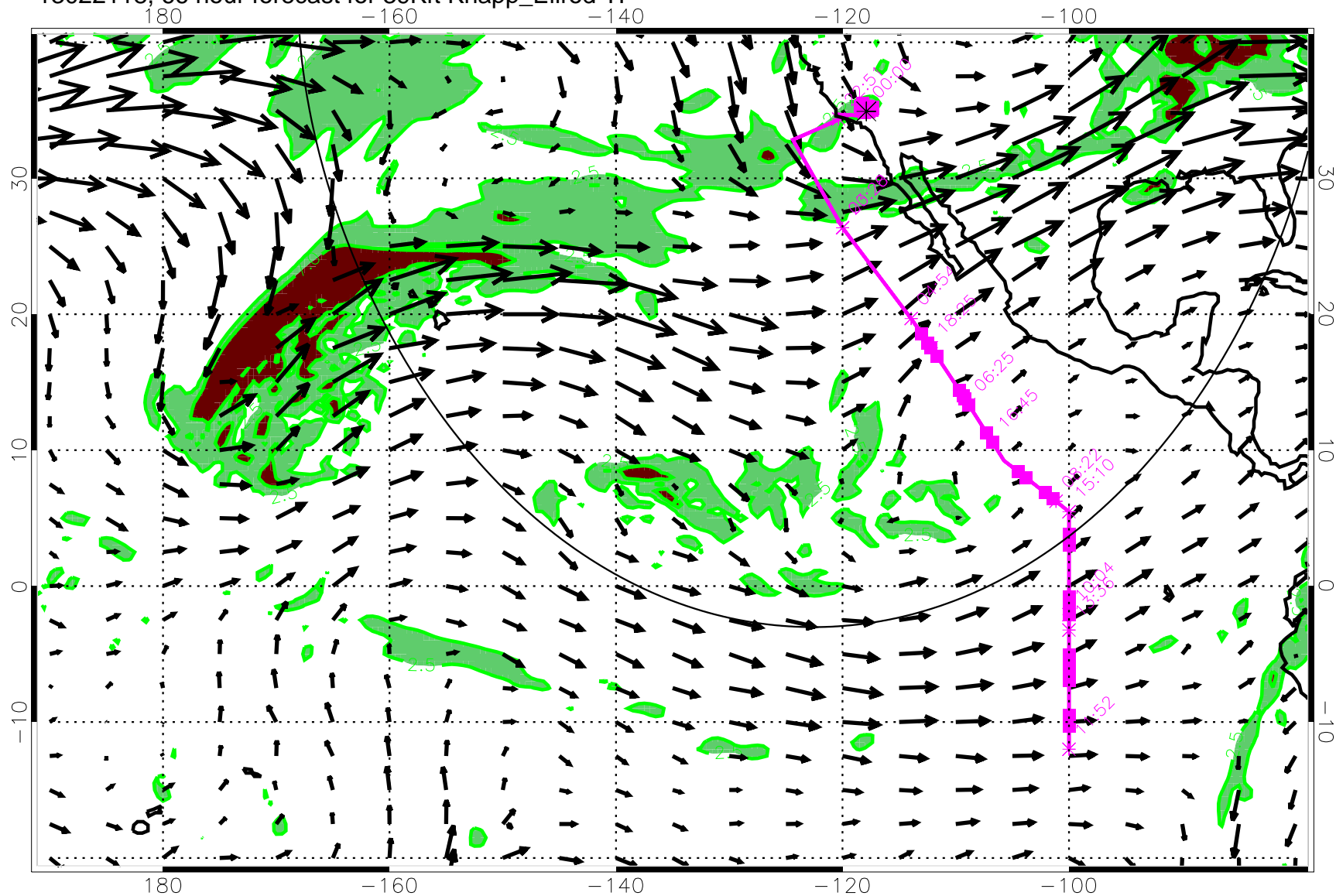
13022118, 66 hour forecast for 39Kft Knapp_Ellrod TI
