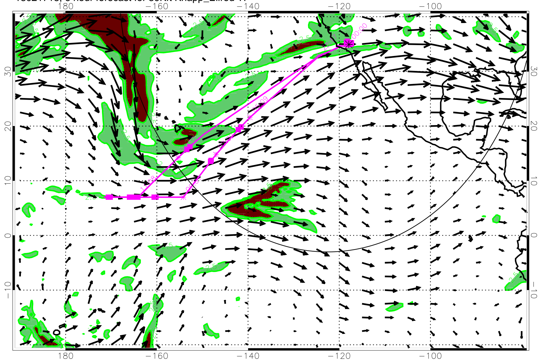
13021718, 6 hour forecast for 39Kft Knapp_Ellrod TI
