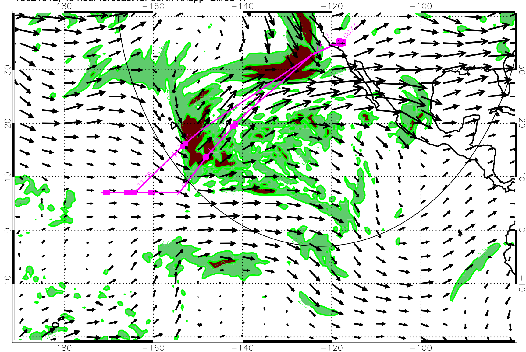
13021912, 48 hour forecast for 39Kft Knapp_Ellrod TI
