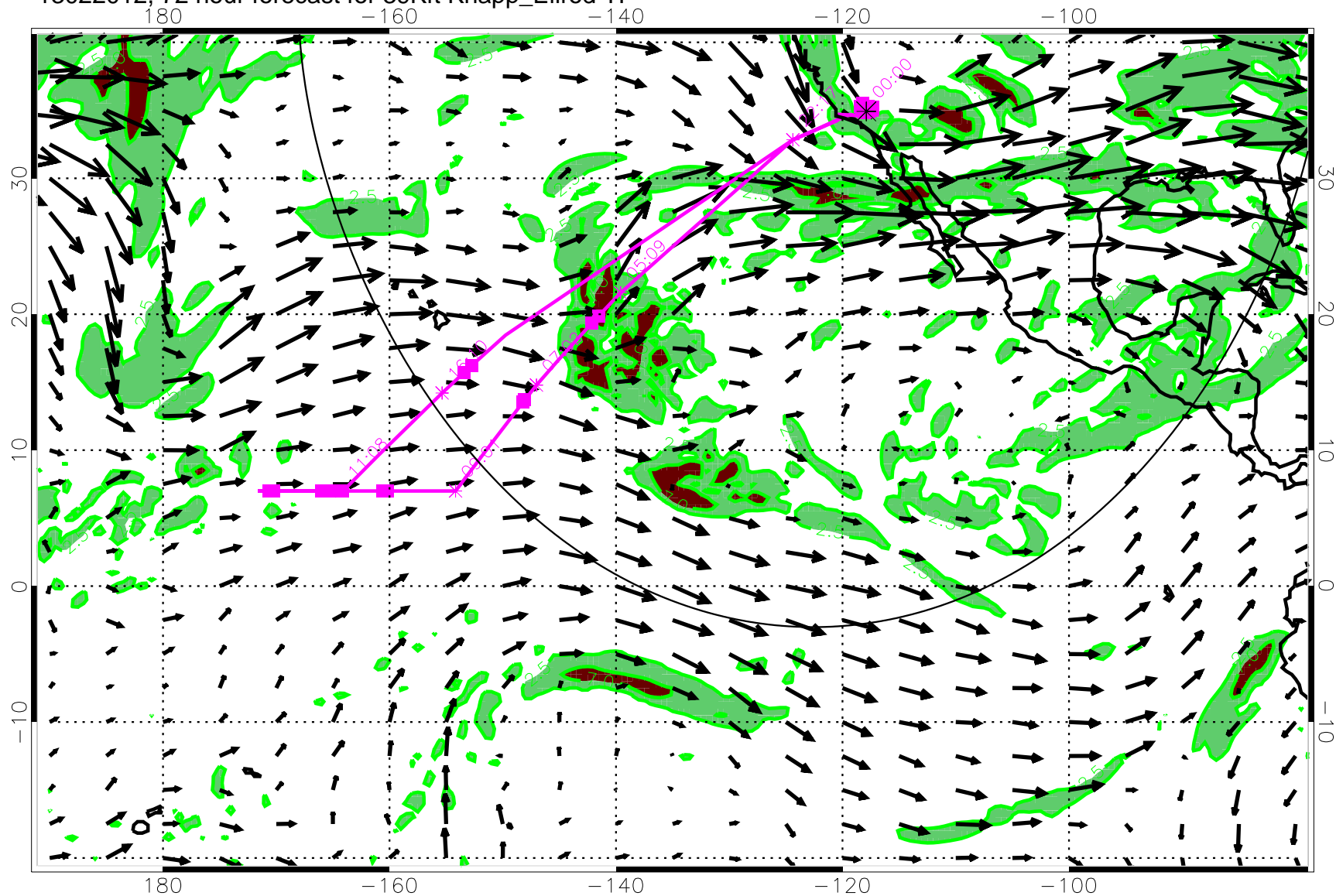
13022012, 72 hour forecast for 39Kft Knapp_Ellrod TI
