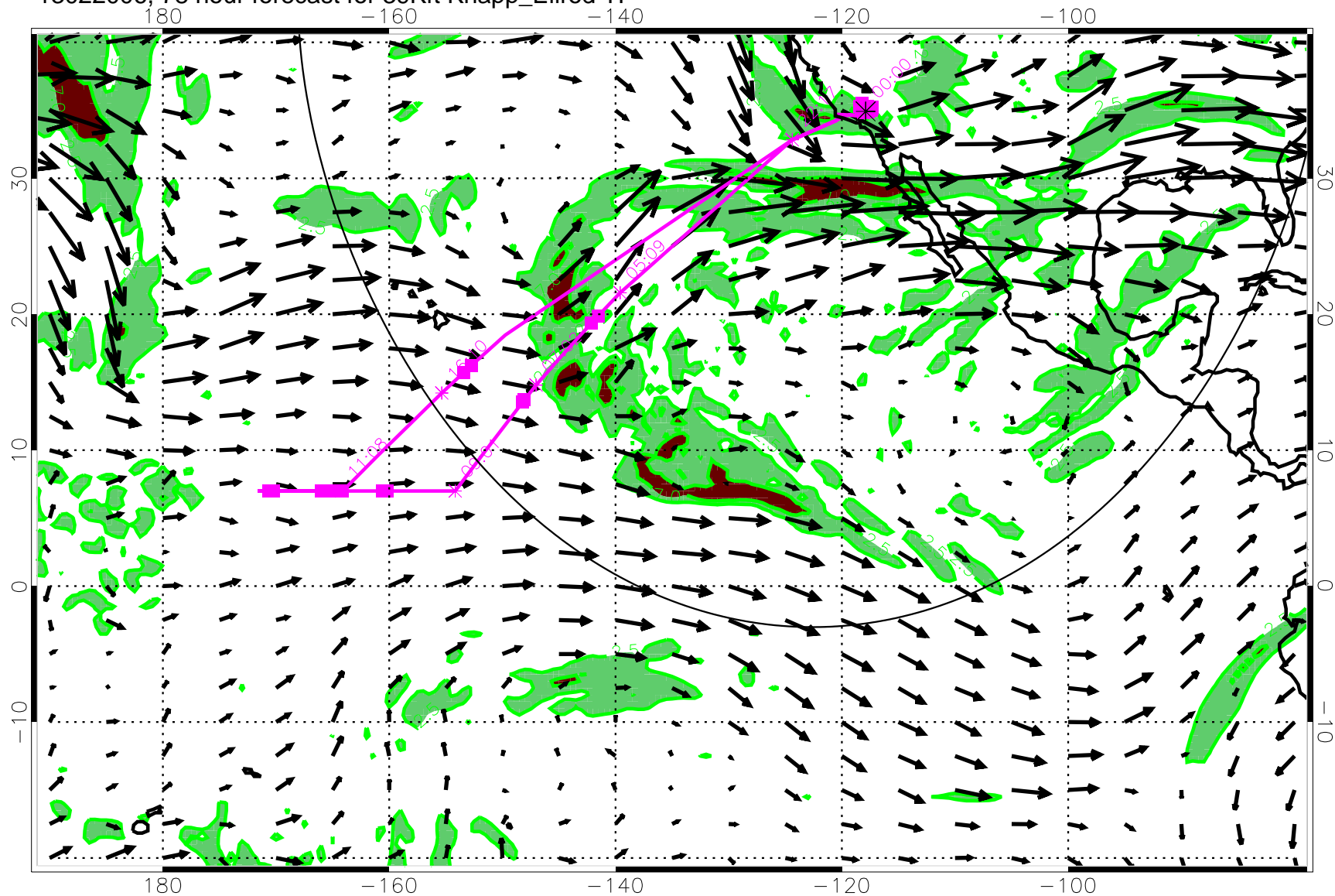
13022006, 78 hour forecast for 39Kft Knapp_Ellrod TI
