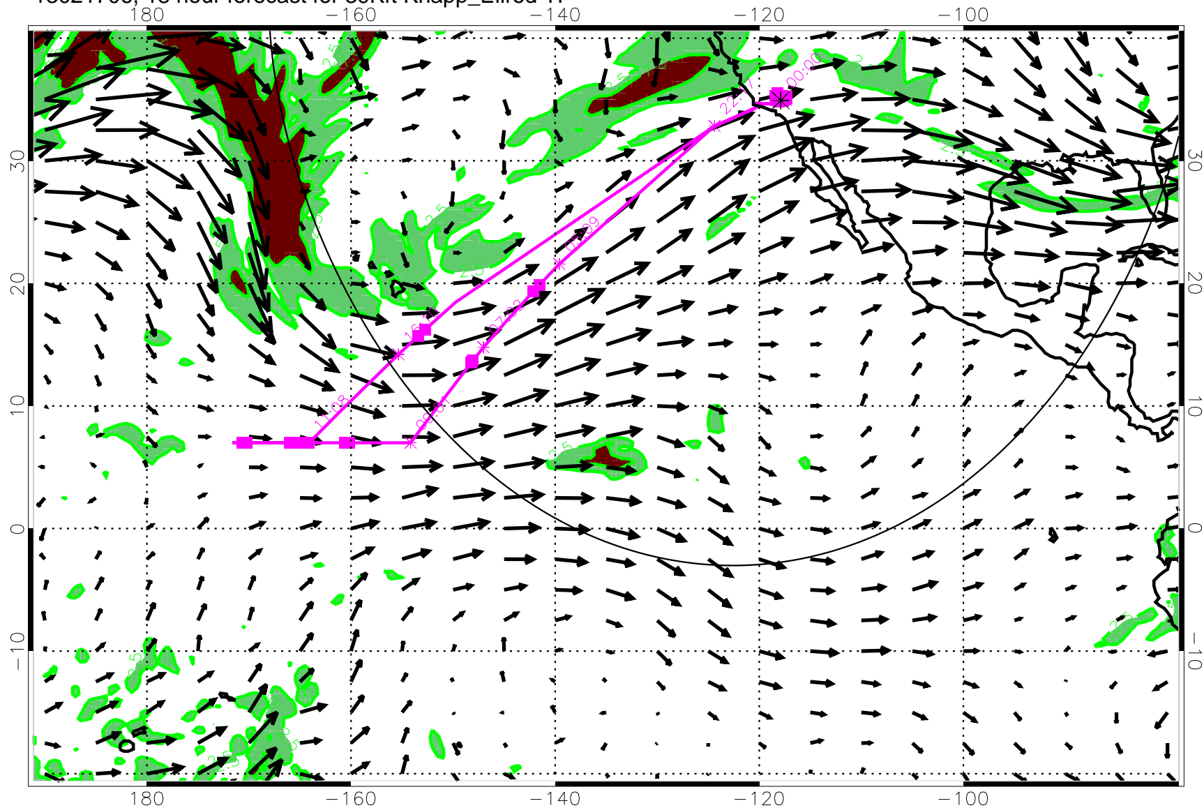
13021706, 18 hour forecast for 39Kft Knapp_Ellrod TI
