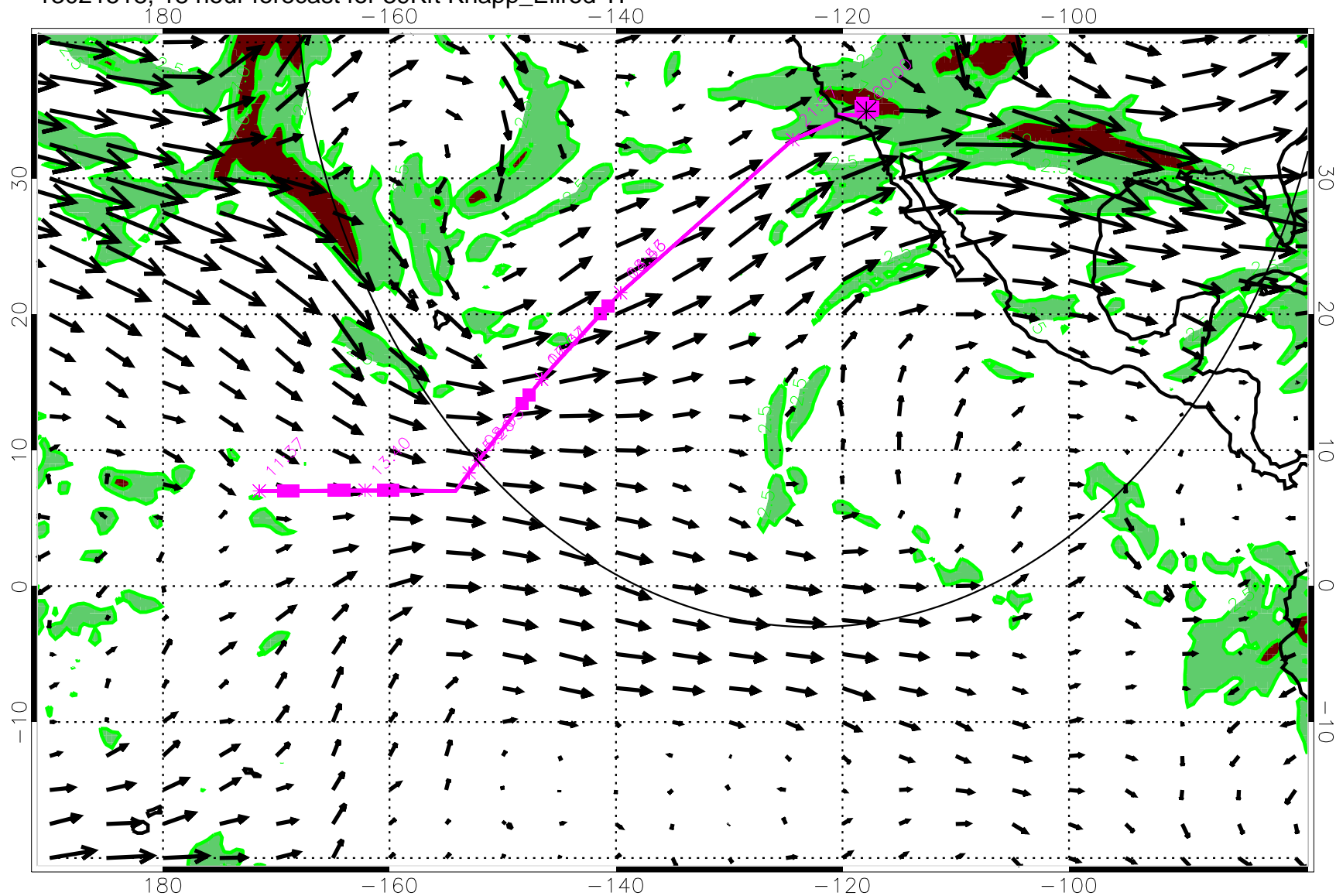
13021518, 18 hour forecast for 39Kft Knapp_Ellrod TI
