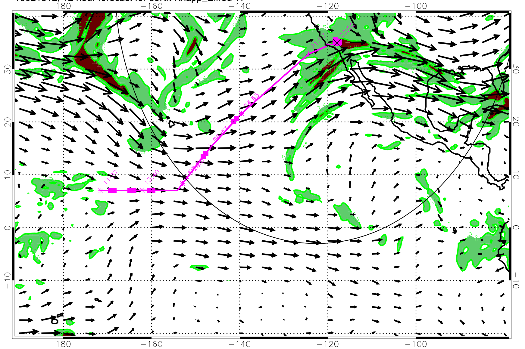
13021512, 12 hour forecast for 39Kft Knapp_Ellrod TI
