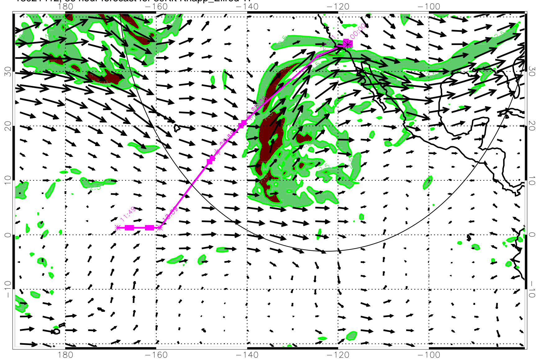
13021412, 36 hour forecast for 39Kft Knapp_Ellrod T1
