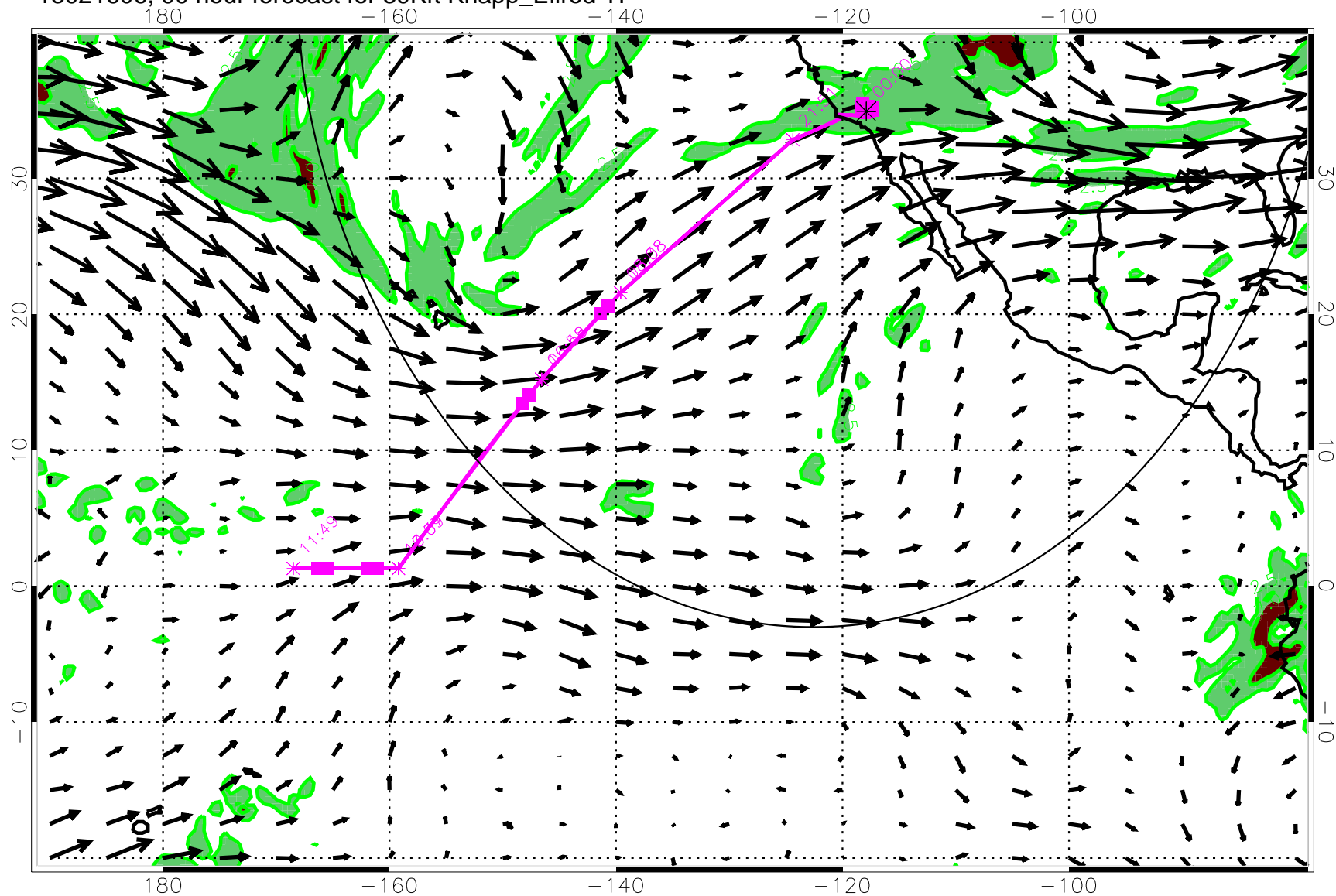
13021606, 90 hour forecast for 39Kft Knapp_Ellrod T1
