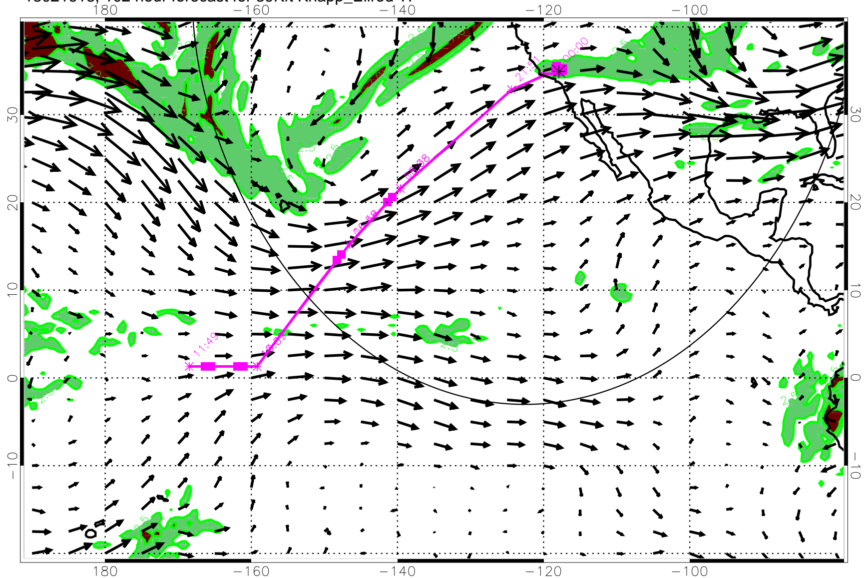
13021618, 102 hour forecast for 39Kft Knapp_Ellrod T1
