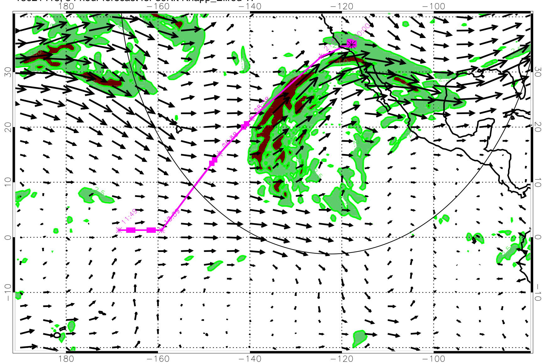
13021418, 54 hour forecast for 39Kft Knapp_Ellrod TI
