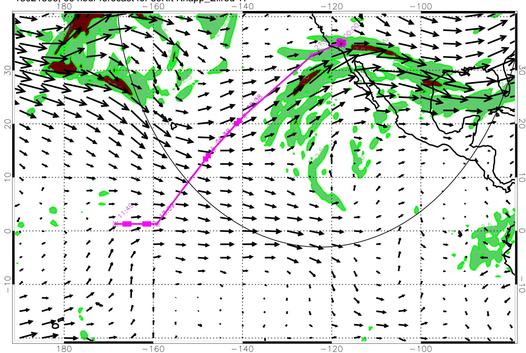
13021506, 66 hour forecast for 39Kft Knapp_Ellrod TI
