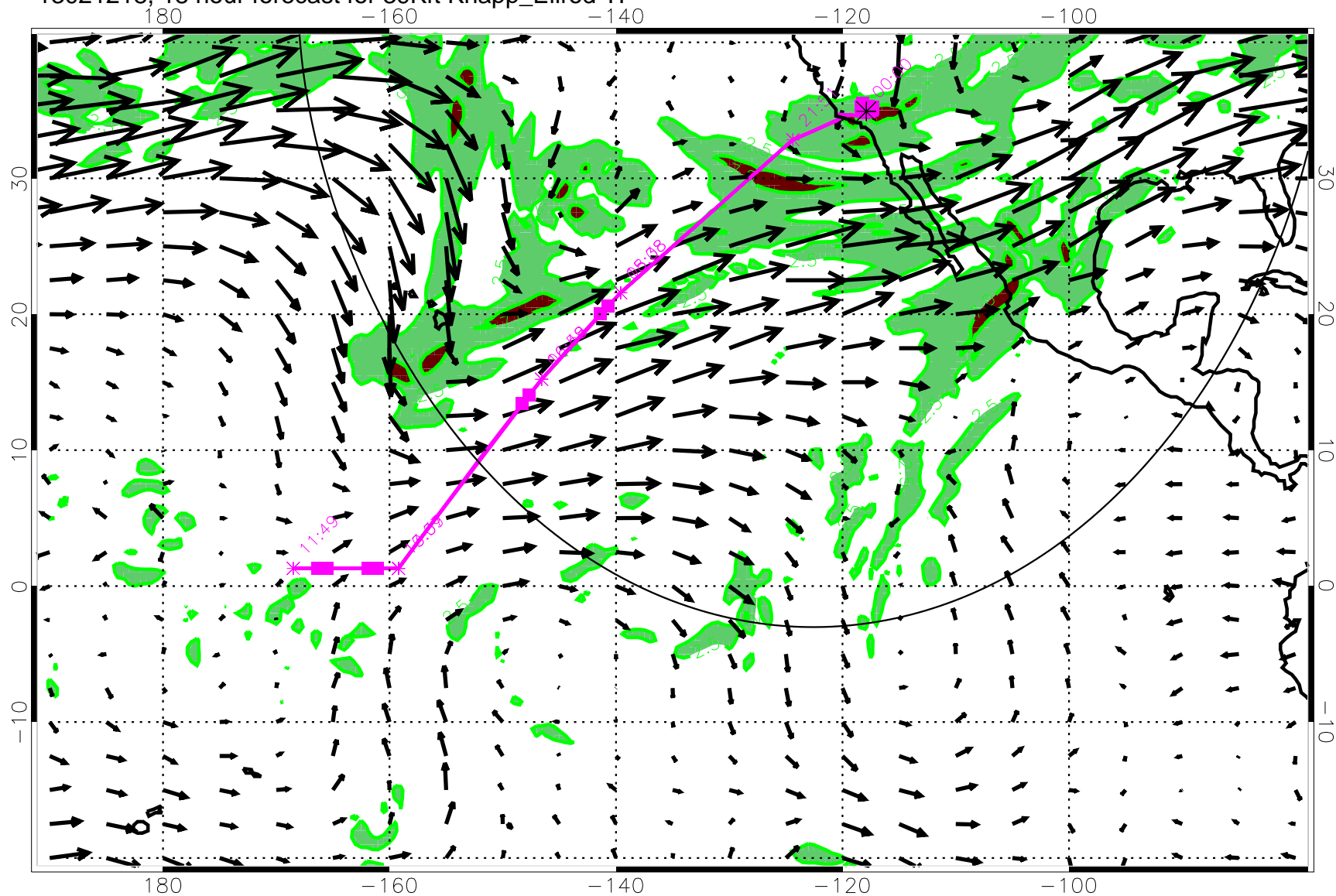
13021218, 18 hour forecast for 39Kft Knapp_Ellrod TI
