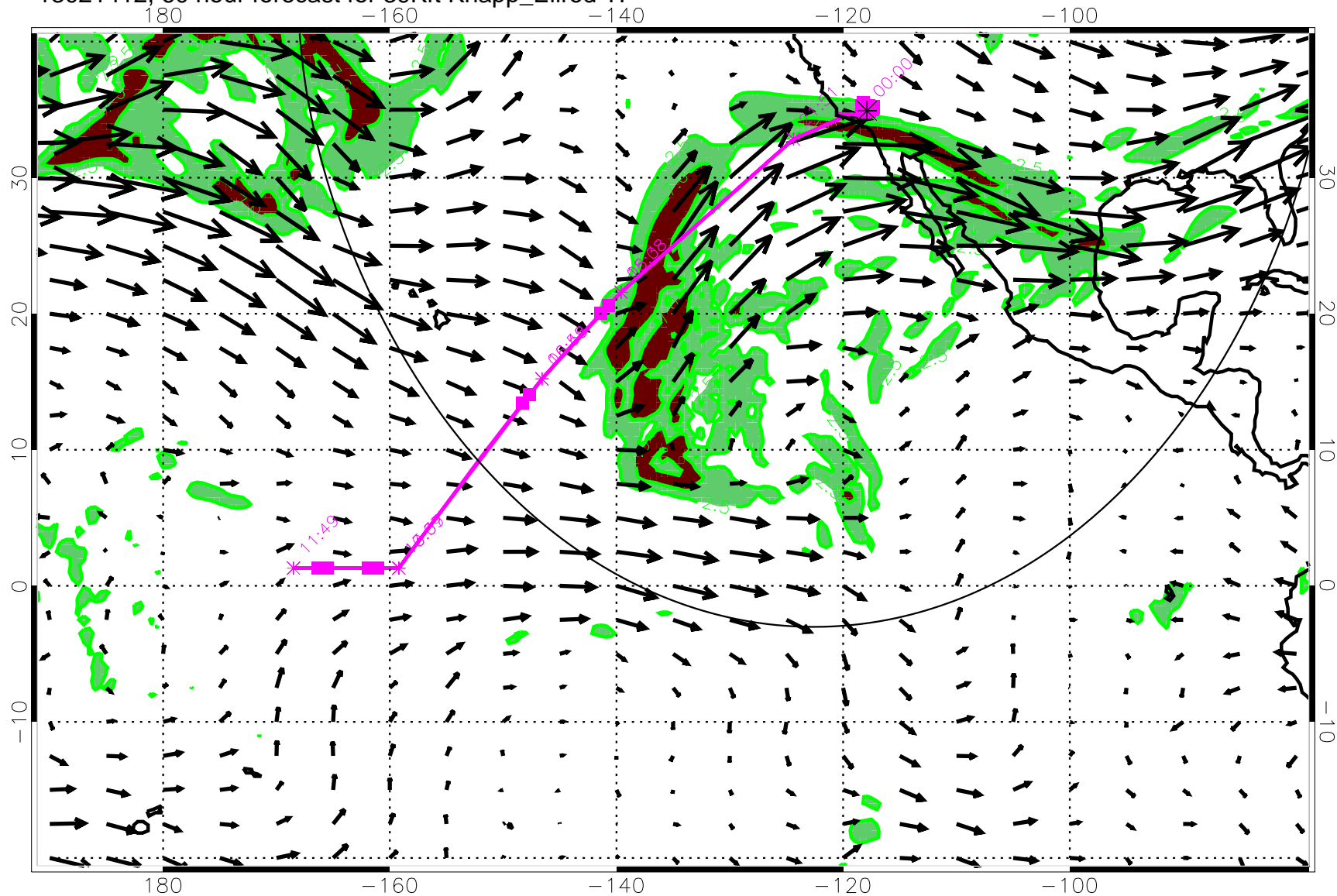
13021412, 60 hour forecast for 39Kft Knapp_Ellrod TI
