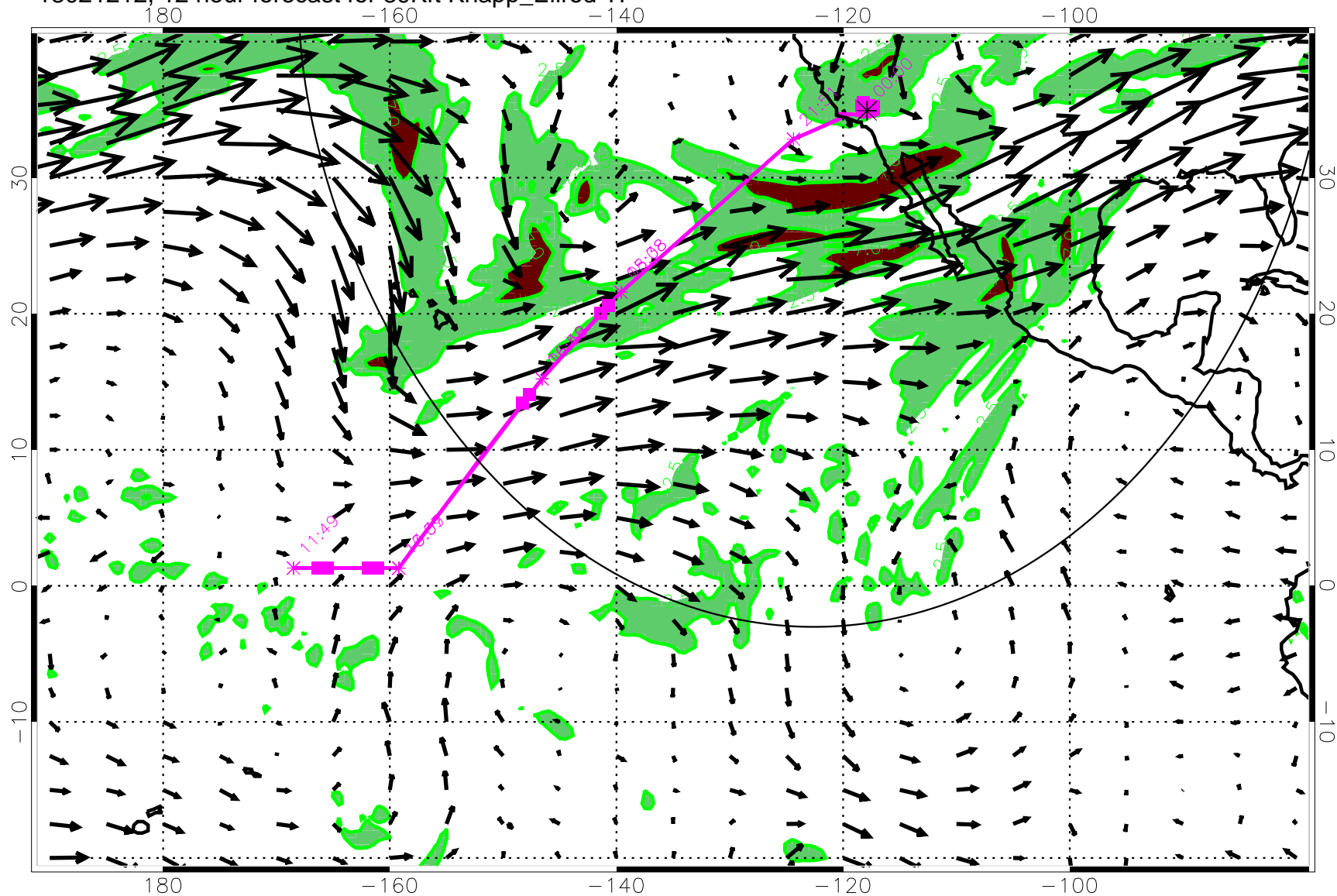
13021212, 12 hour forecast for 39Kft Knapp_Ellrod TI
