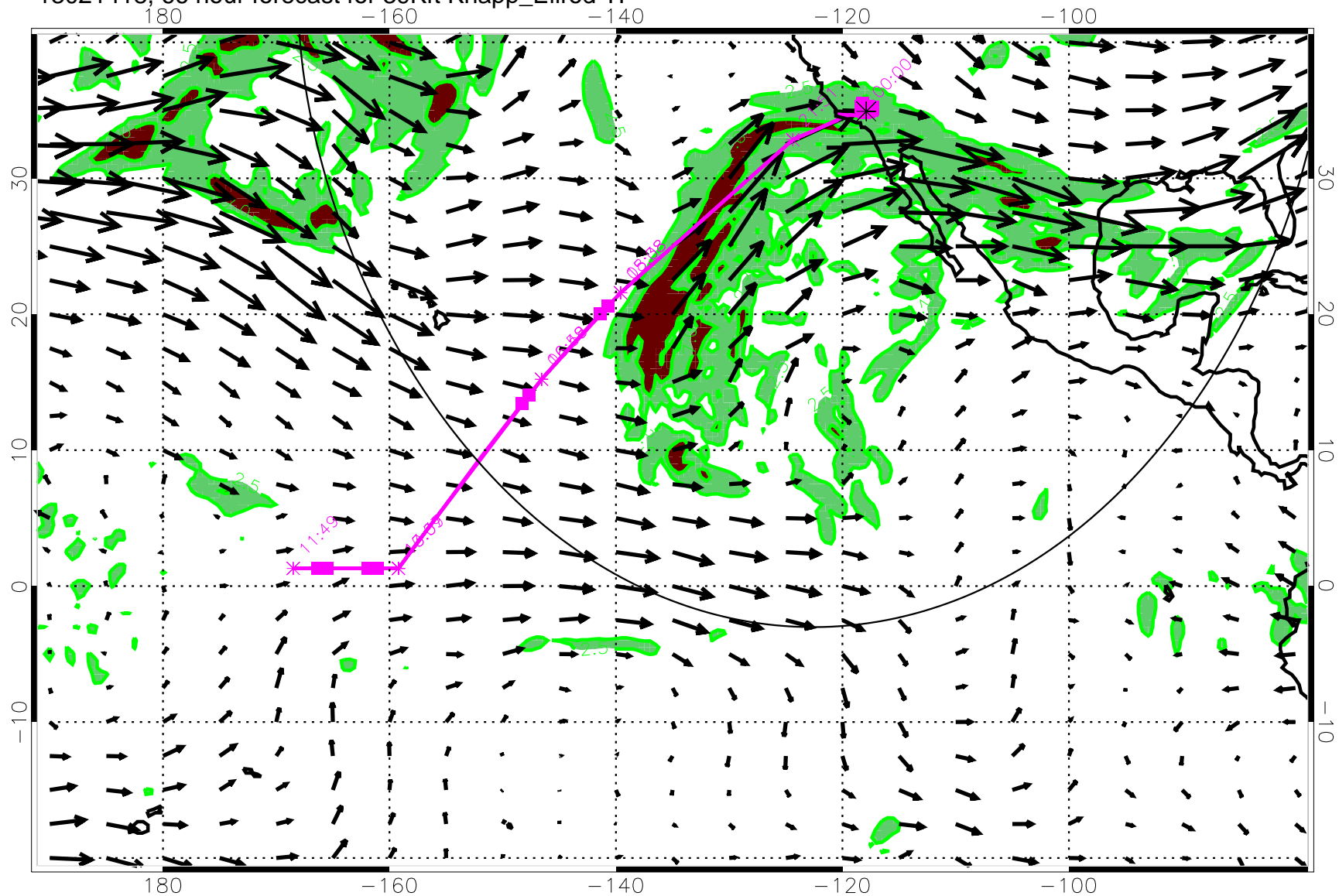
13021418, 66 hour forecast for 39Kft Knapp_Ellrod T1
