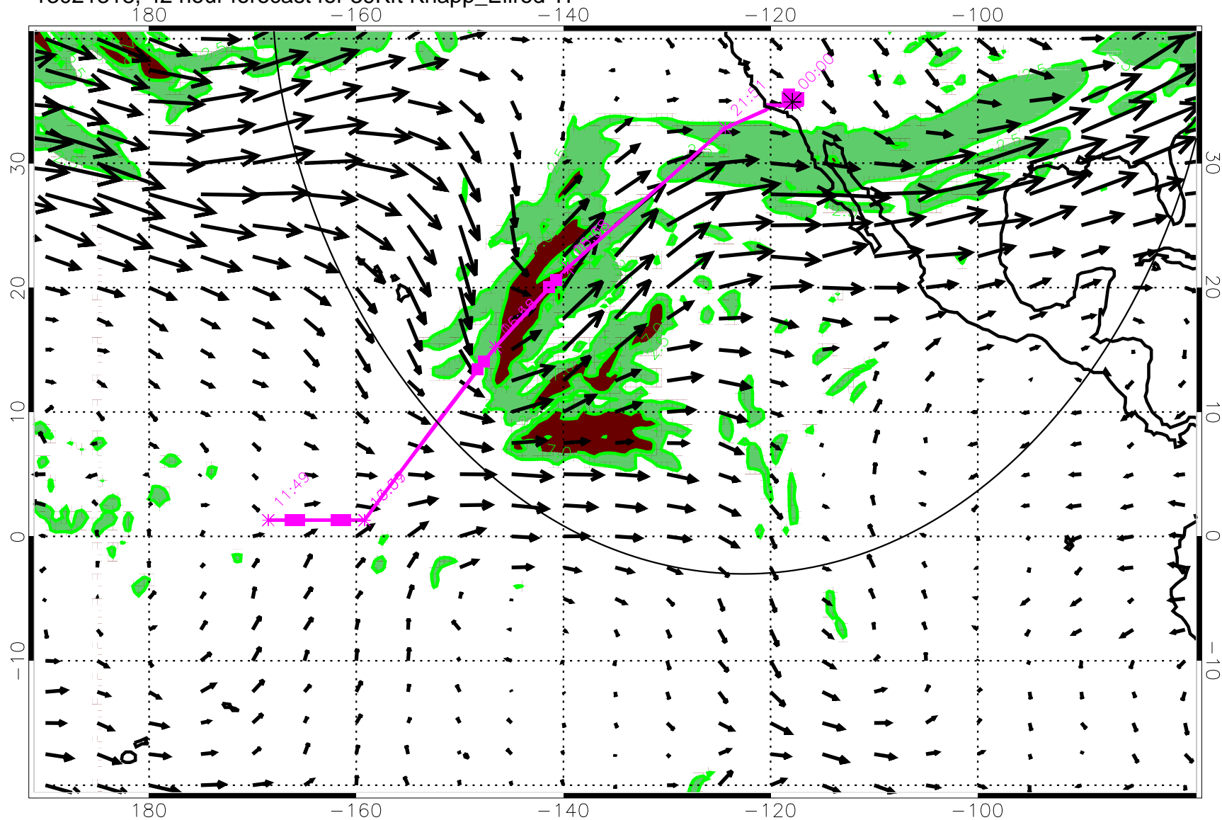
13021318, 42 hour forecast for 39Kft Knapp_Ellrod T1
