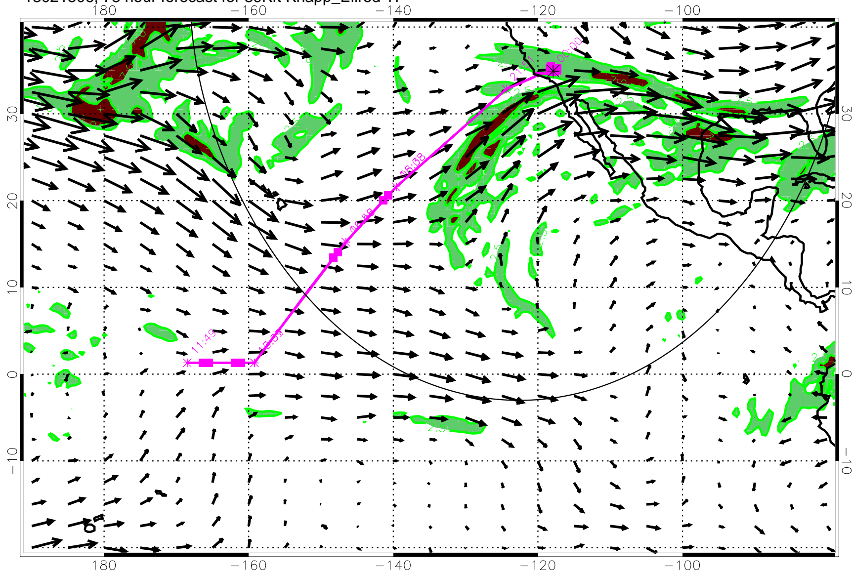
13021506, 78 hour forecast for 39Kft Knapp_Ellrod TI
