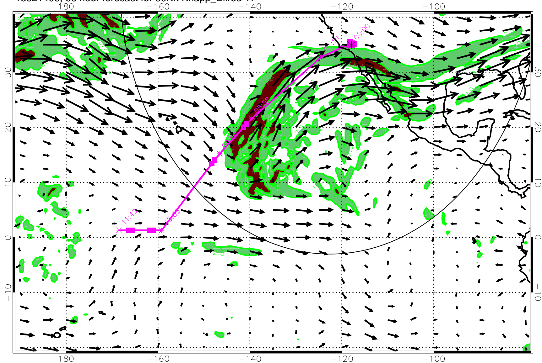
13021406, 66 hour forecast for 39Kft Knapp_Ellrod TI
