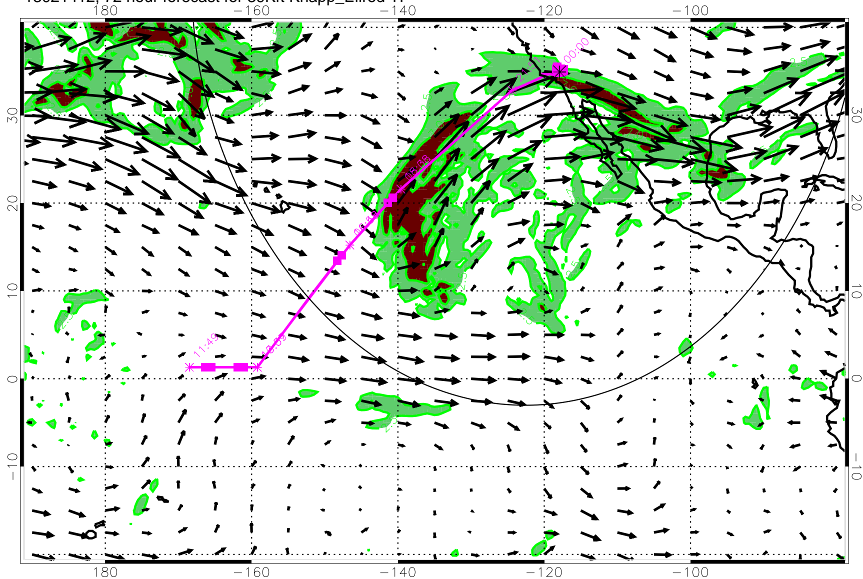
13021412, 72 hour forecast for 39Kft Knapp_Ellrod TI
