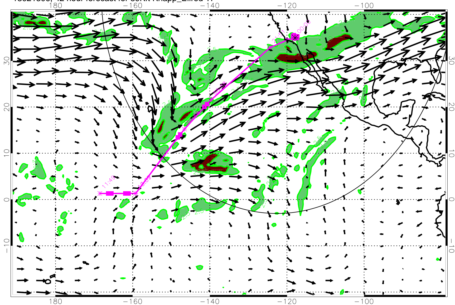
13021306, 42 hour forecast for 39Kft Knapp_Ellrod TI
