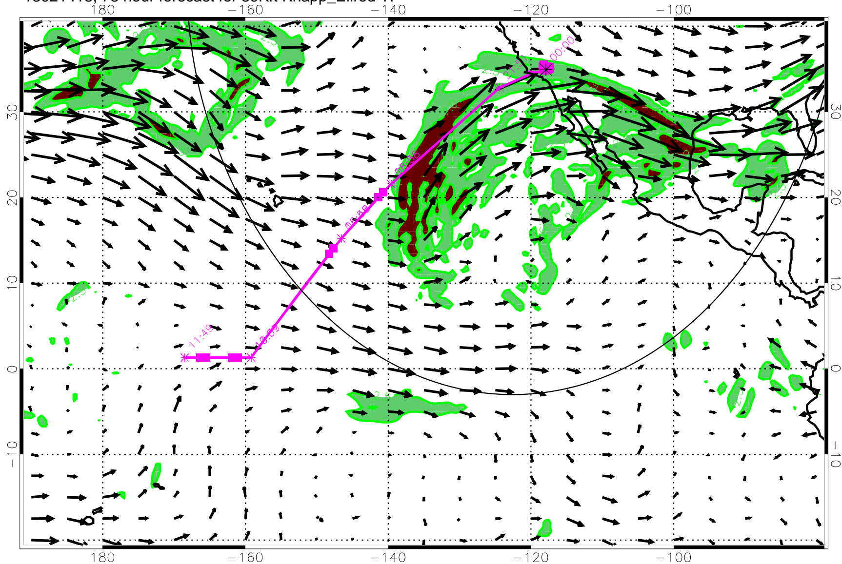
13021418, 78 hour forecast for 39Kft Knapp_Ellrod T1
