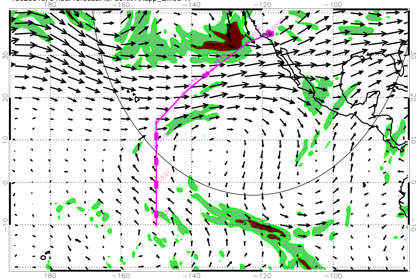
13020818, 6 hour forecast for 39Kft Knapp_Ellrod TI
