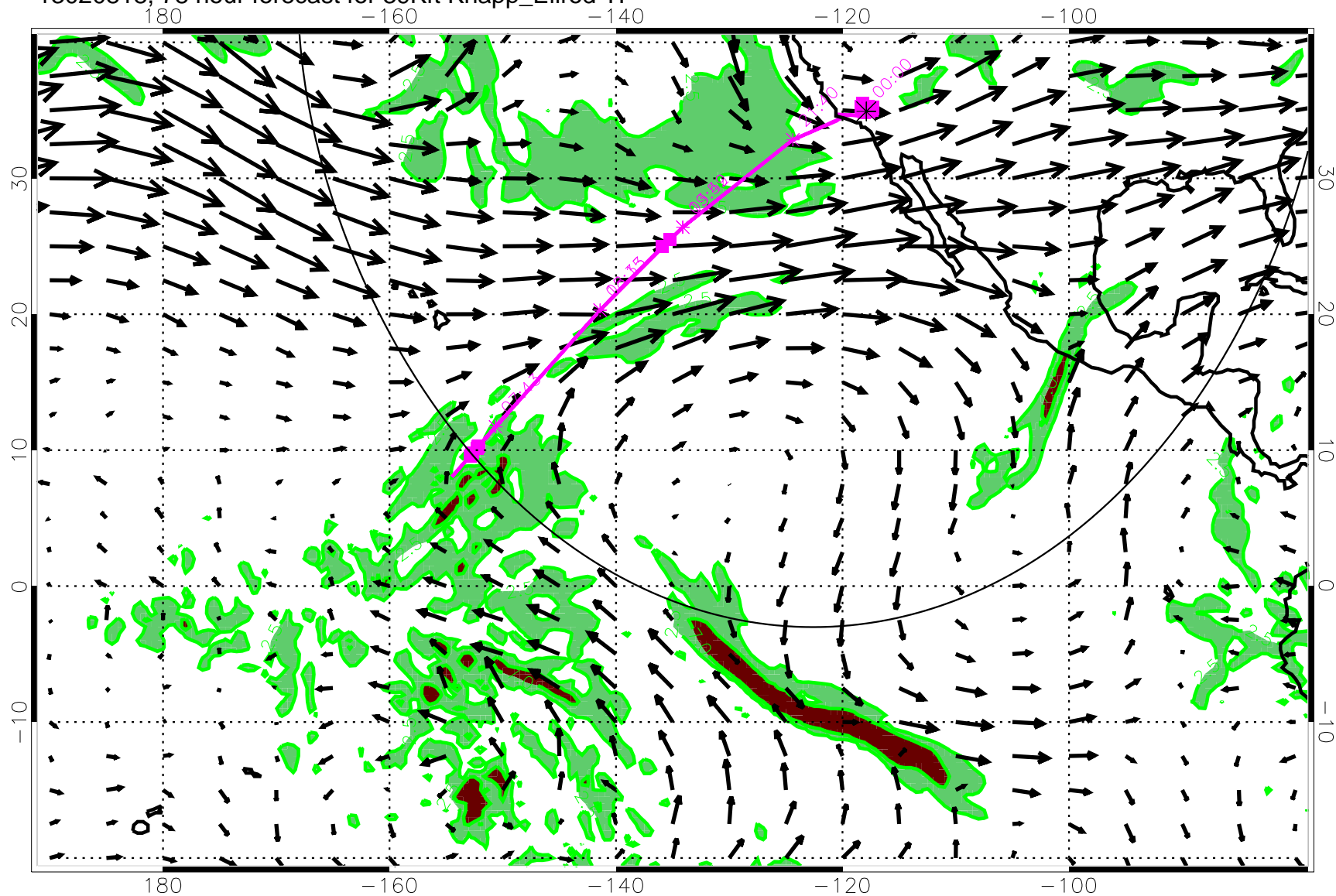
13020818, 78 hour forecast for 39Kft Knapp_Ellrod TI
