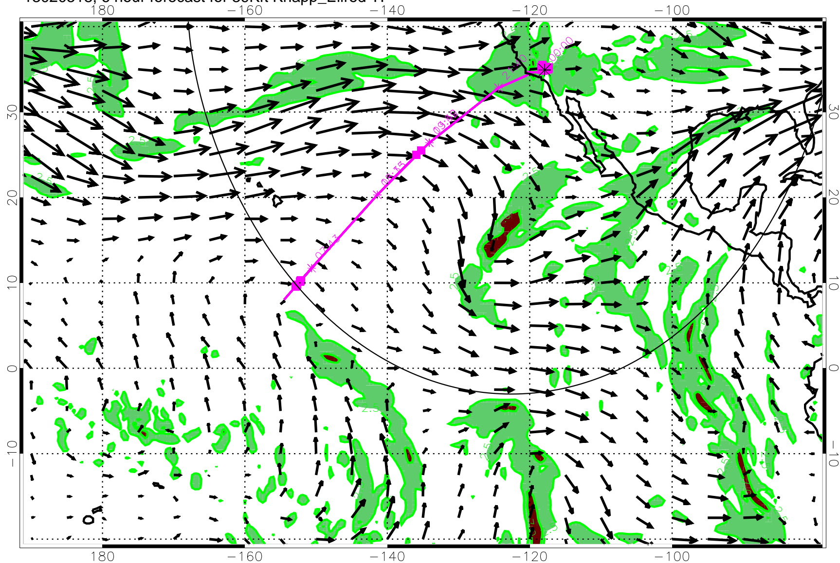
13020518, 6 hour forecast for 39Kft Knapp_Ellrod TI
