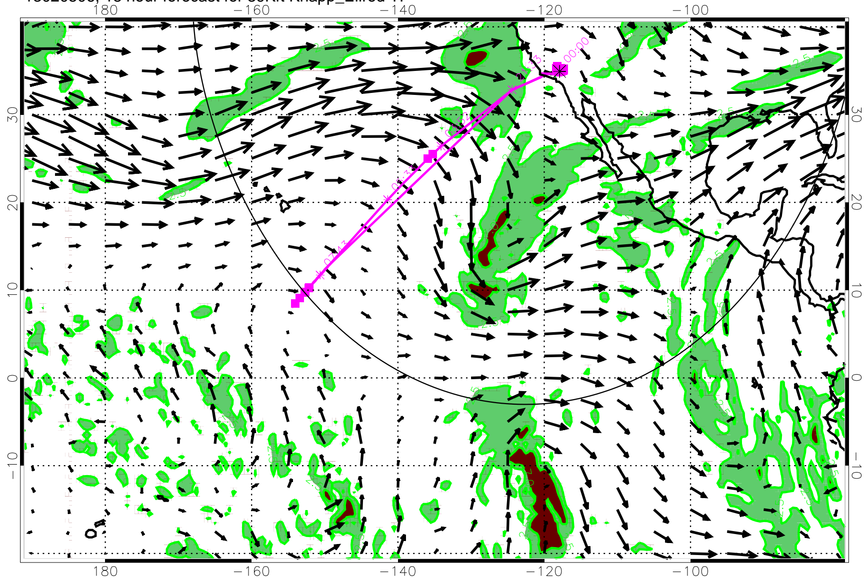
13020506, 18 hour forecast for 39Kft Knapp_Ellrod TI
