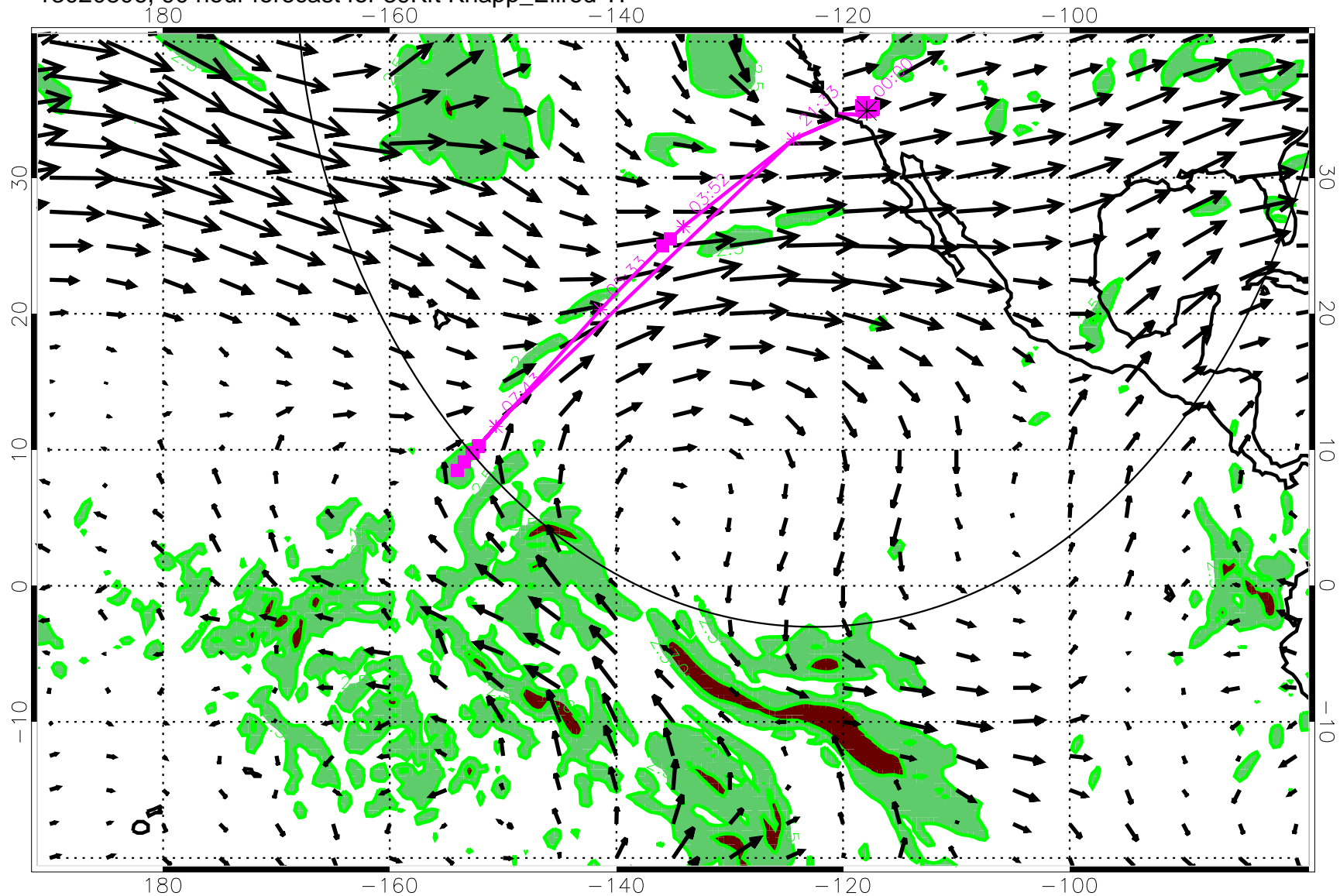
13020806, 90 hour forecast for 39Kft Knapp_Ellrod TI
