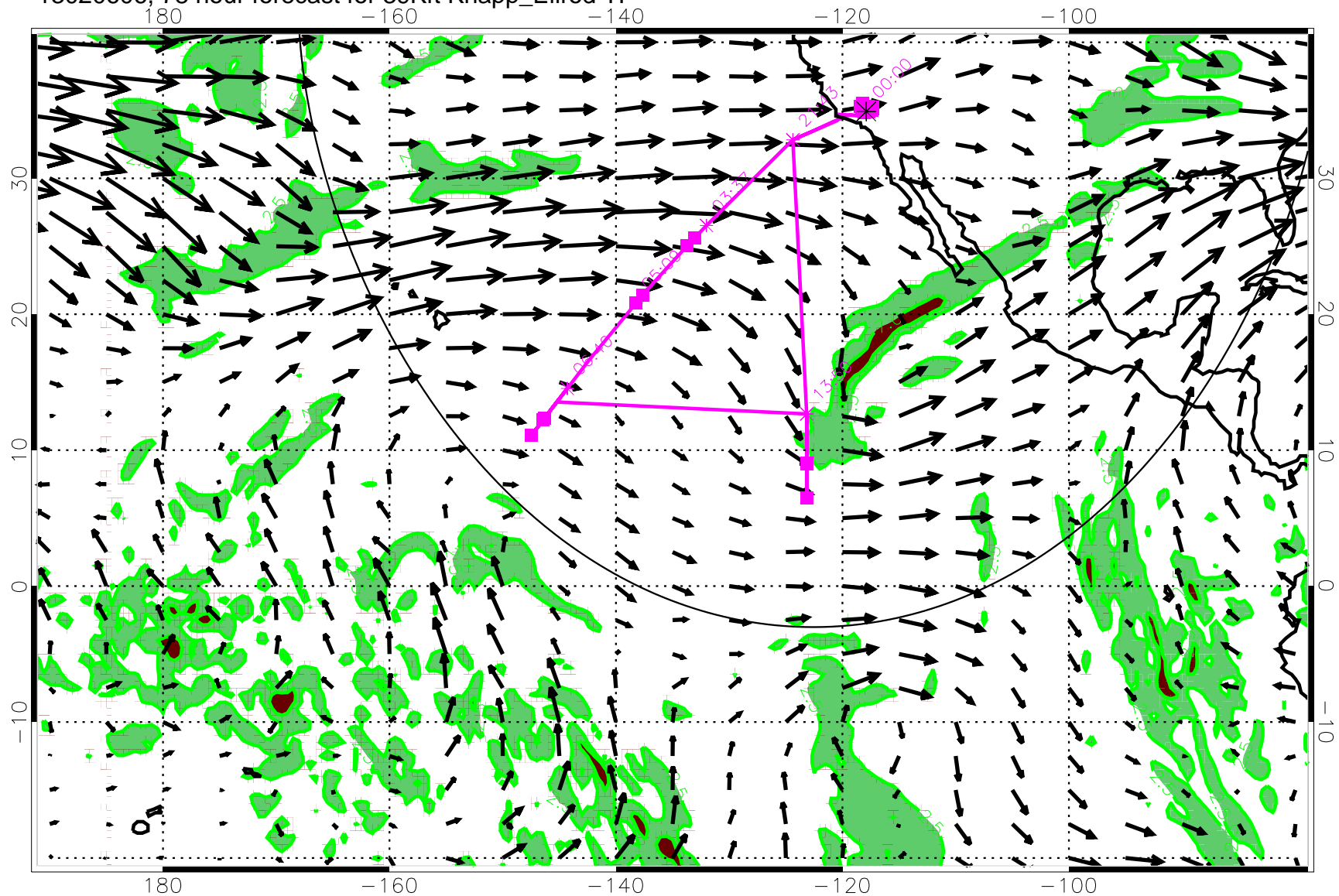
13020606, 78 hour forecast for 39Kft Knapp_Ellrod TI
