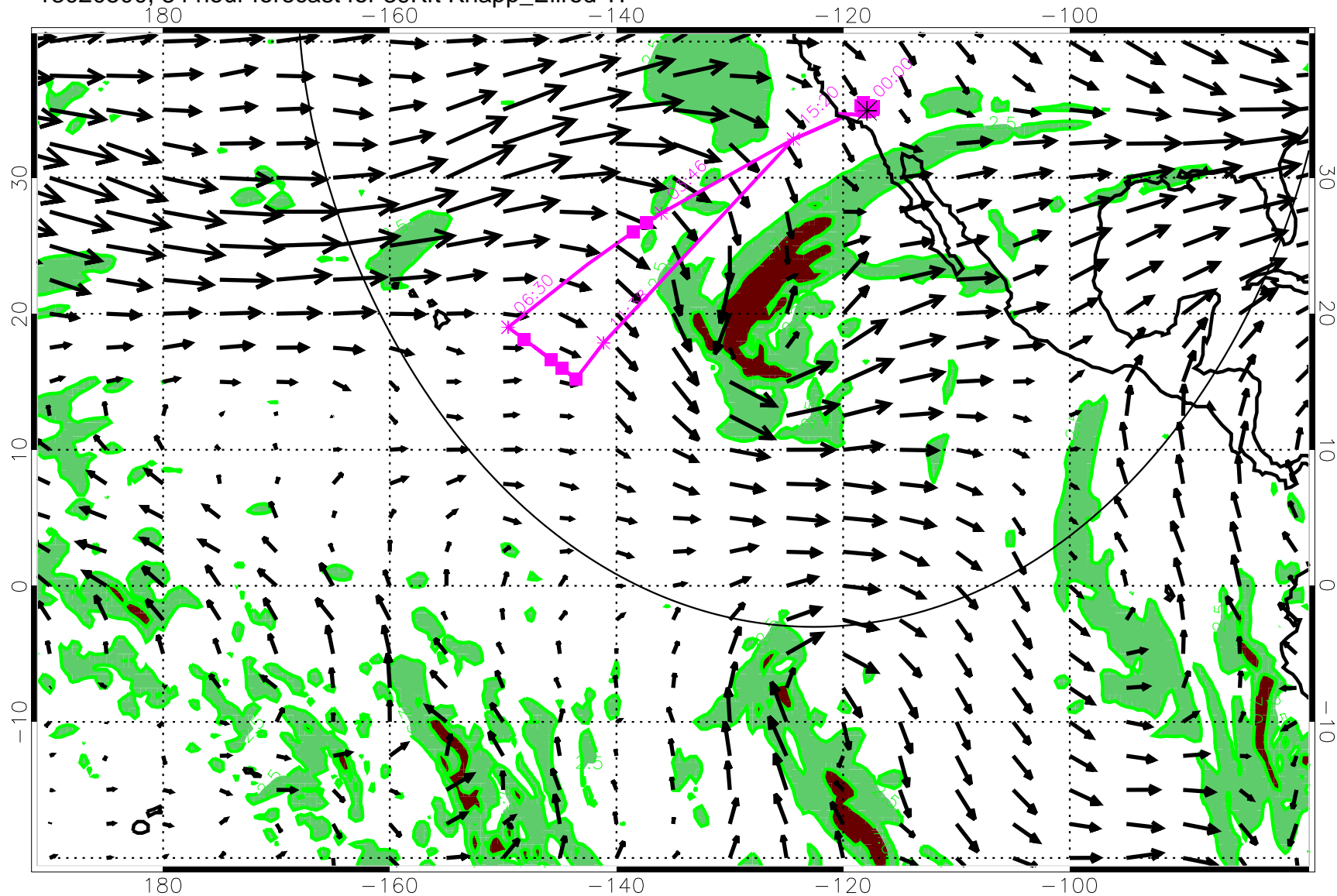
13020500, 84 hour forecast for 39Kft Knapp_Ellrod TI
