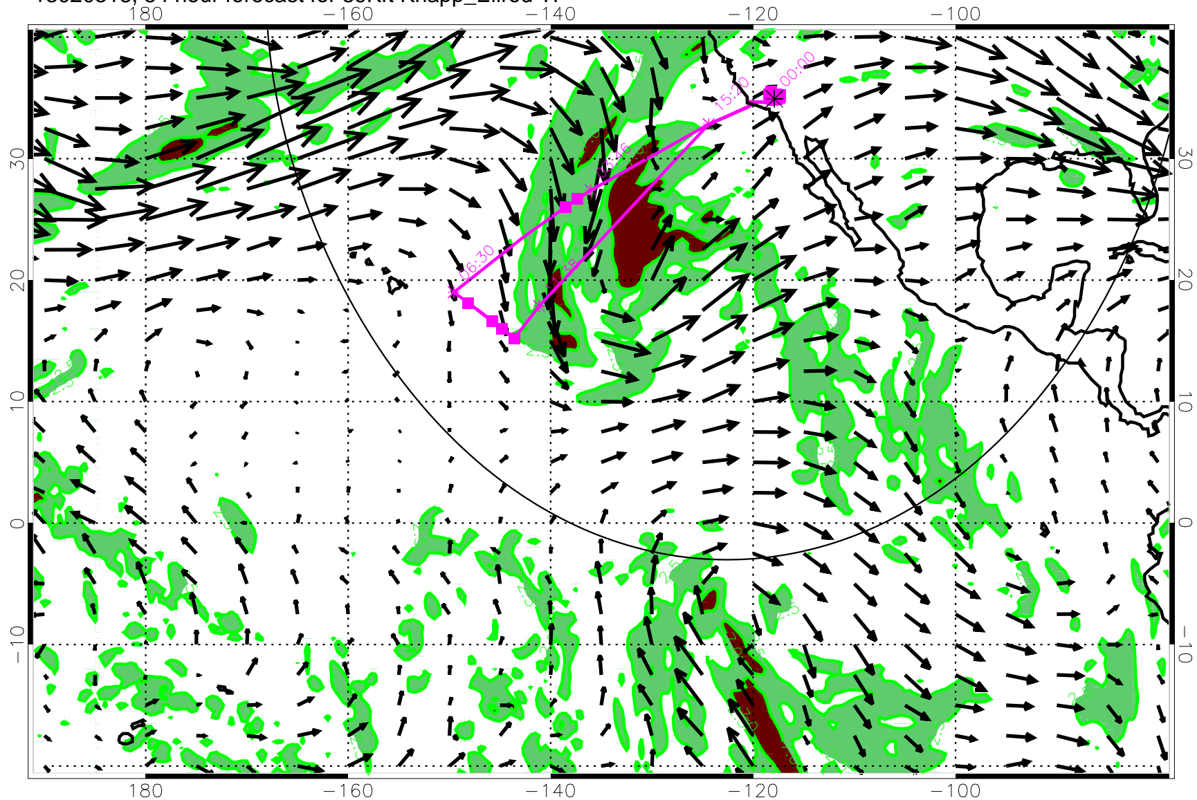
13020318, 54 hour forecast for 39Kft Knapp_Ellrod TI
