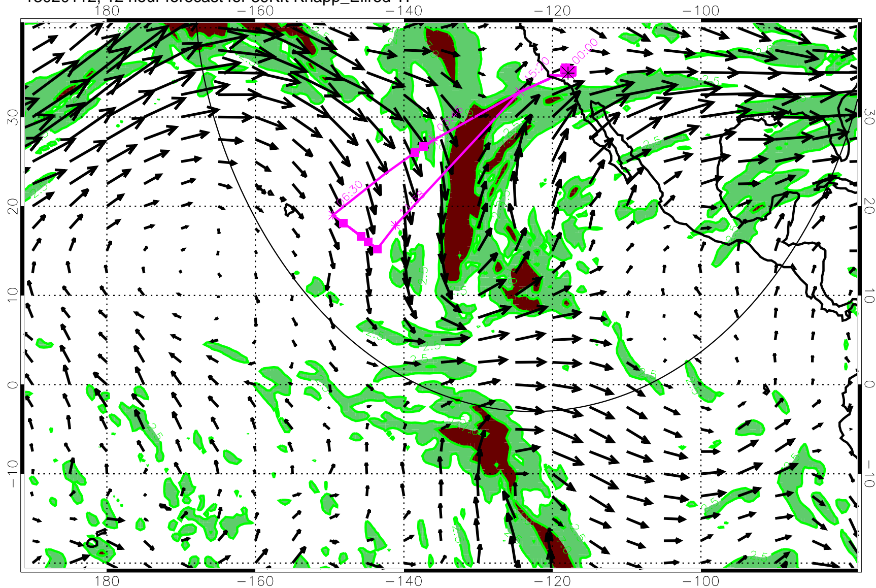
13020112, 12 hour forecast for 39Kft Knapp_Ellrod TI
