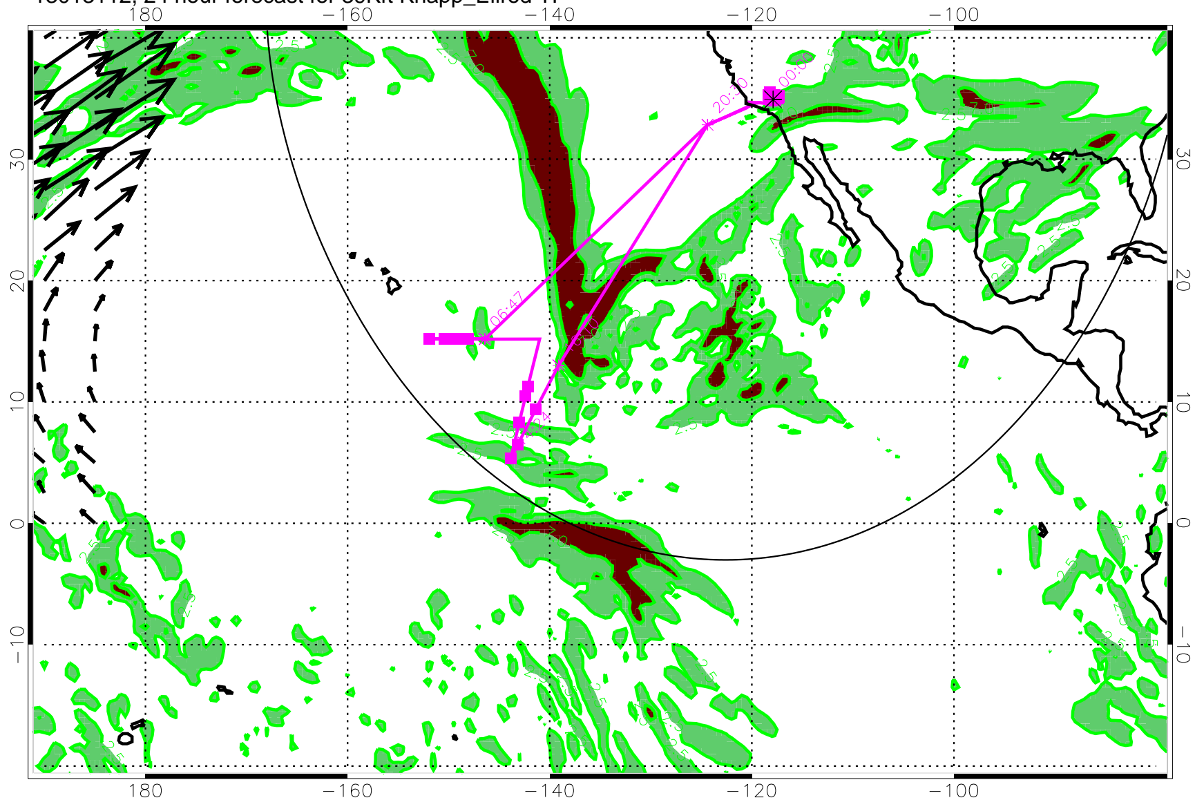
13013112, 24 hour forecast for 39Kft Knapp_Ellrod TI
