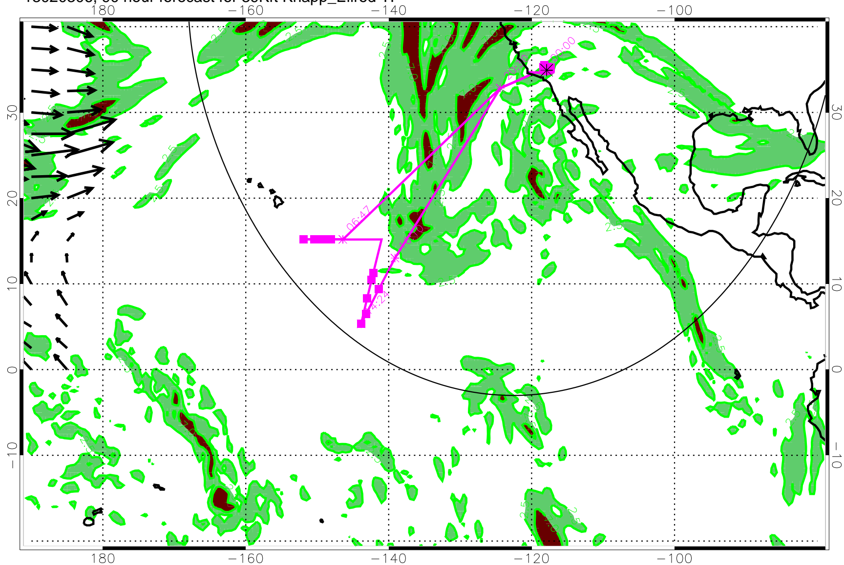
13020306, 90 hour forecast for 39Kft Knapp_Ellrod TI
