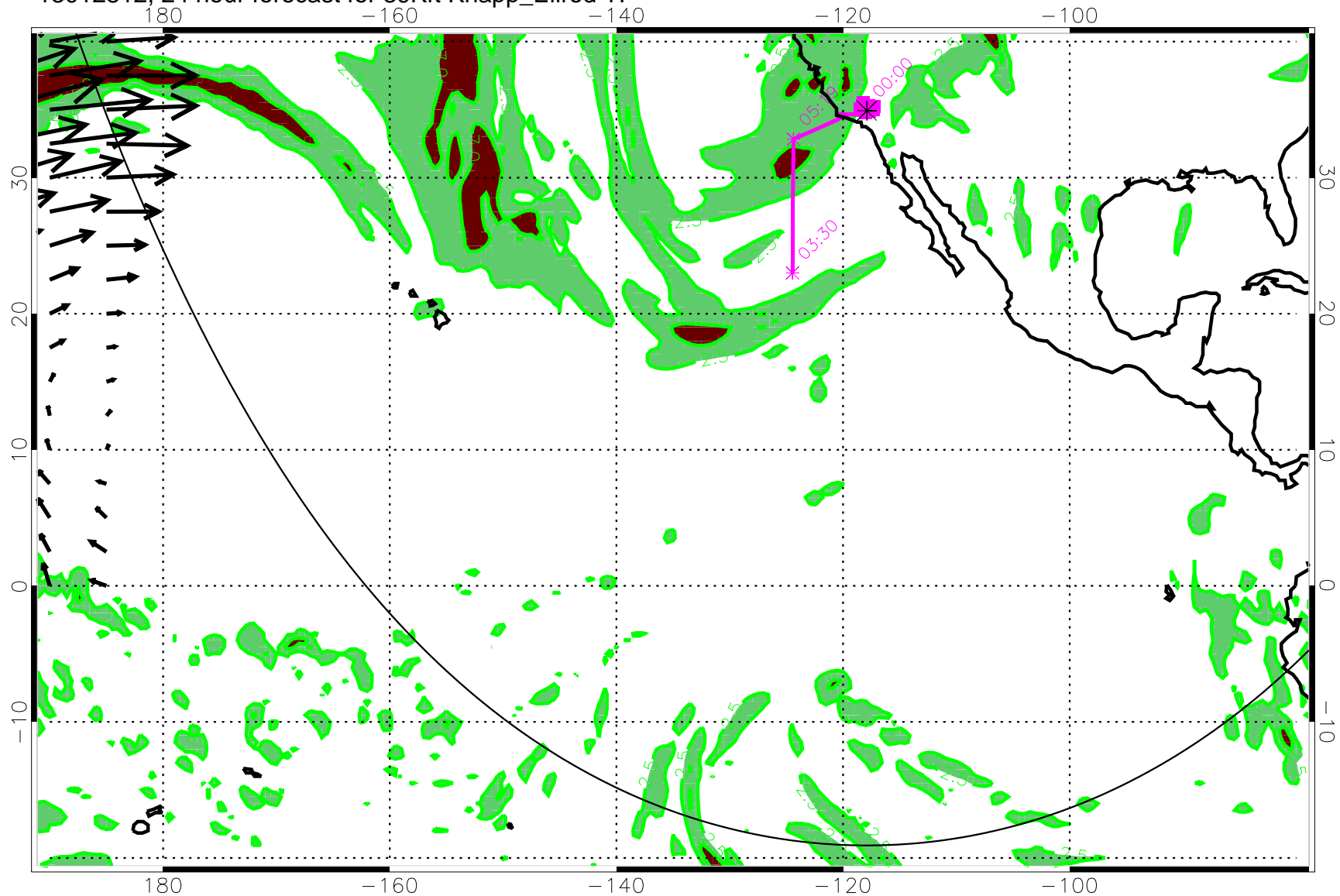
13012812, 24 hour forecast for 39Kft Knapp_Ellrod TI
