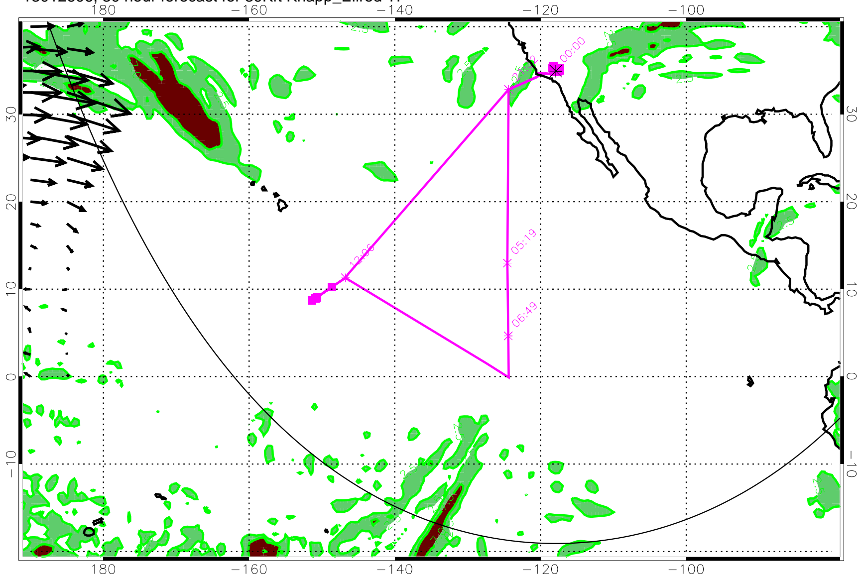
13012606, 30 hour forecast for 39Kft Knapp_Ellrod TI
