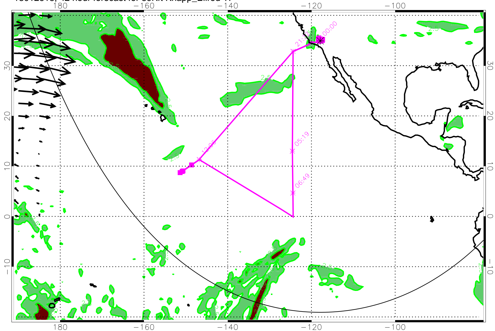
13012618, 42 hour forecast for 39Kft Knapp_Ellrod TI
