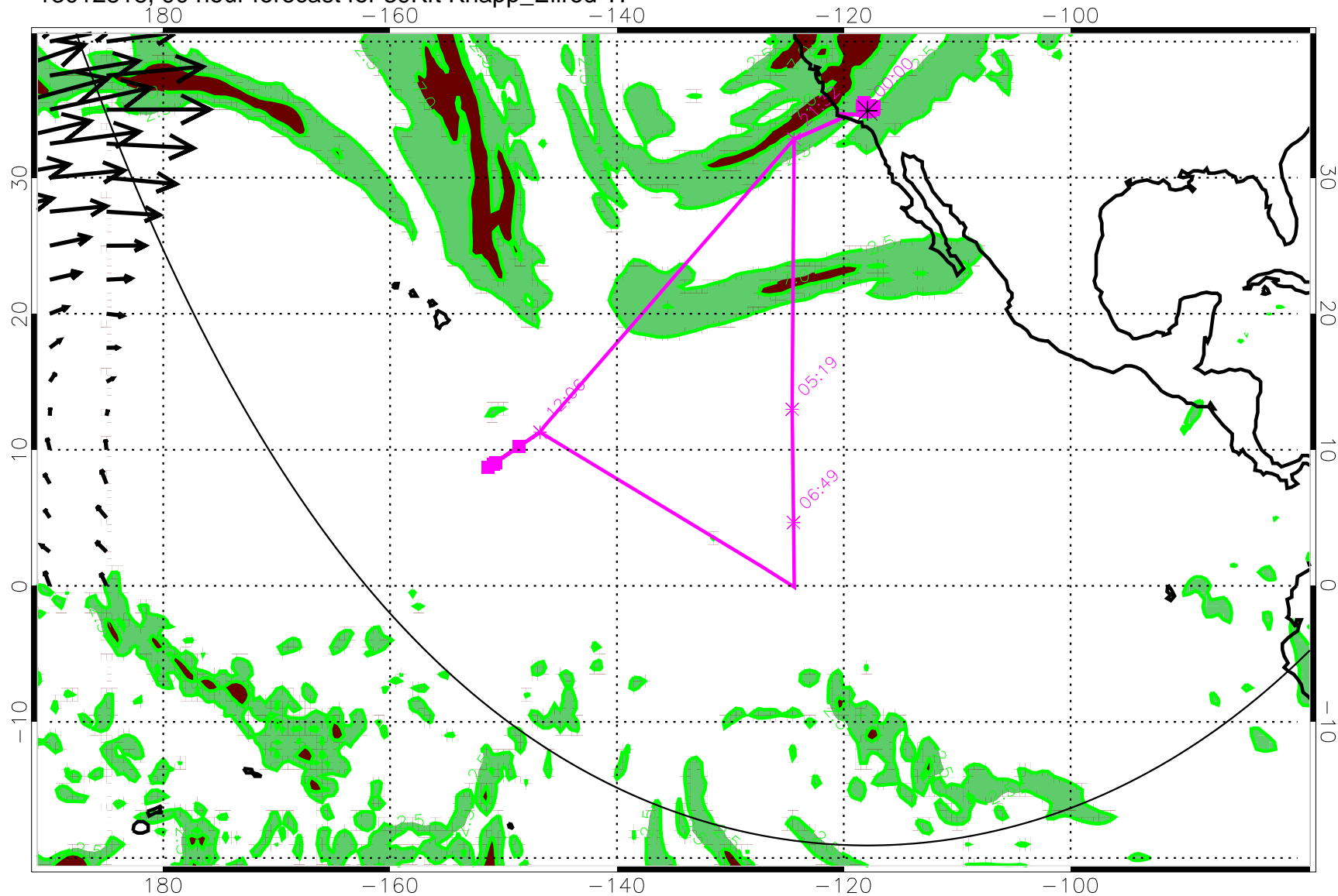
13012818, 90 hour forecast for 39Kft Knapp_Ellrod TI
