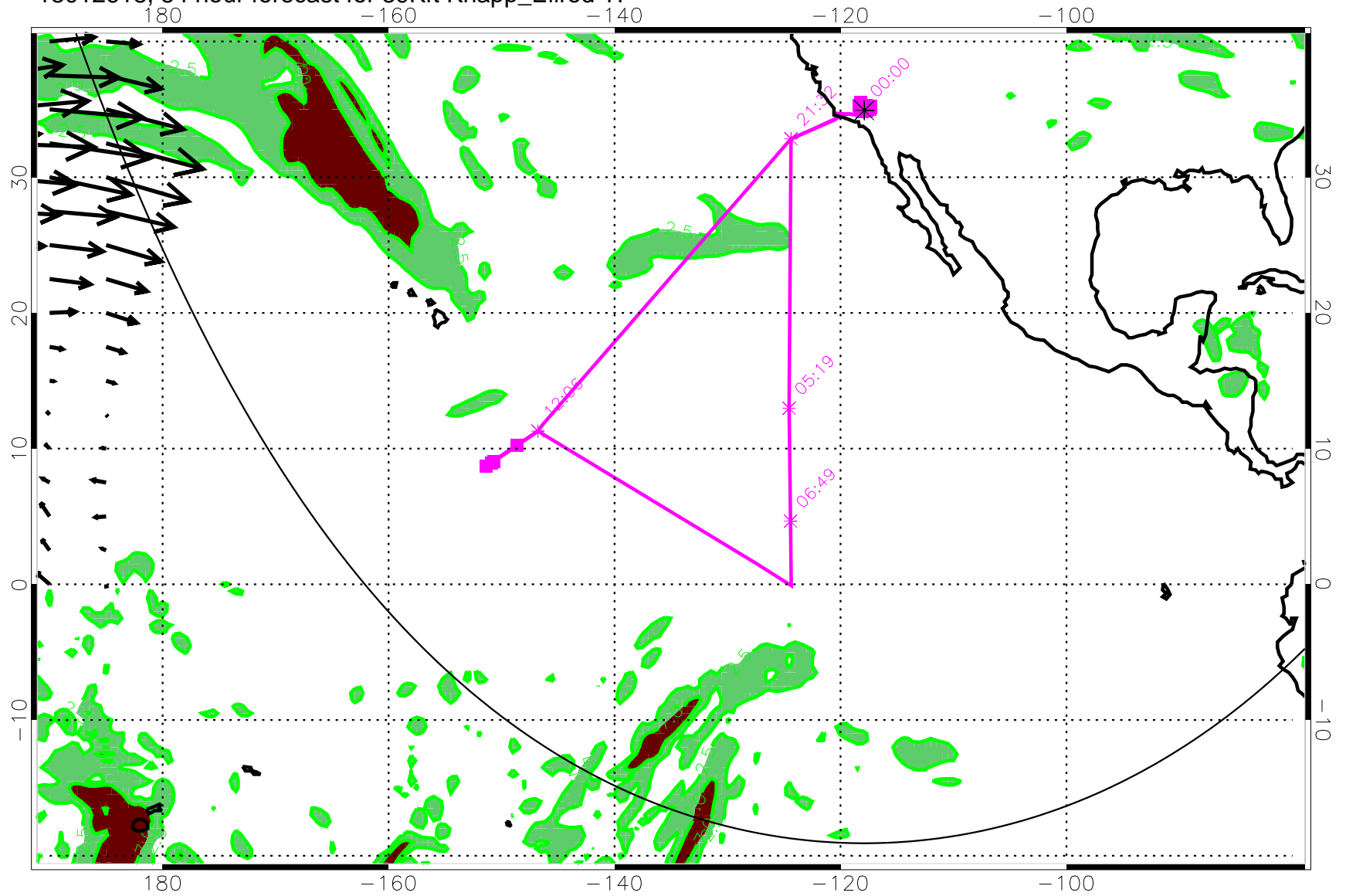
13012618, 54 hour forecast for 39Kft Knapp_Ellrod TI
