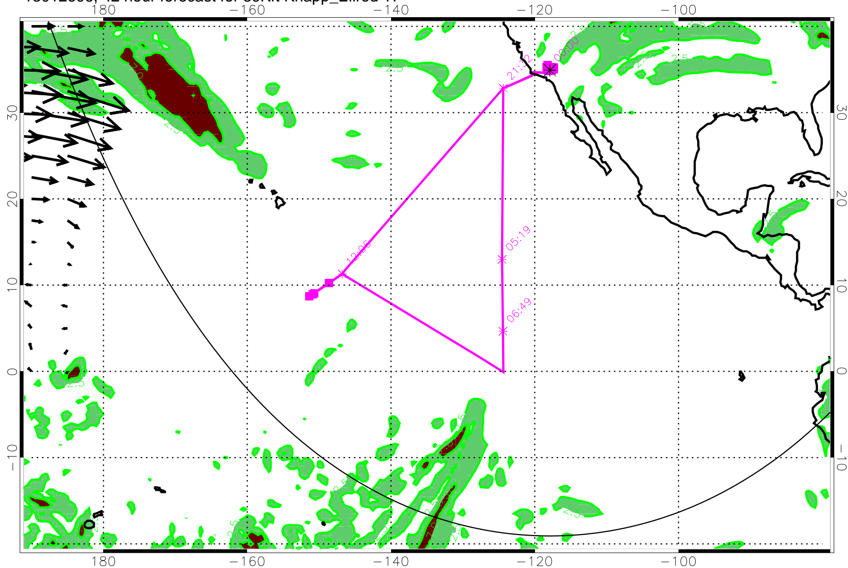
13012606, 42 hour forecast for 39Kft Knapp_Ellrod TI
