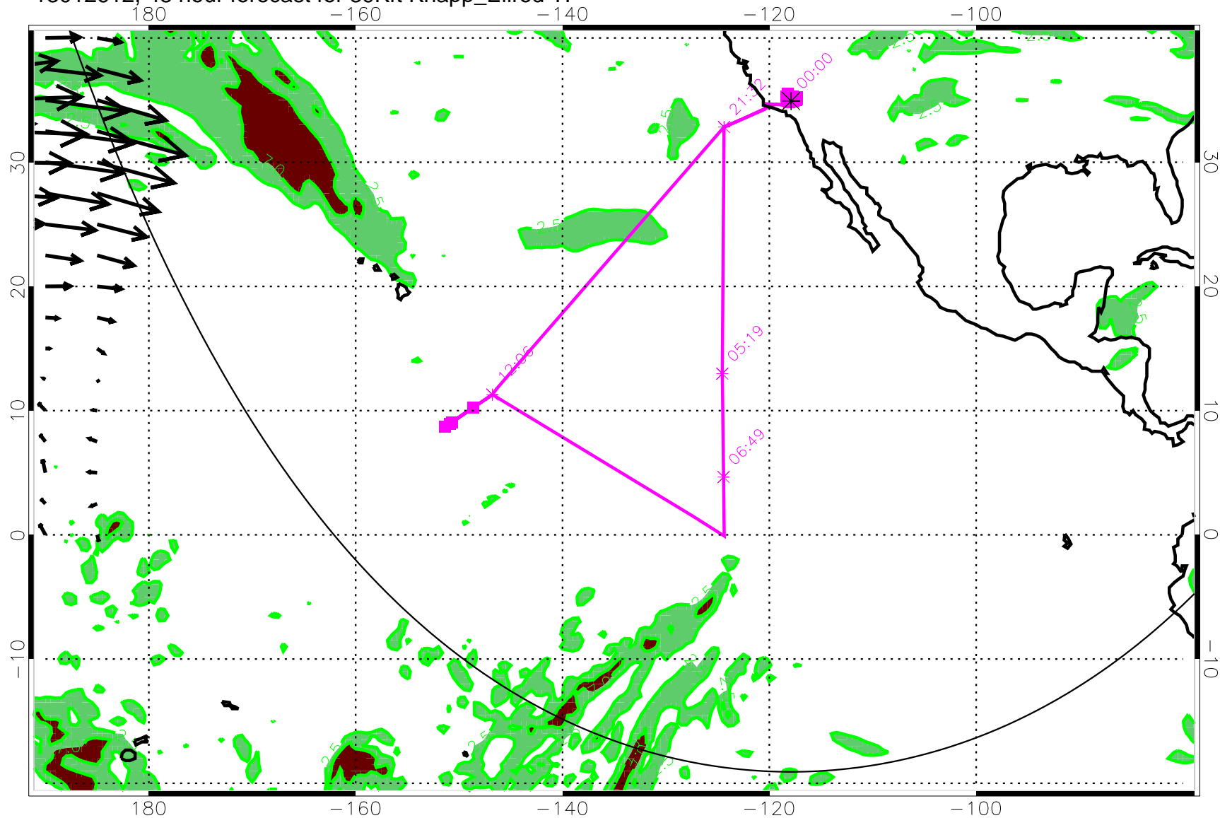
13012612, 48 hour forecast for 39Kft Knapp_Ellrod TI
