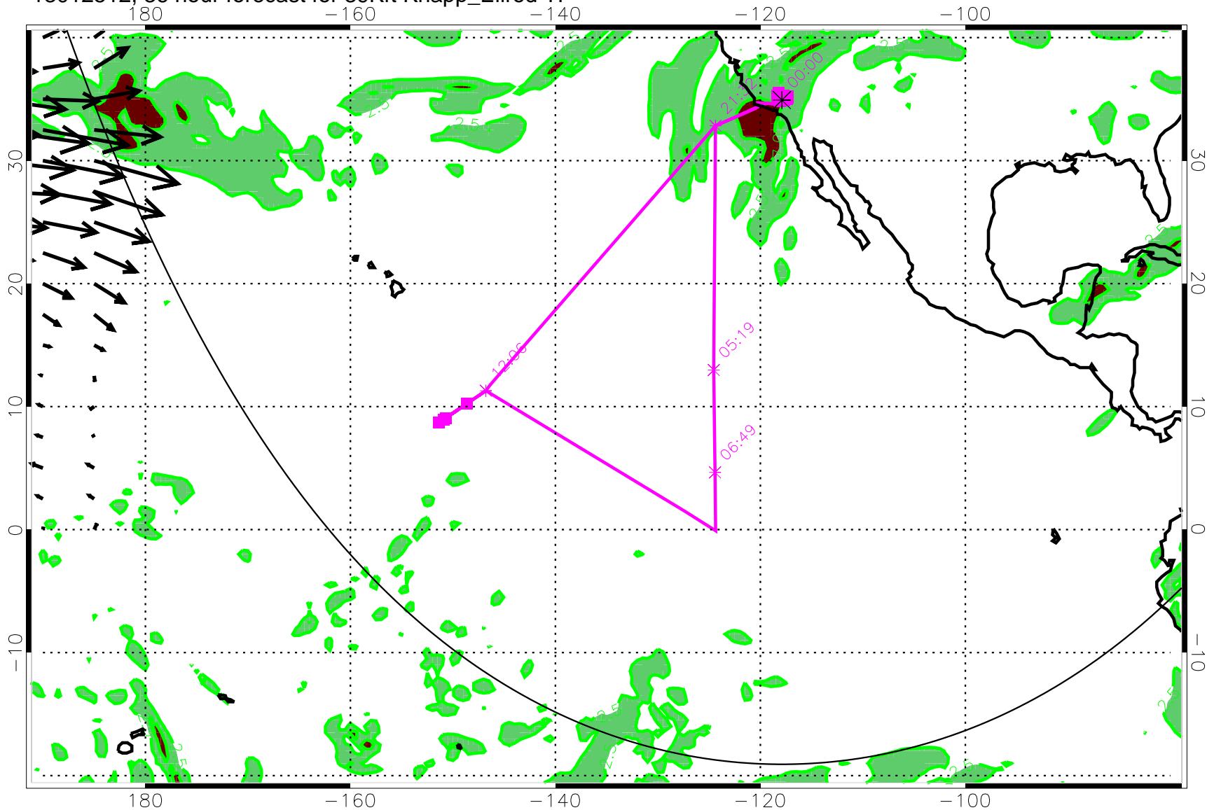
13012512, 36 hour forecast for 39Kft Knapp_Ellrod TI
