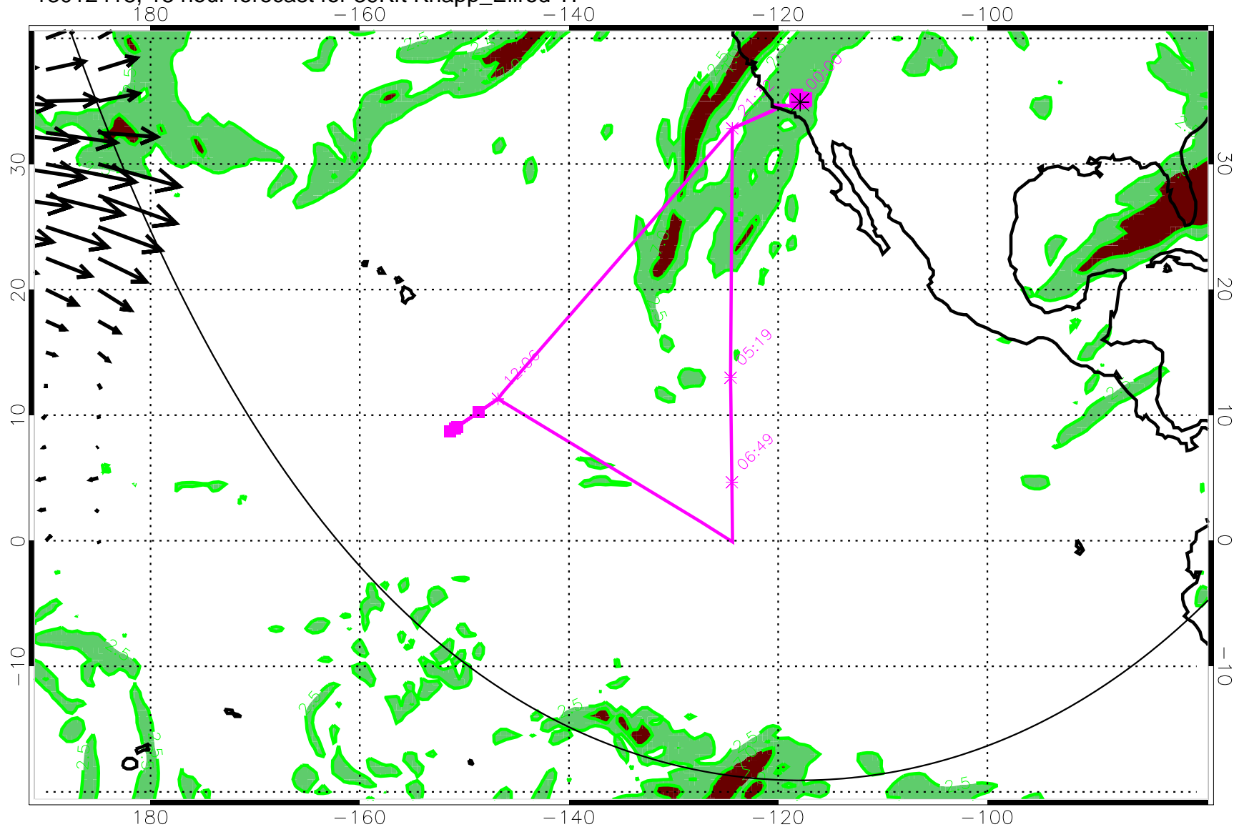
13012418, 18 hour forecast for 39Kft Knapp_Ellrod TI
