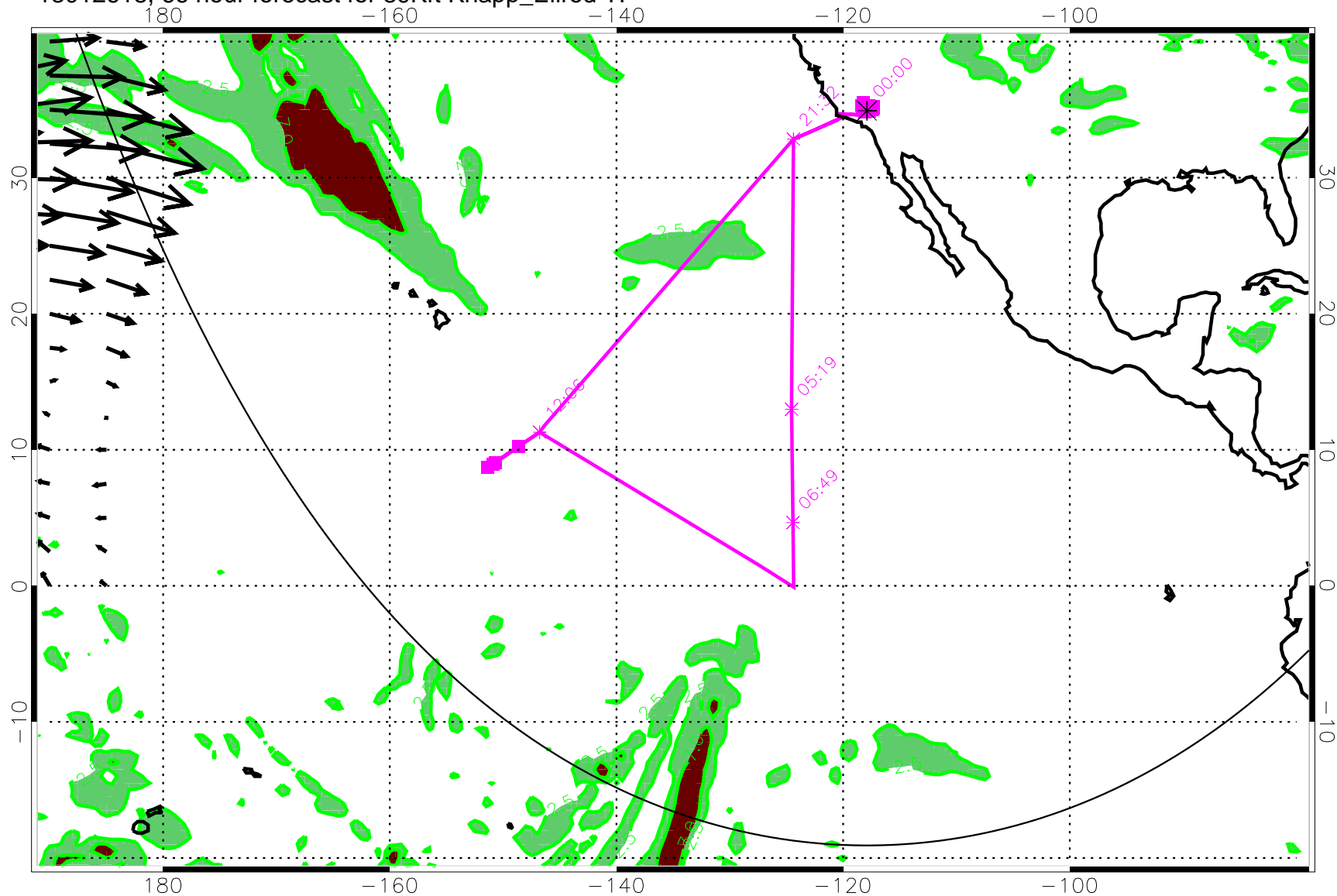
13012618, 66 hour forecast for 39Kft Knapp_Ellrod TI
