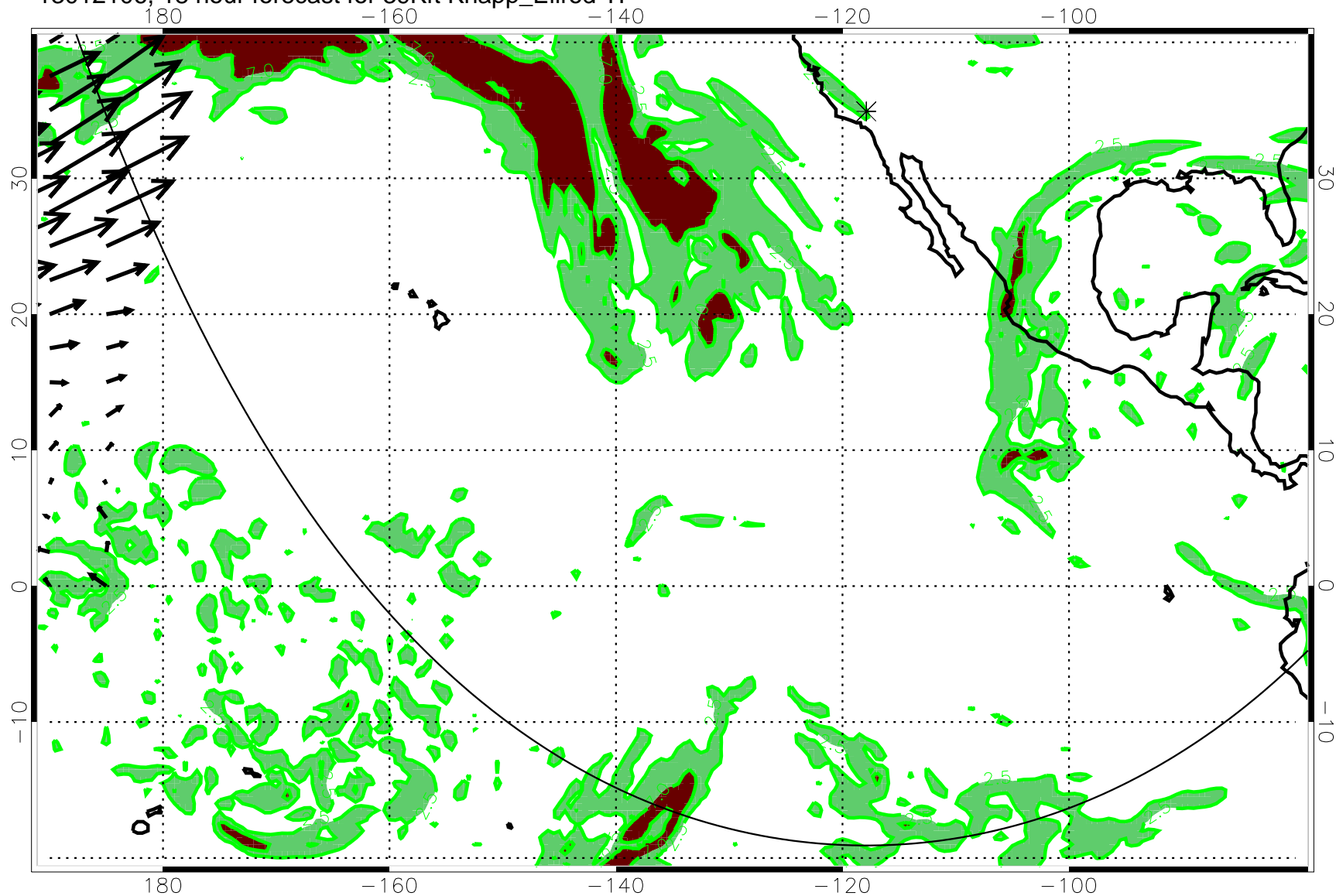
13012106, 18 hour forecast for 39Kft Knapp_Ellrod TI
