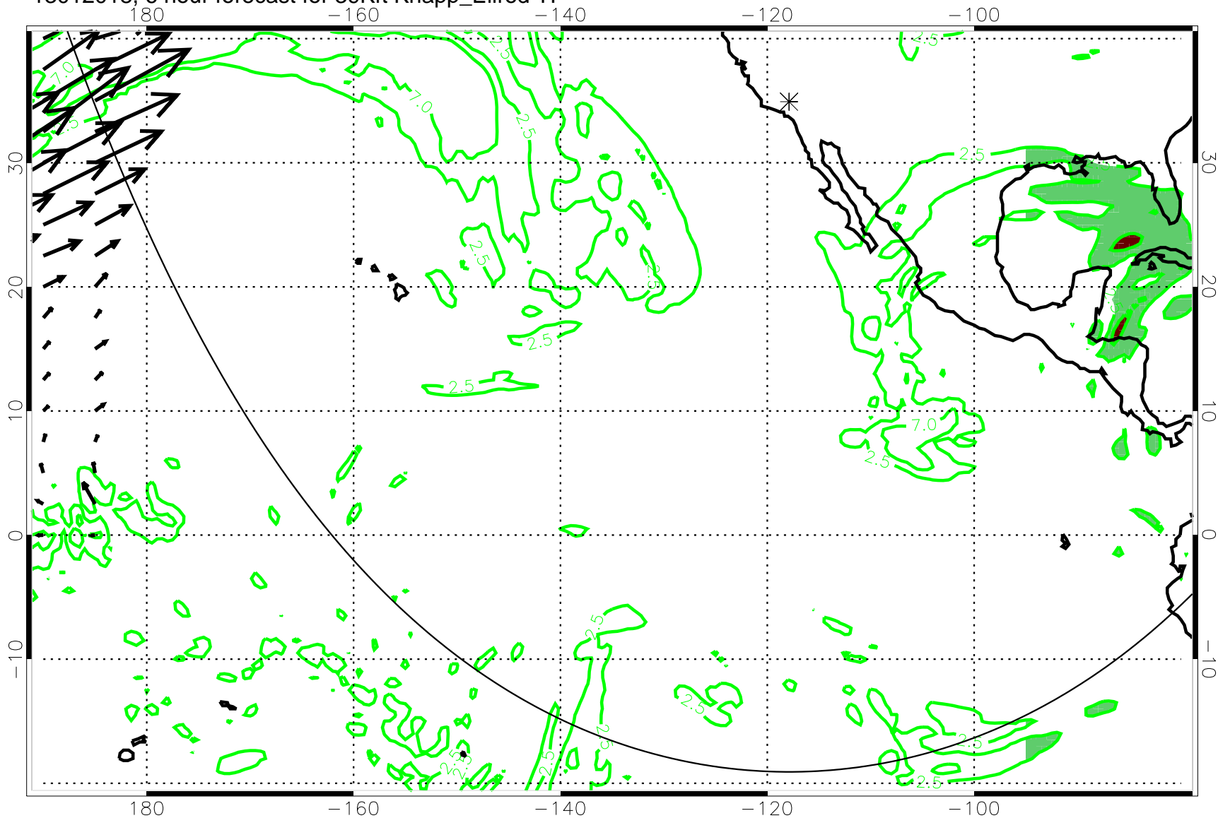
13012018, 6 hour forecast for 39Kft Knapp_Ellrod TI
