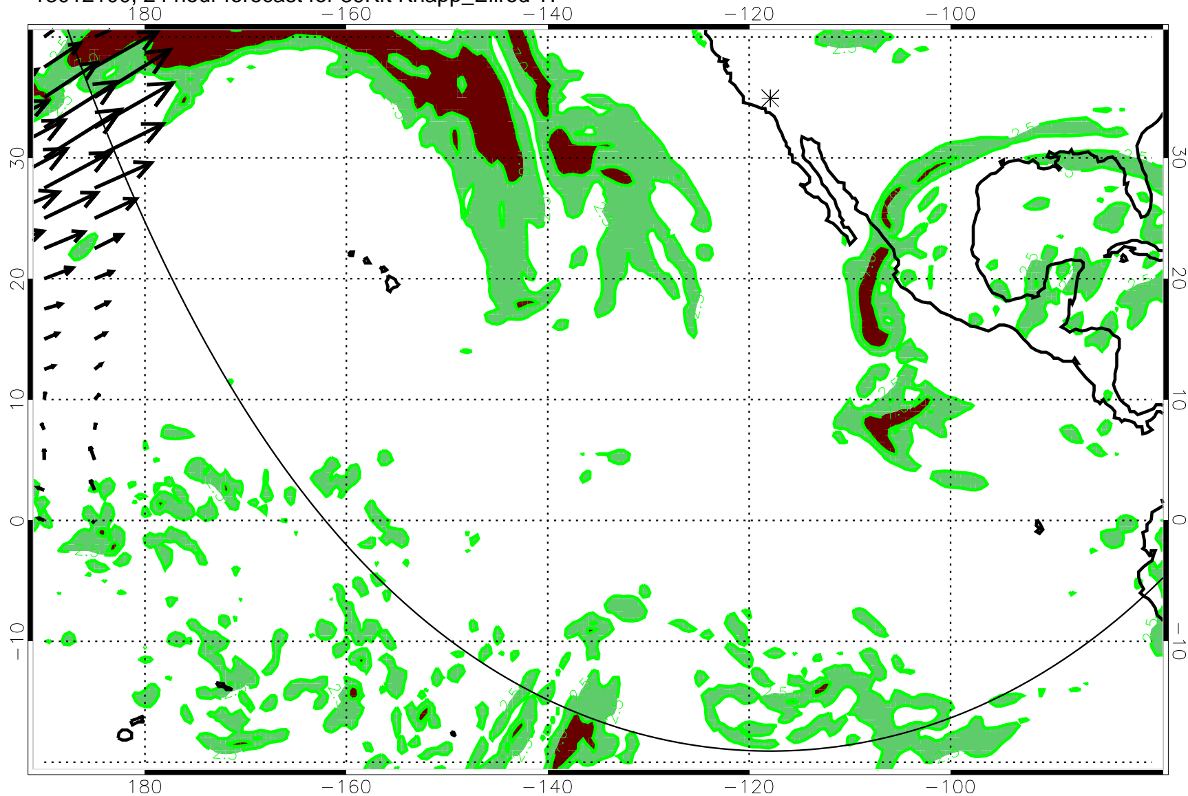
13012100, 24 hour forecast for 39Kft Knapp_Ellrod TI
