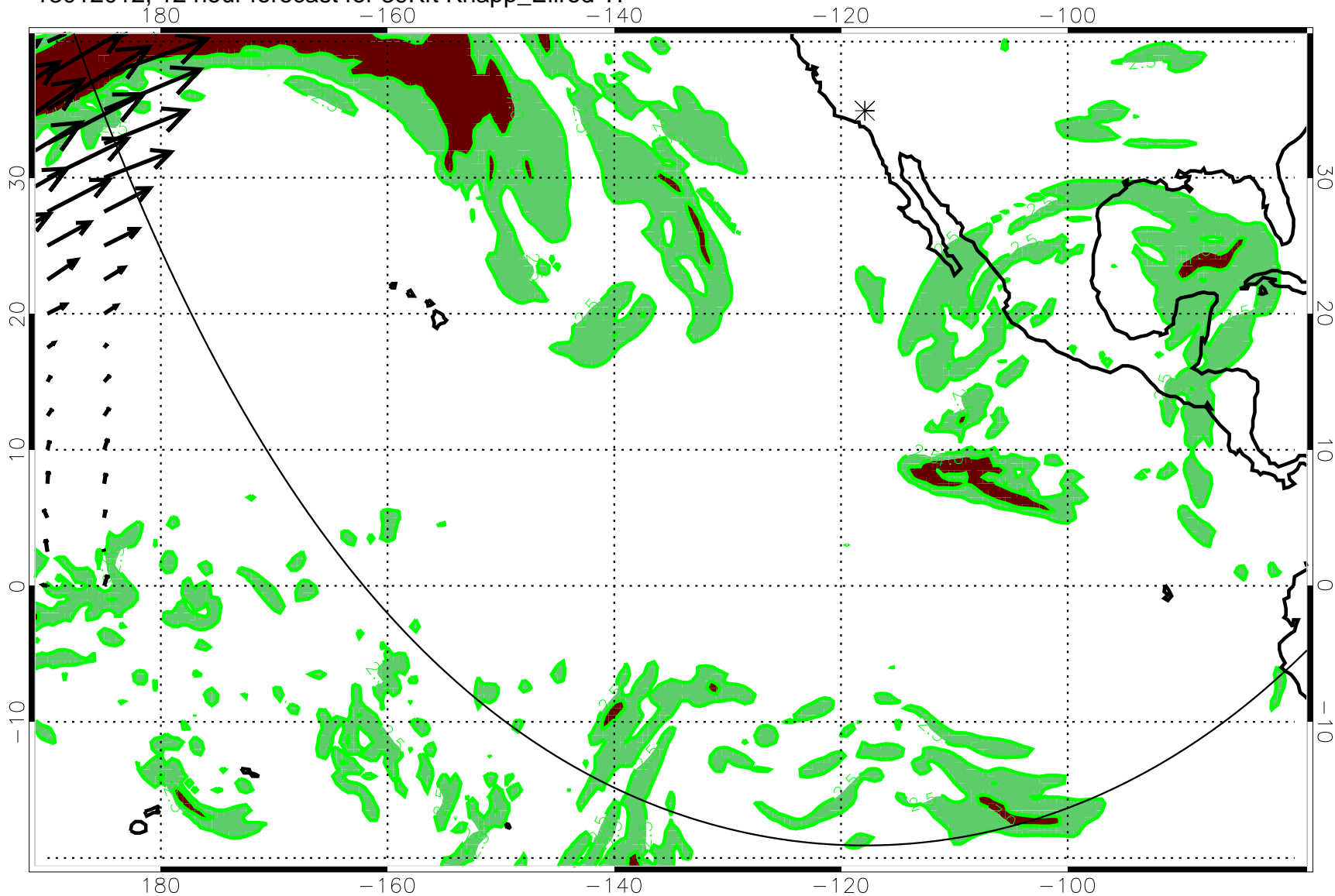
13012012, 12 hour forecast for 39Kft Knapp_Ellrod TI
