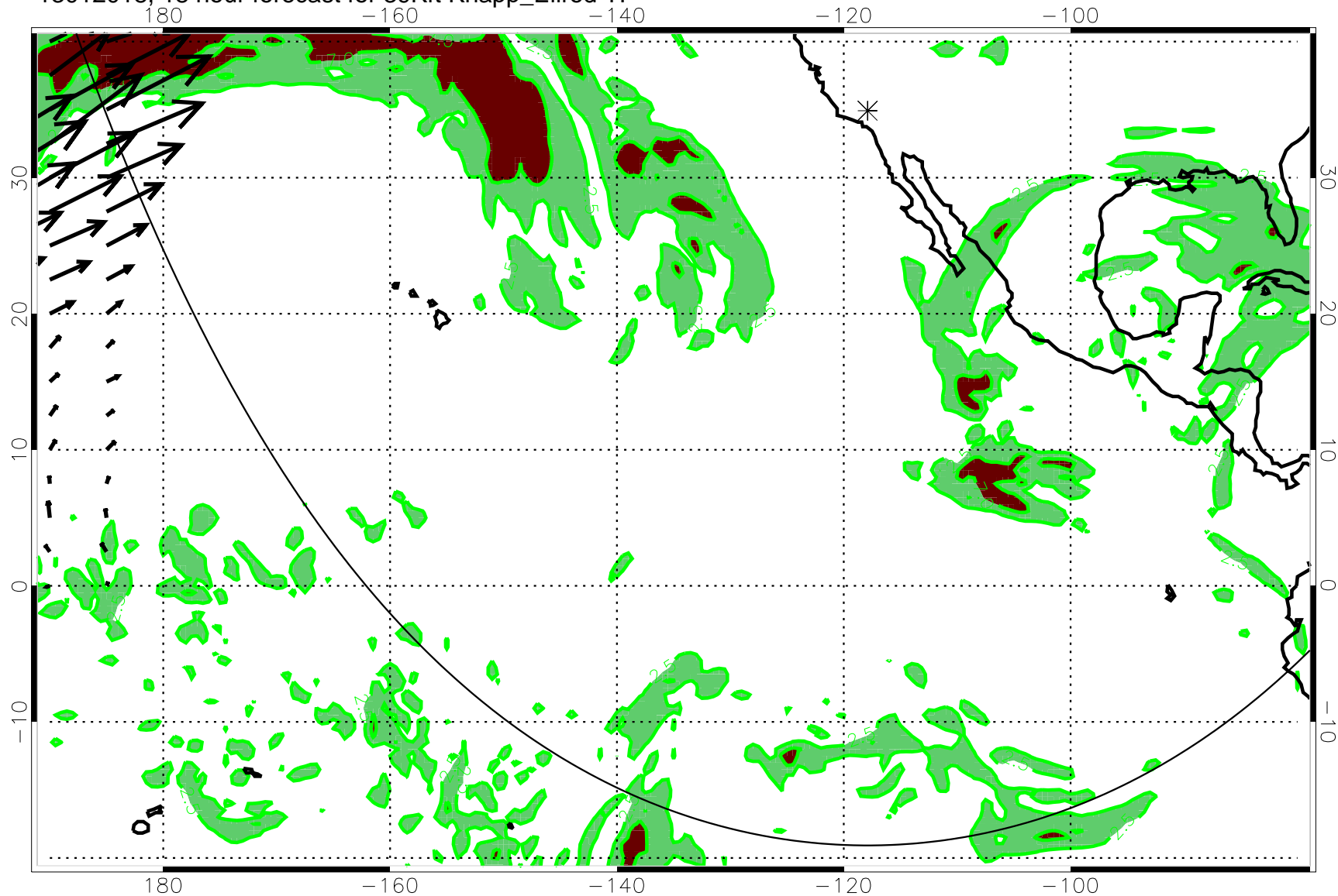
13012018, 18 hour forecast for 39Kft Knapp_Ellrod TI
