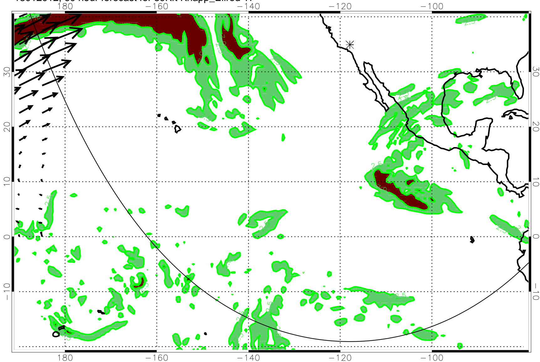
13012012, 60 hour forecast for 39Kft Knapp_Ellrod TI
