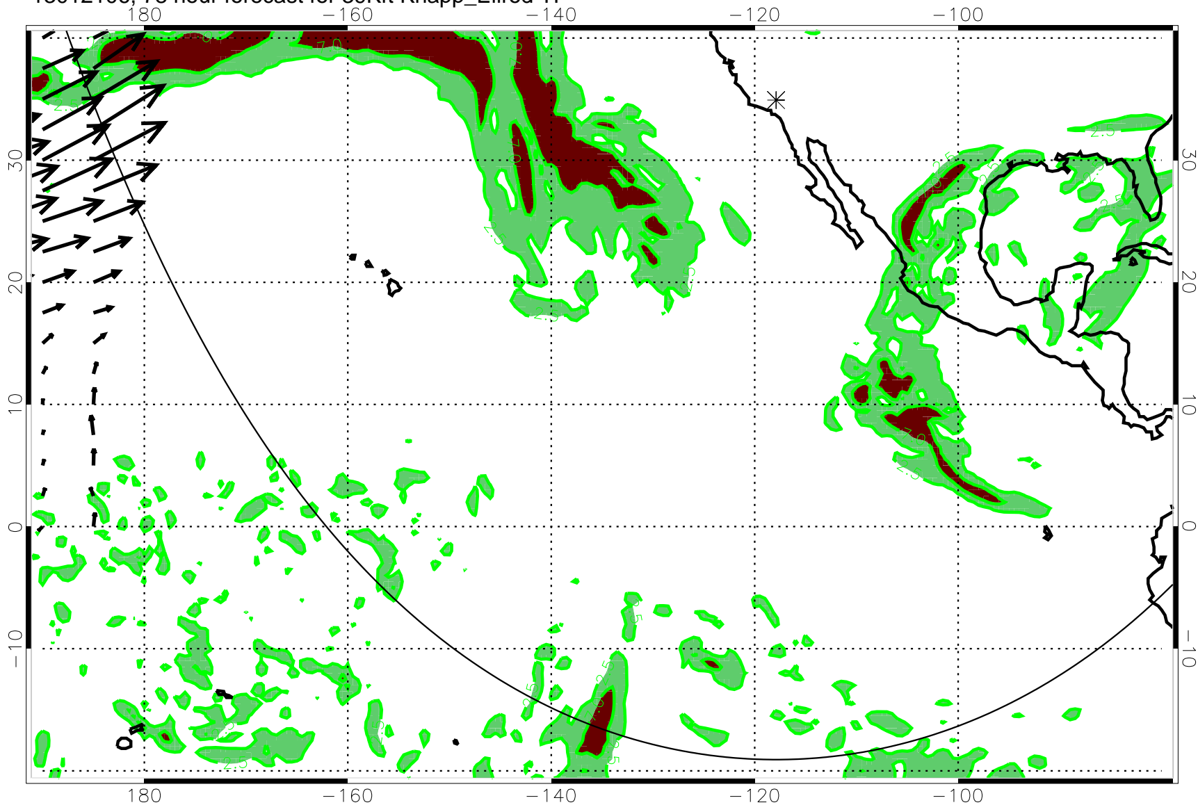
13012106, 78 hour forecast for 39Kft Knapp_Ellrod TI
