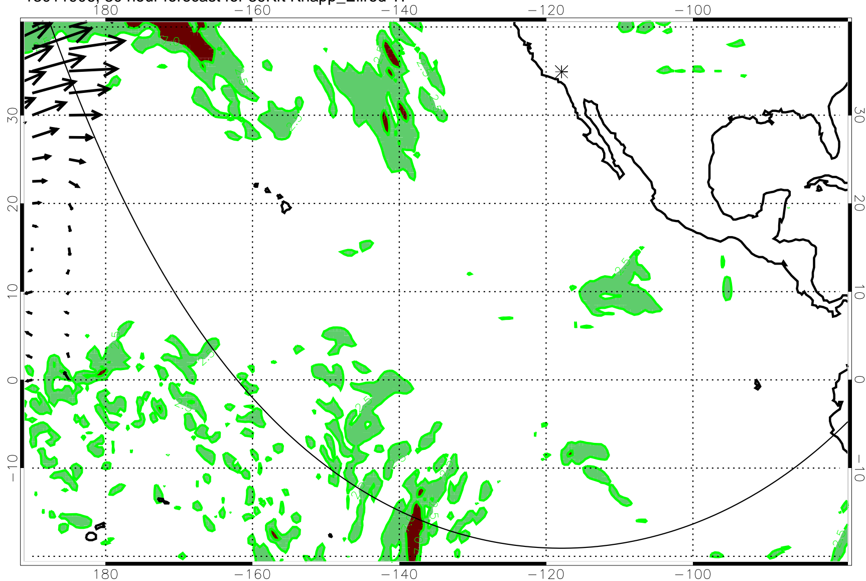
13011906, 30 hour forecast for 39Kft Knapp_Ellrod TI
