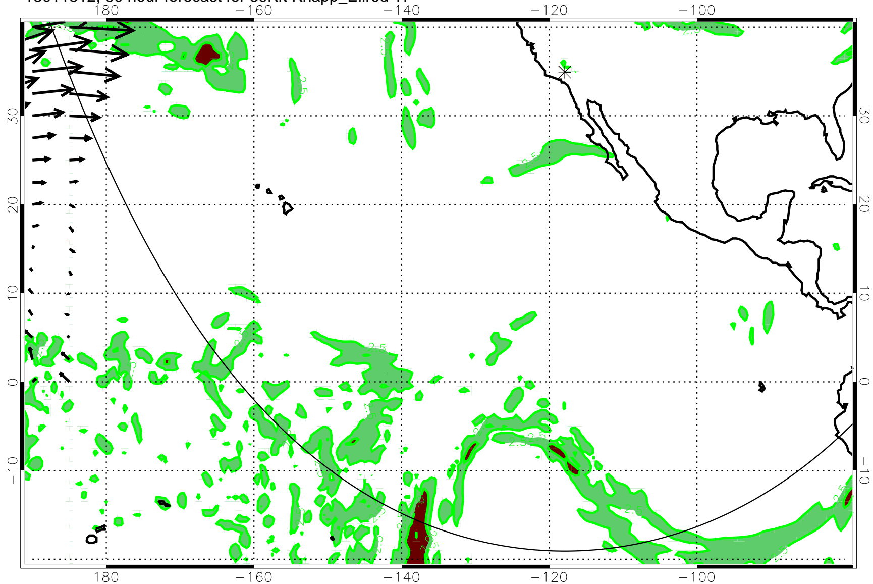
13011812, 60 hour forecast for 39Kft Knapp_Ellrod TI
