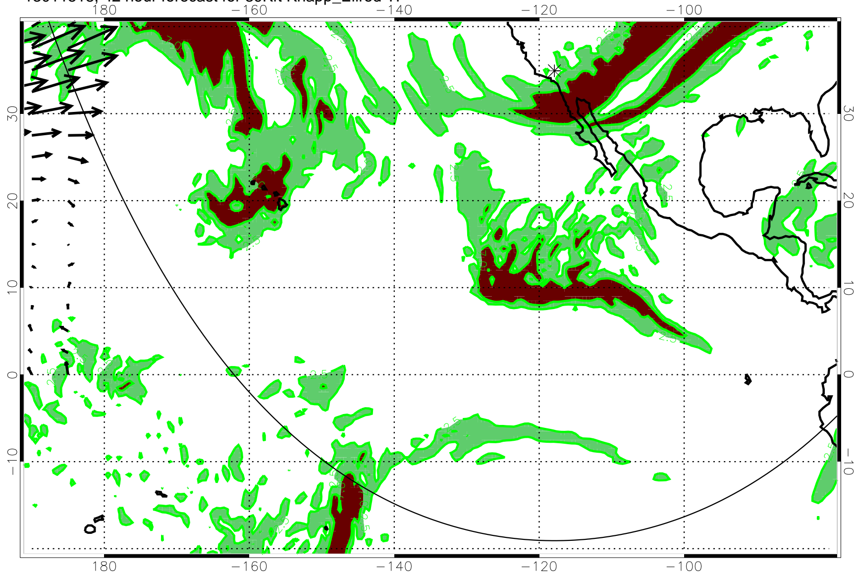
13011518, 42 hour forecast for 39Kft Knapp_Ellrod TI
