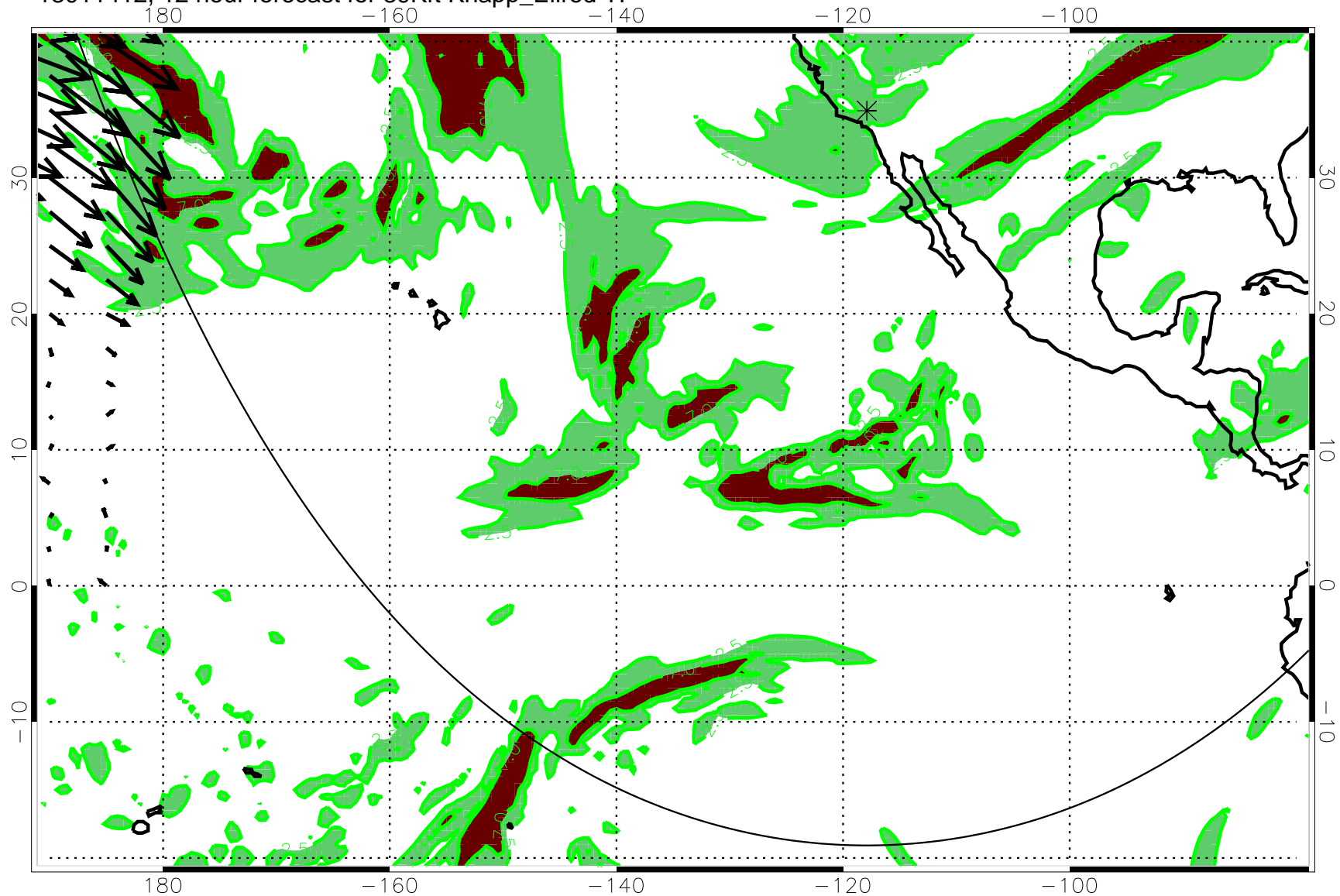
13011412, 12 hour forecast for 39Kft Knapp_Ellrod TI
