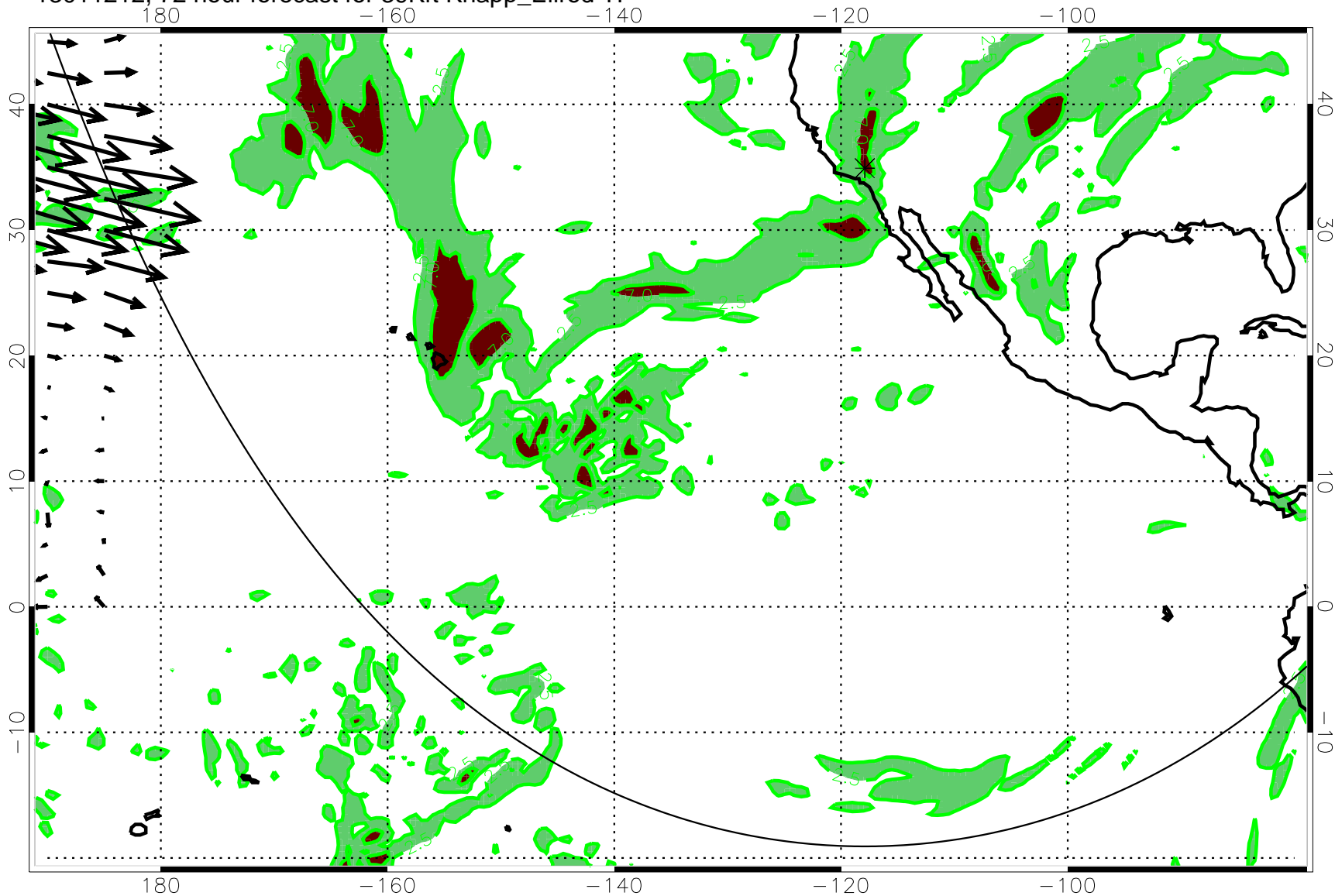
13011212, 72 hour forecast for 39Kft Knapp_Ellrod TI
