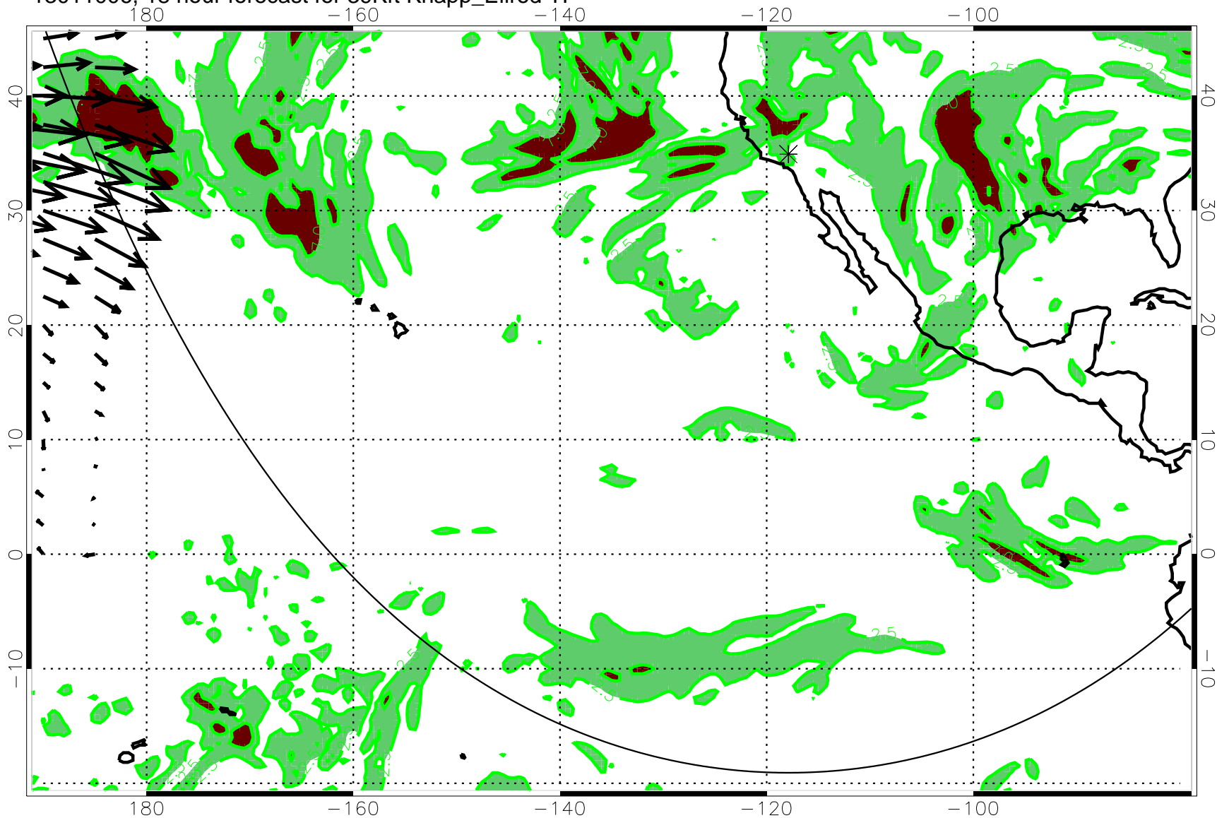
13011006, 18 hour forecast for 39Kft Knapp_Ellrod TI
