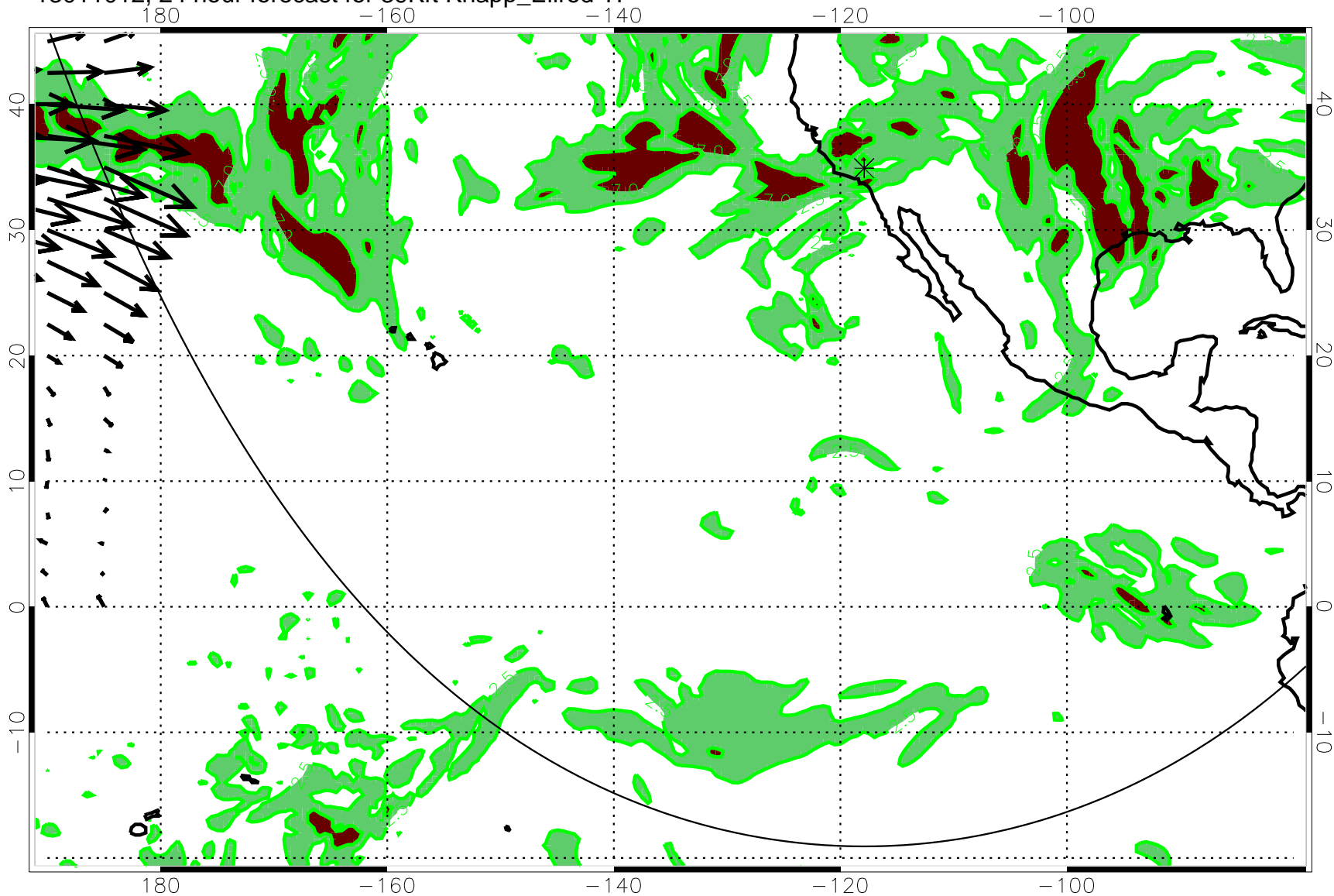
13011012, 24 hour forecast for 39Kft Knapp_Ellrod TI
