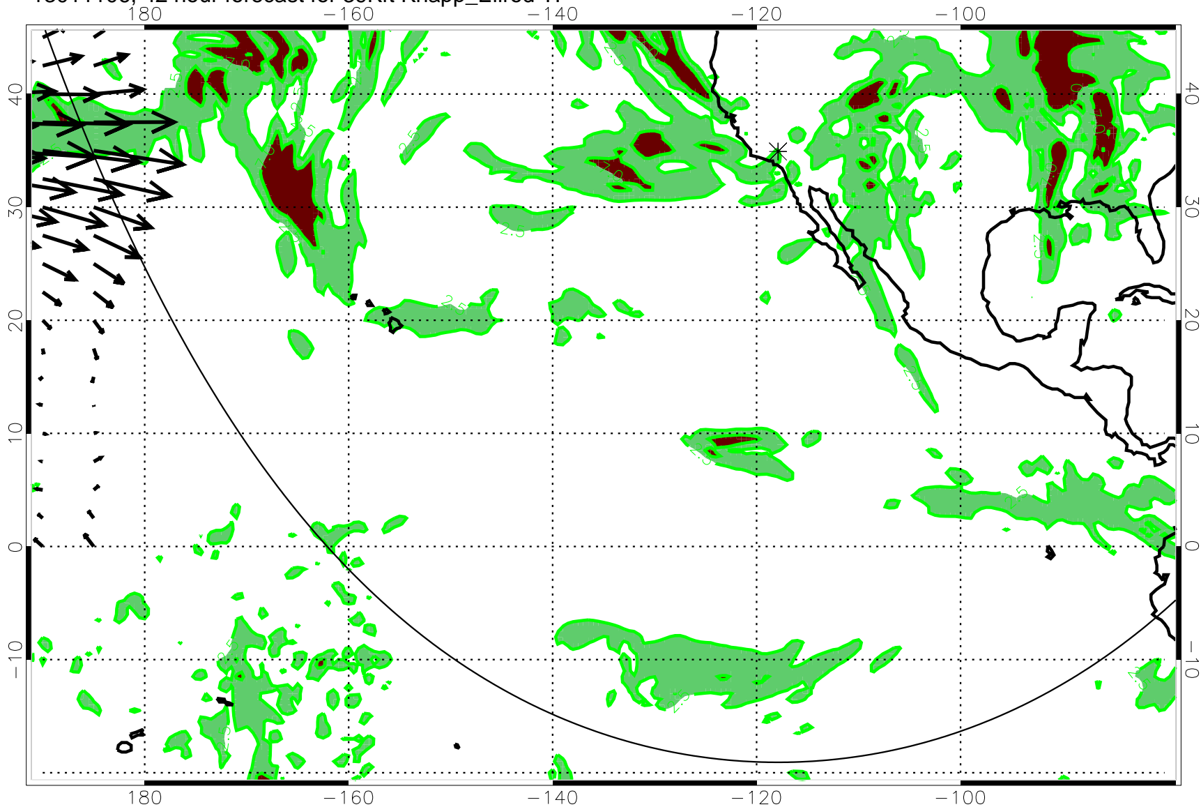
13011106, 42 hour forecast for 39Kft Knapp_Ellrod TI
