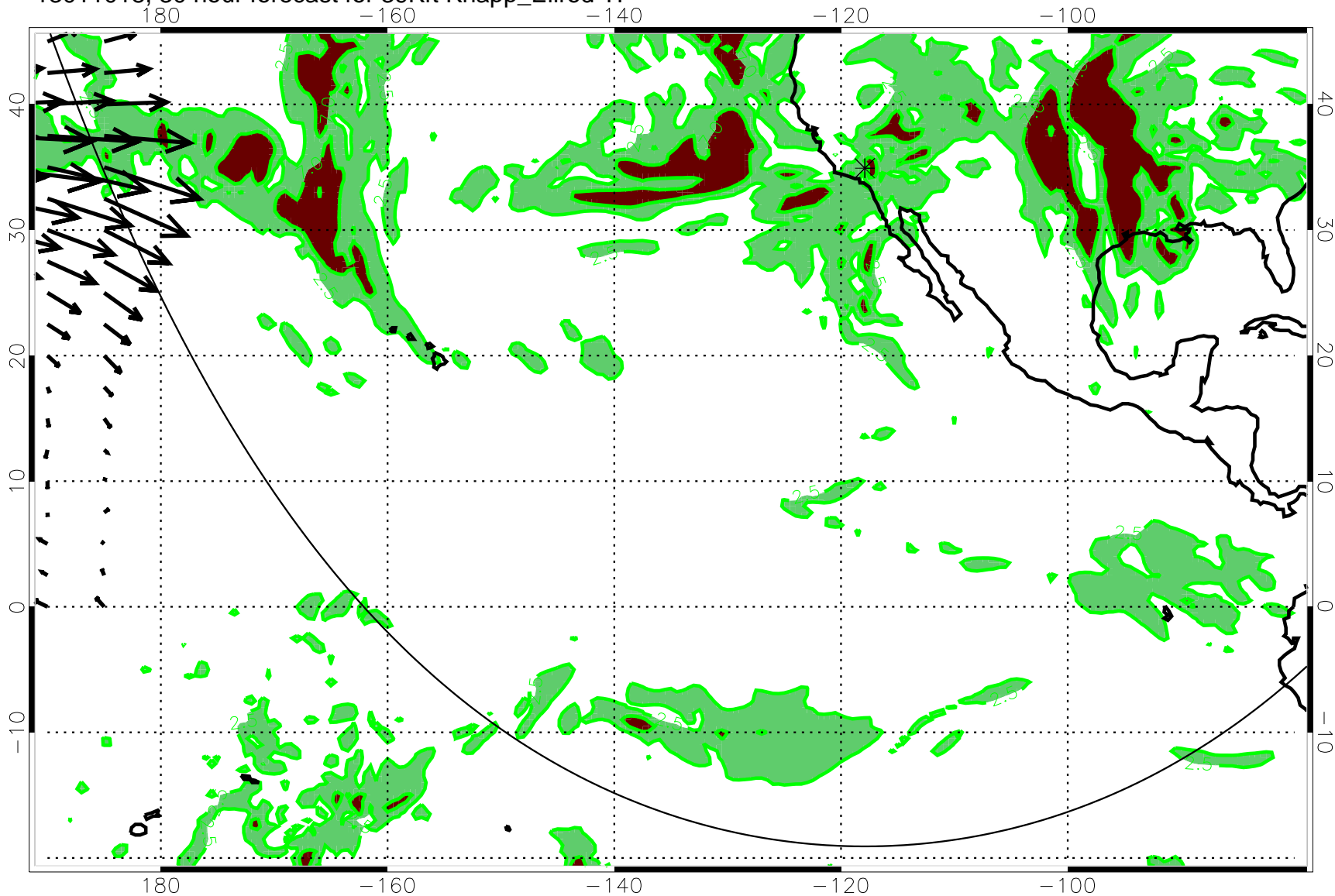
13011018, 30 hour forecast for 39Kft Knapp_Ellrod TI
