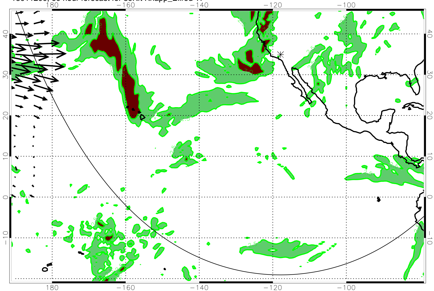
13011200, 60 hour forecast for 39Kft Knapp_Ellrod TI
