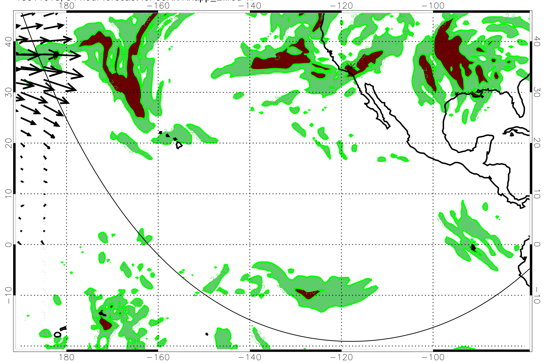
13011018, 54 hour forecast for 39Kft Knapp_Ellrod TI
