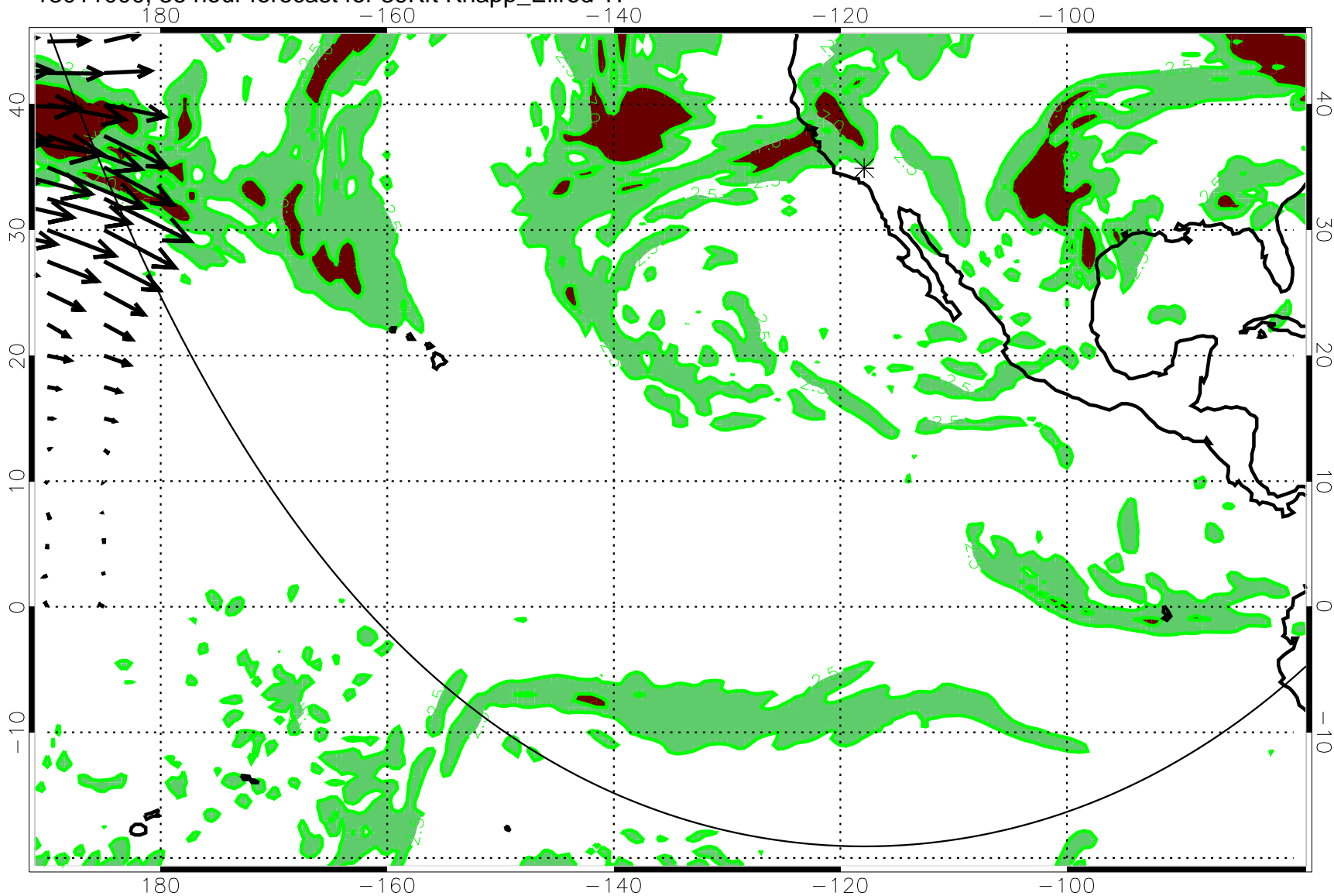
13011000, 36 hour forecast for 39Kft Knapp_Ellrod TI
