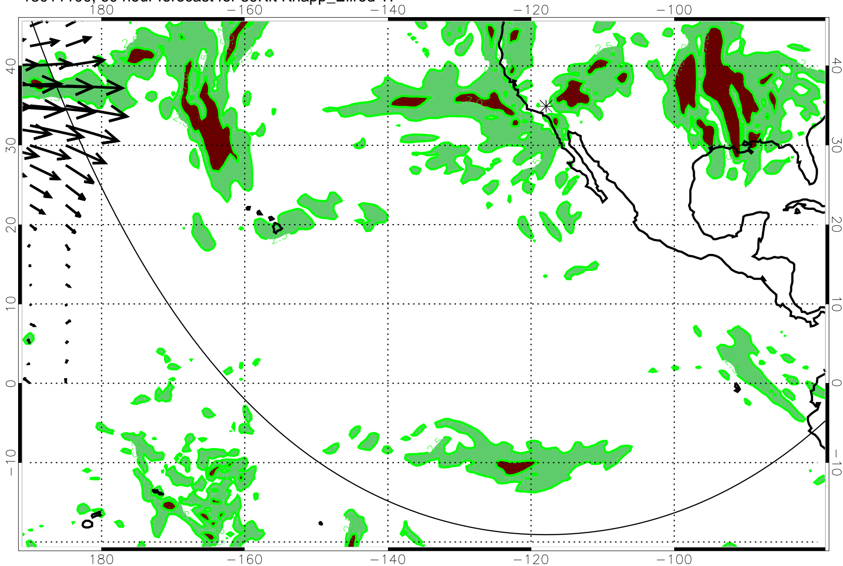
13011100, 60 hour forecast for 39Kft Knapp_Ellrod TI
