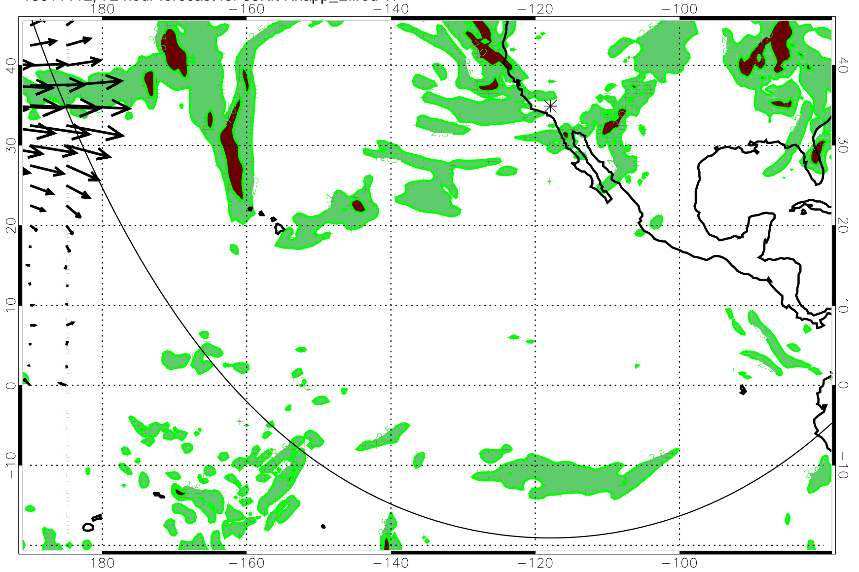
13011112, 72 hour forecast for 39Kft Knapp_Ellrod TI
