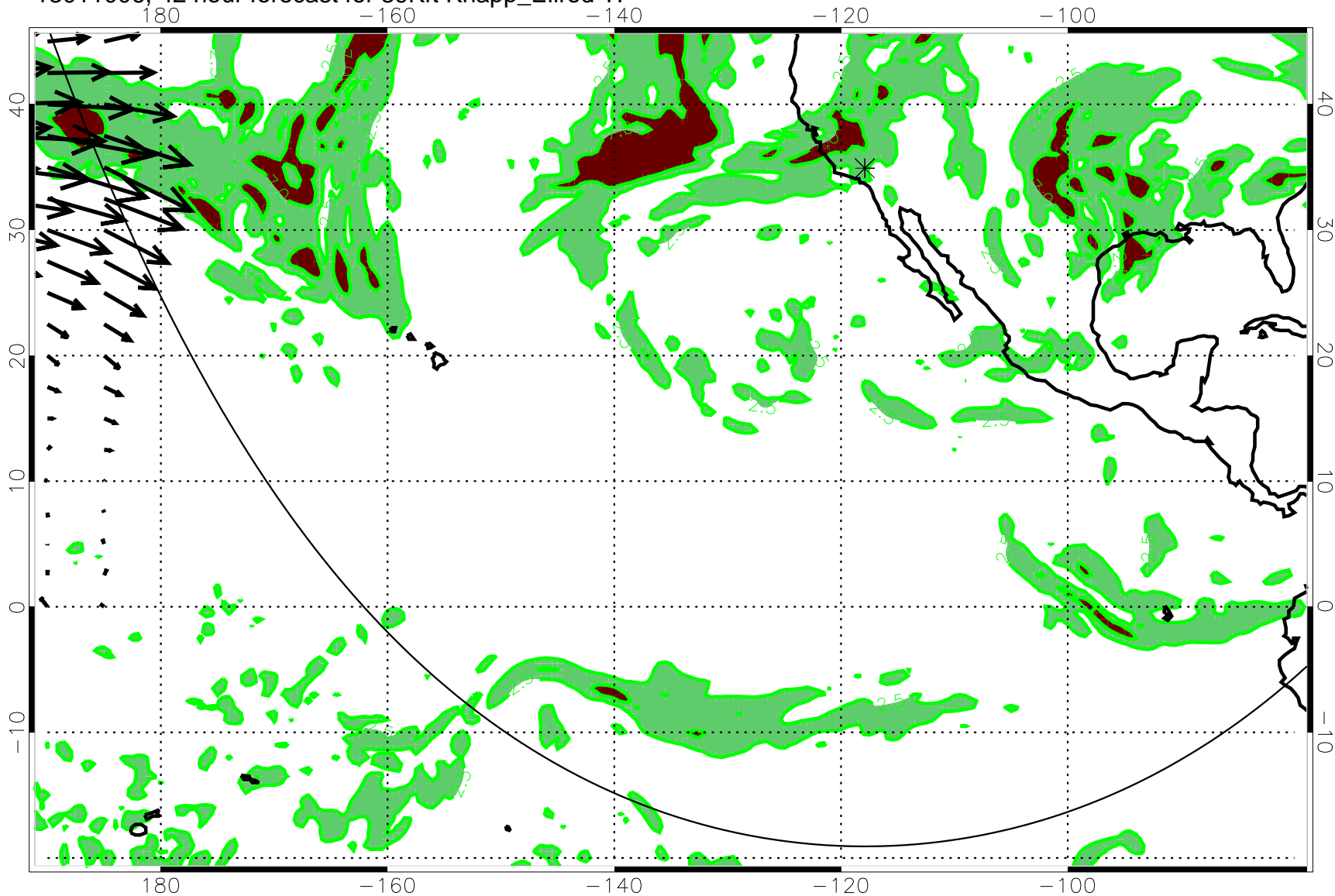
13011006, 42 hour forecast for 39Kft Knapp_Ellrod TI
