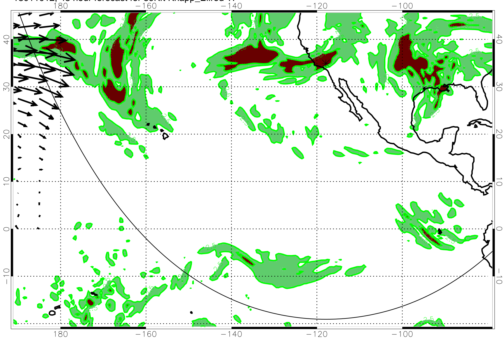
13011012, 48 hour forecast for 39Kft Knapp_Ellrod TI
