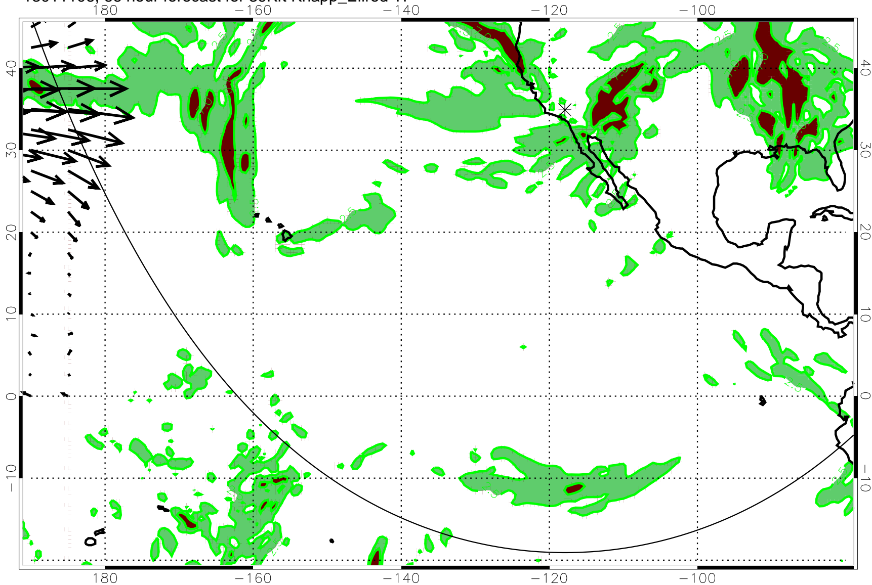
13011106, 66 hour forecast for 39Kft Knapp_Ellrod TI
