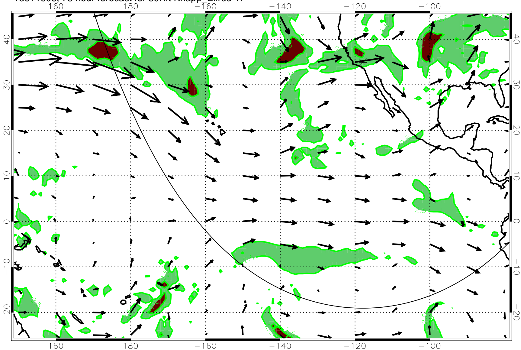
13011006, 78 hour forecast for 39Kft Knapp_Ellrod T1
