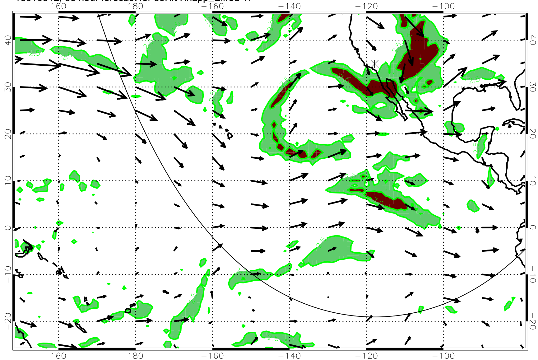
13010812, 36 hour forecast for 39Kft Knapp_Ellrod T1
