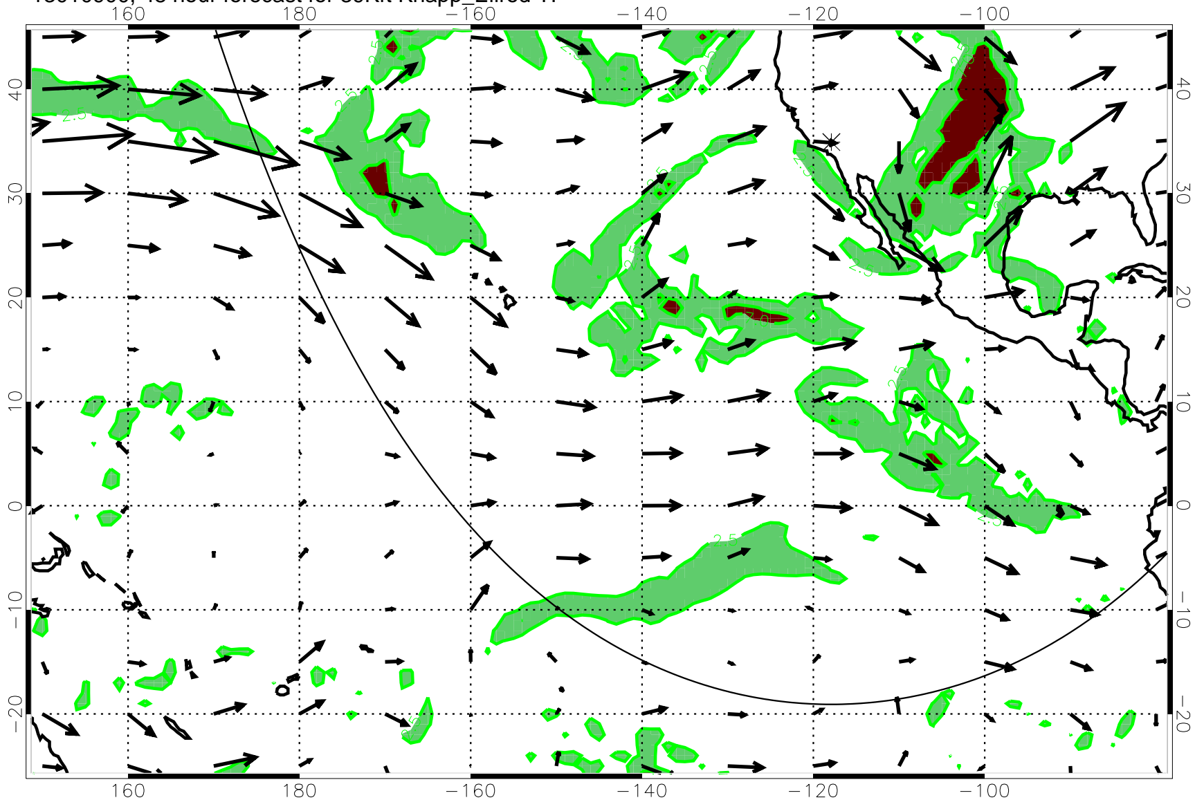
13010900, 48 hour forecast for 39Kft Knapp_Ellrod T1
