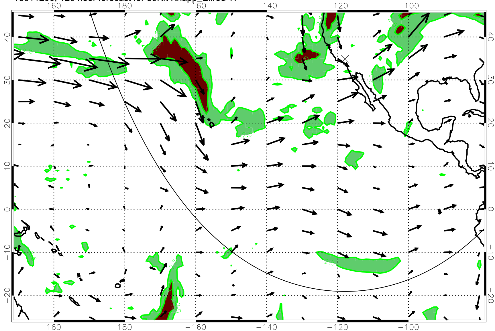
13011200, 120 hour forecast for 39Kft Knapp_Ellrod T1
