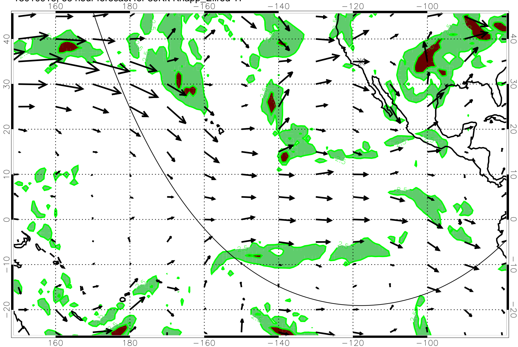
13010918, 66 hour forecast for 39Kft Knapp_Ellrod T1
