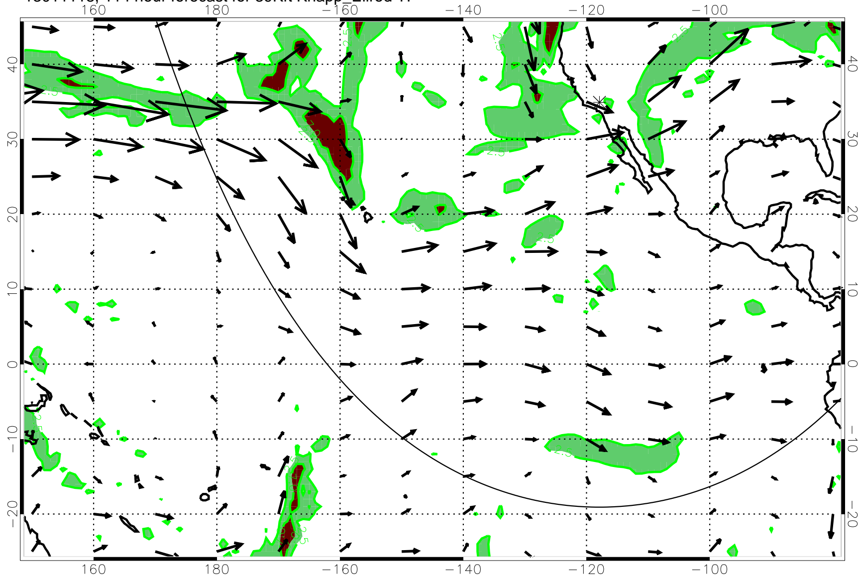
13011118, 114 hour forecast for 39Kft Knapp_Ellrod T1
