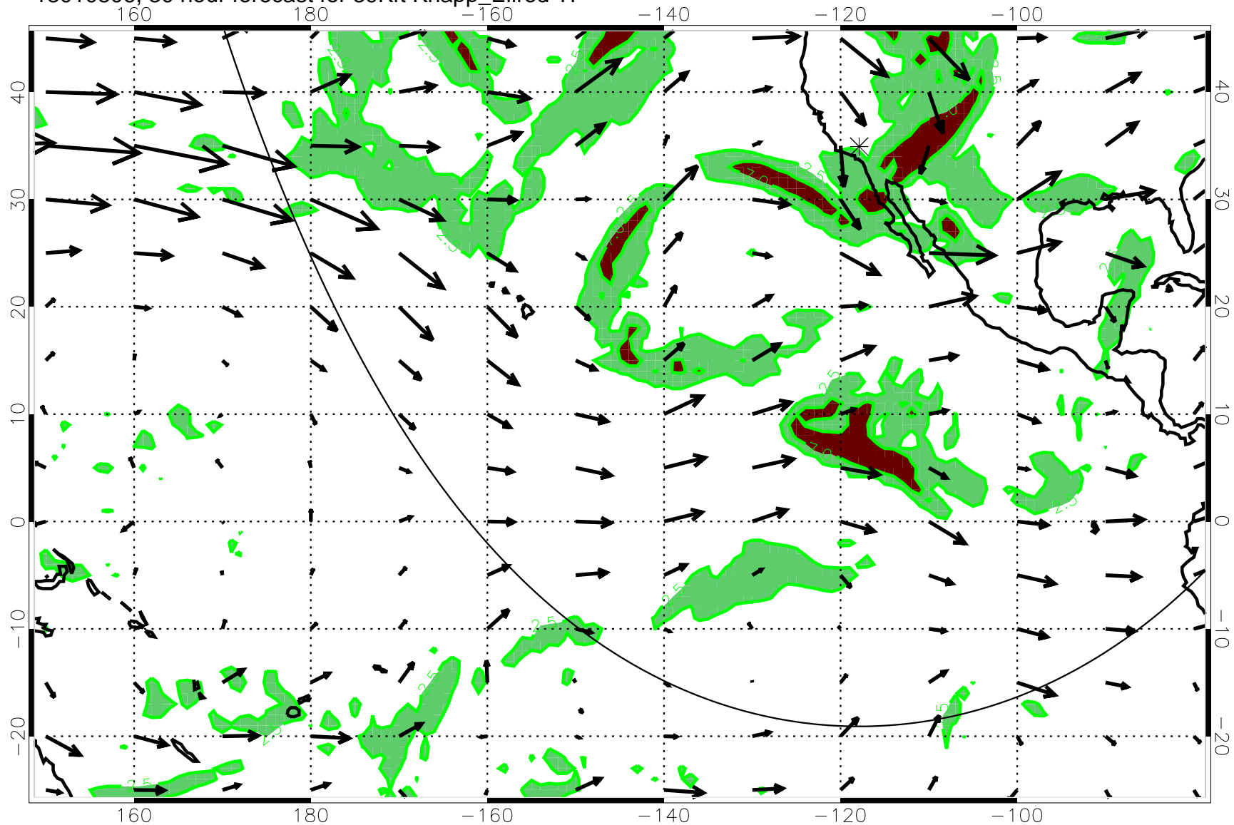
13010806, 30 hour forecast for 39Kft Knapp_Ellrod T1
