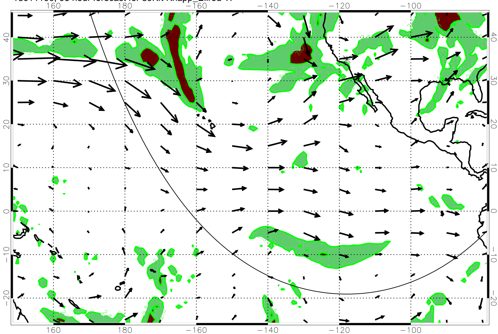
13011100, 96 hour forecast for 39Kft Knapp_Ellrod T1
