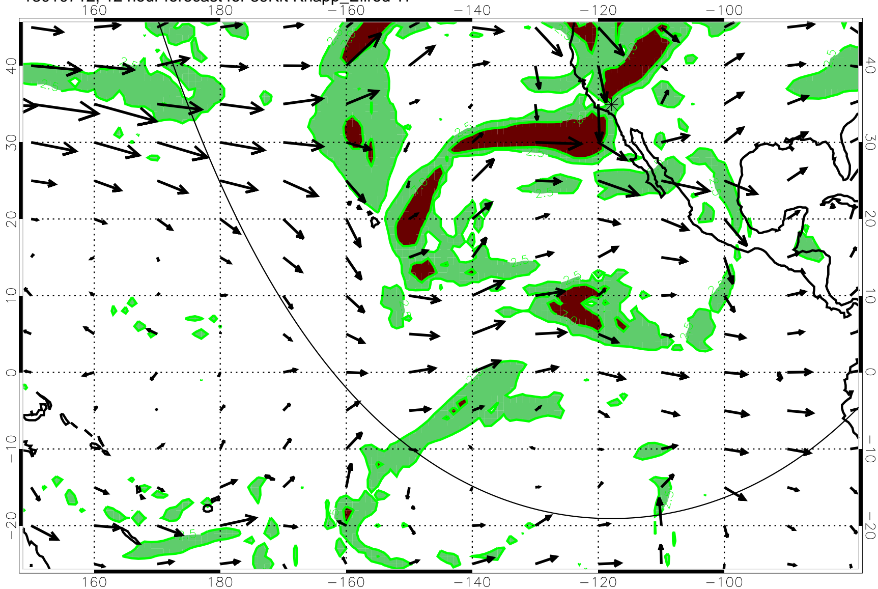
13010712, 12 hour forecast for 39Kft Knapp_Ellrod T1
