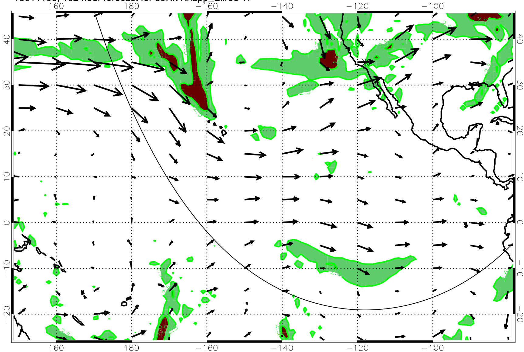
13011106, 102 hour forecast for 39Kft Knapp_Ellrod T1
