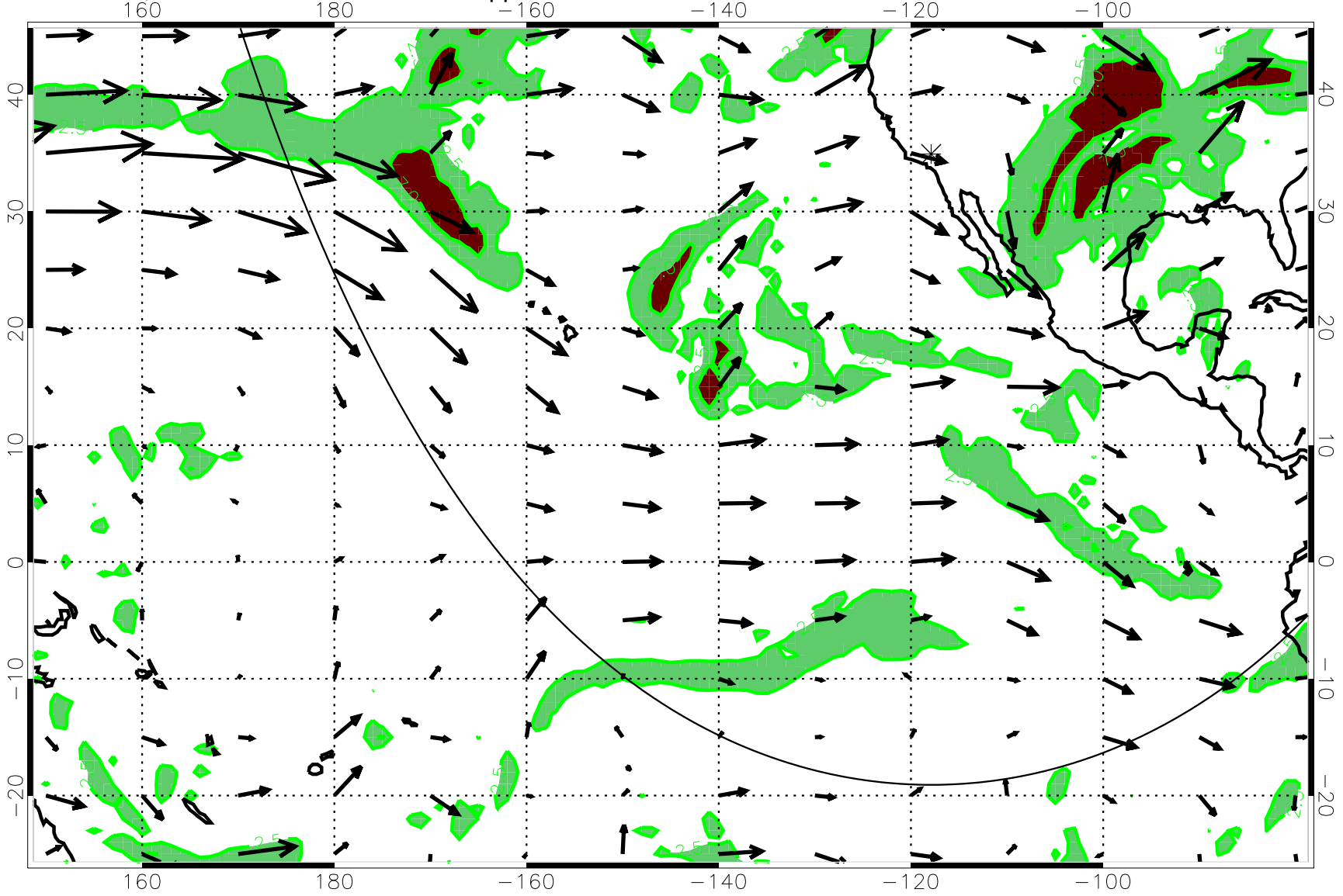
13010906, 54 hour forecast for 39Kft Knapp_Ellrod T1
