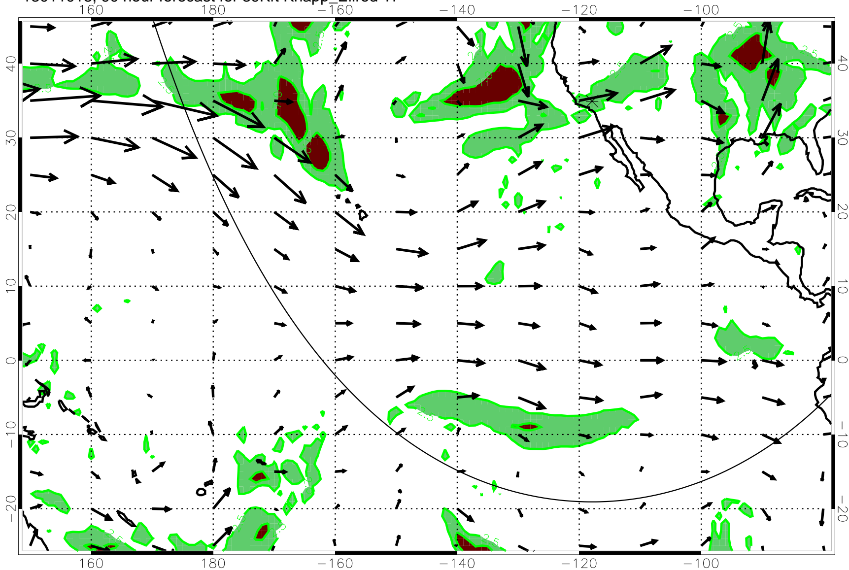
13011018, 90 hour forecast for 39Kft Knapp_Ellrod T1
