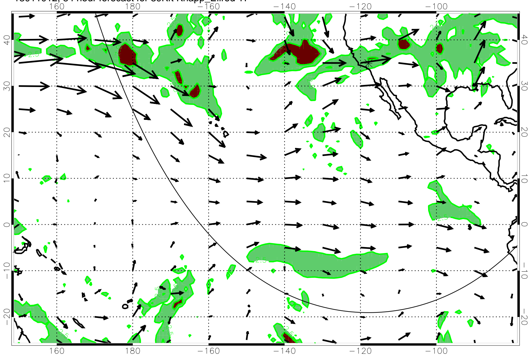
13011012, 84 hour forecast for 39Kft Knapp_Ellrod T1
