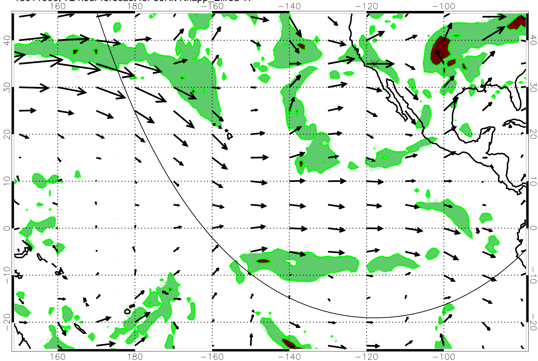
13011000, 72 hour forecast for 39Kft Knapp_Ellrod T1
