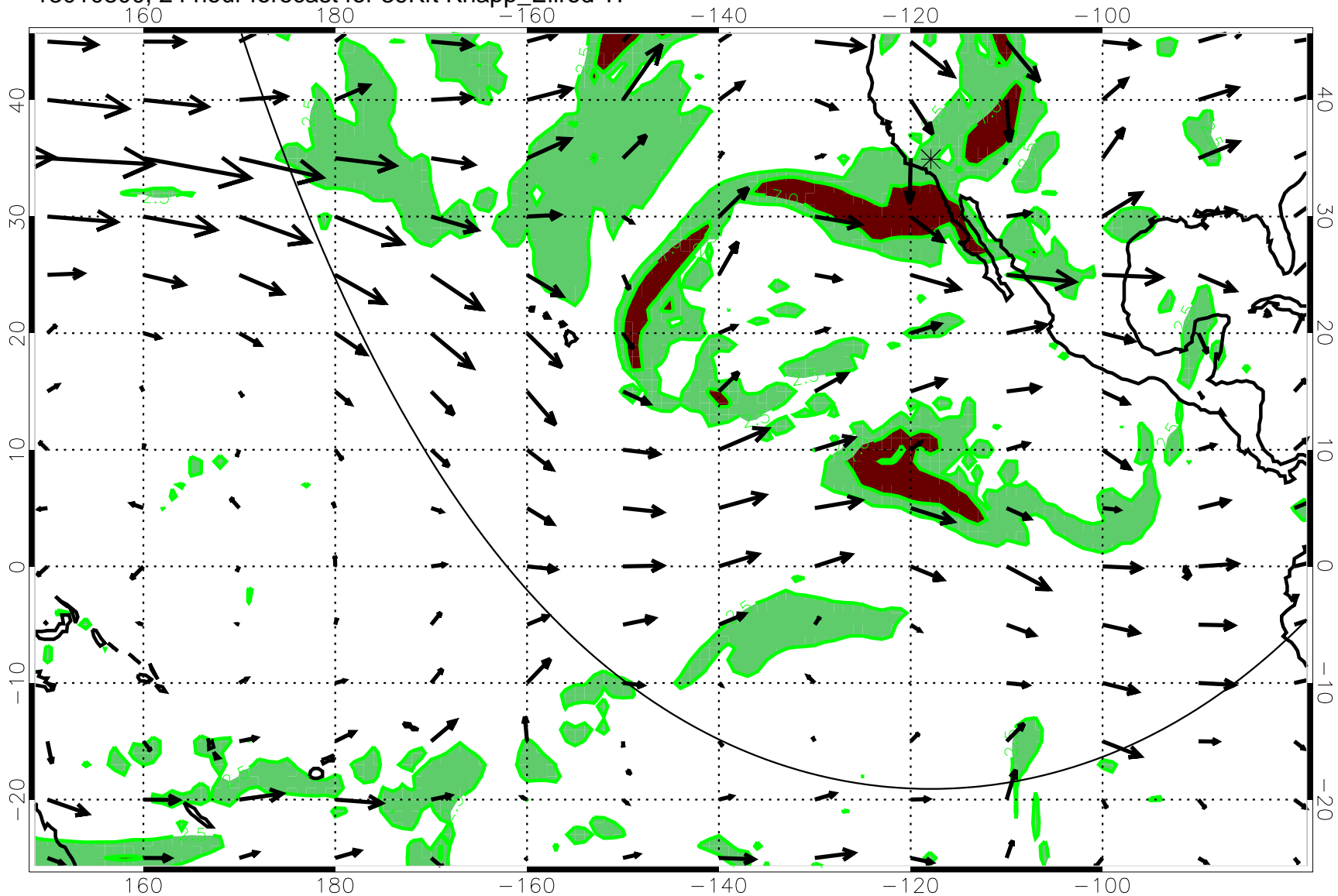
13010800, 24 hour forecast for 39Kft Knapp_Ellrod T1
