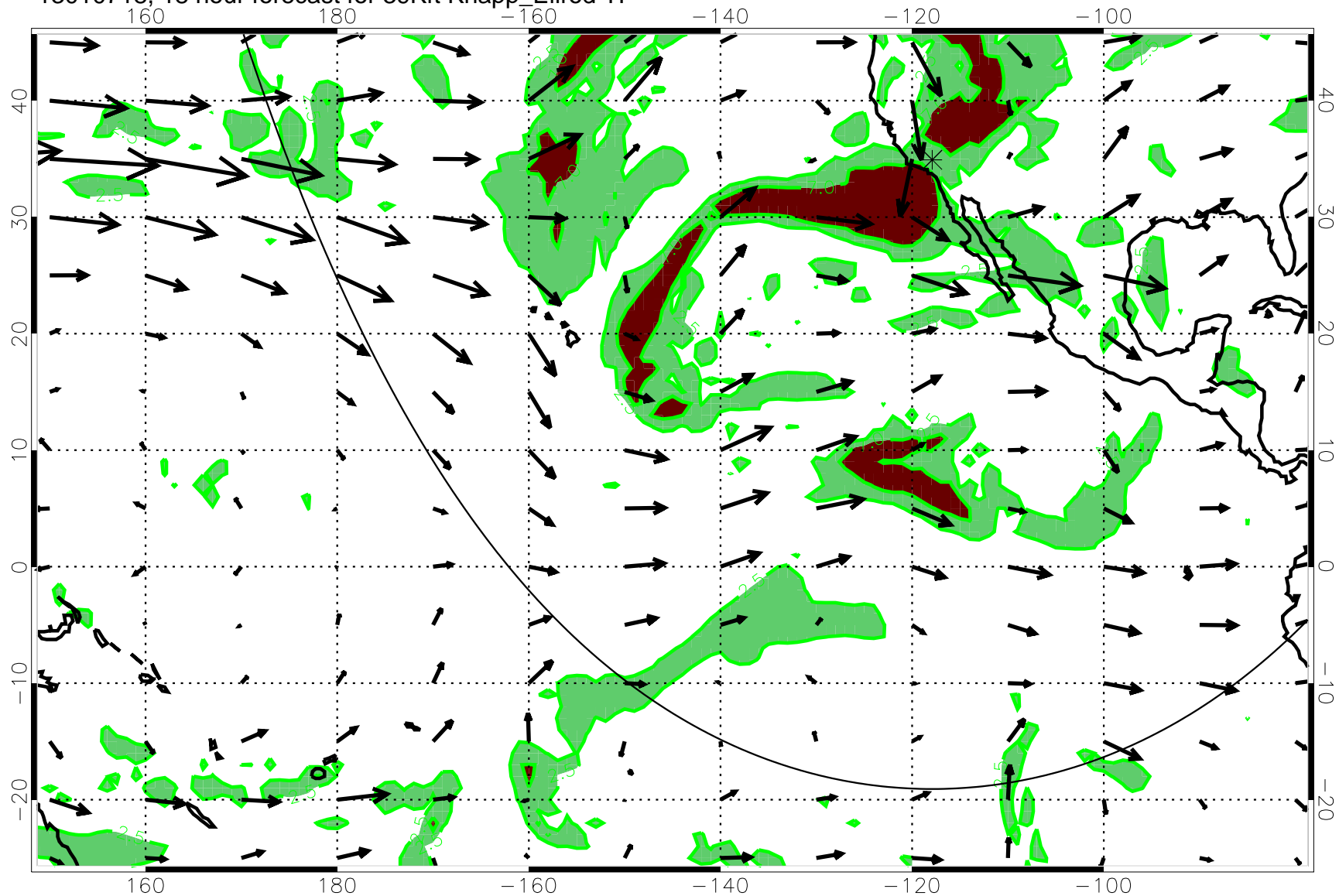
13010718, 18 hour forecast for 39Kft Knapp_Ellrod T1
