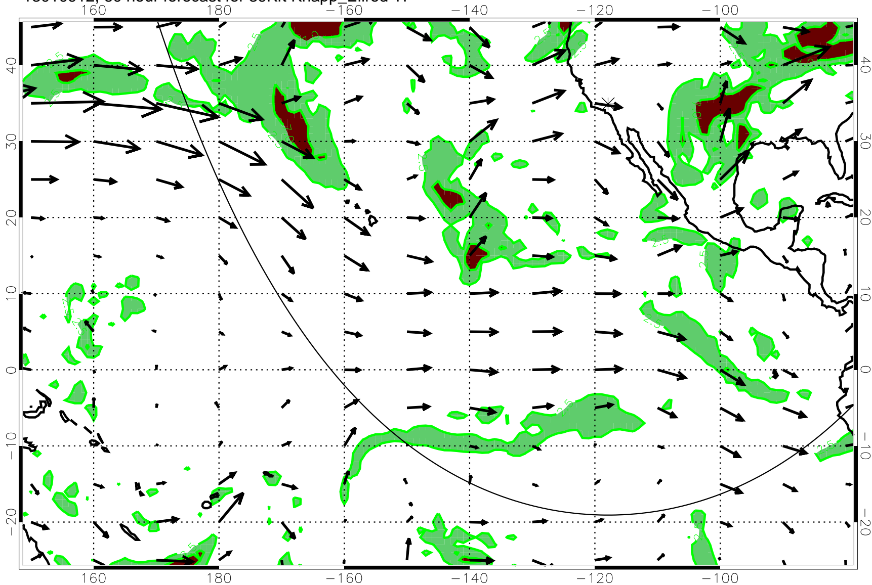
13010912, 60 hour forecast for 39Kft Knapp_Ellrod T1
