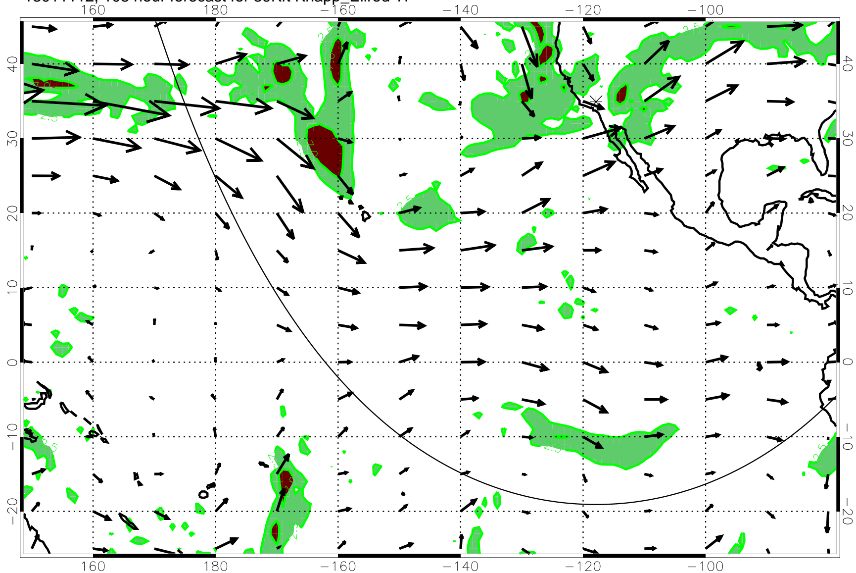
13011112, 108 hour forecast for 39Kft Knapp_Ellrod T1
