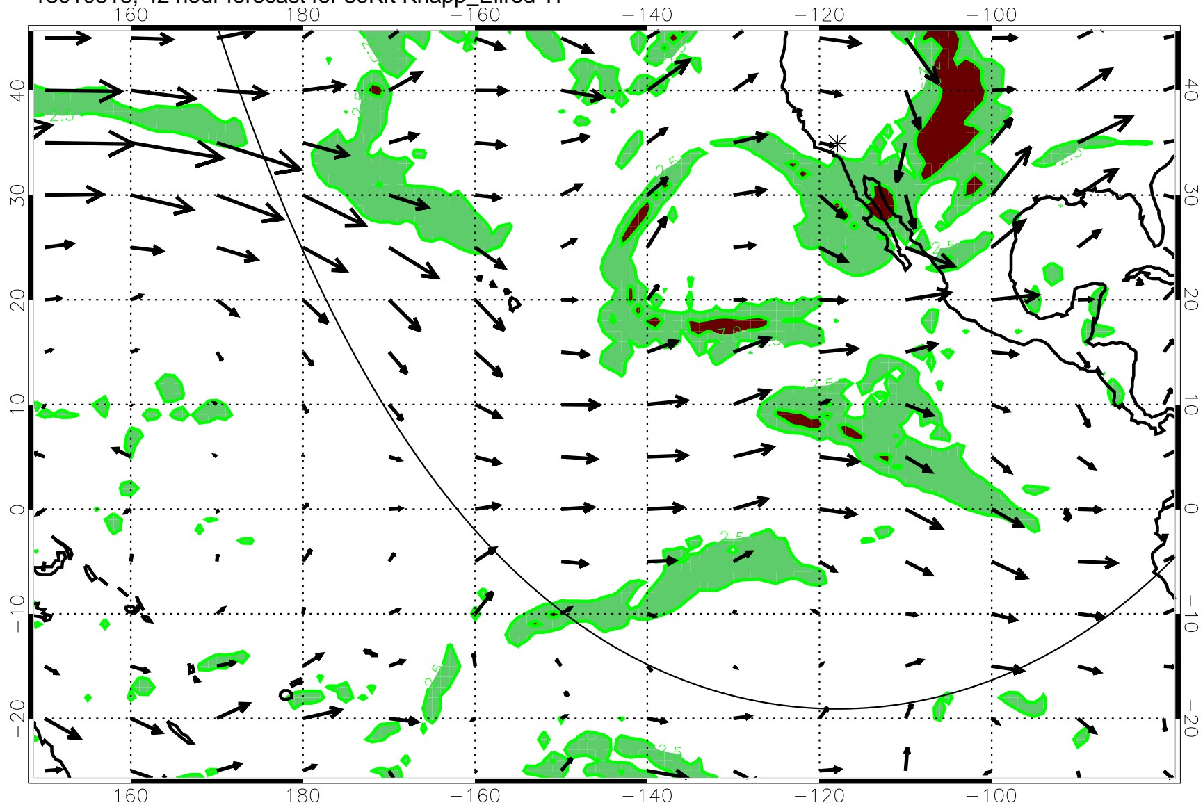
13010818, 42 hour forecast for 39Kft Knapp_Ellrod T1
