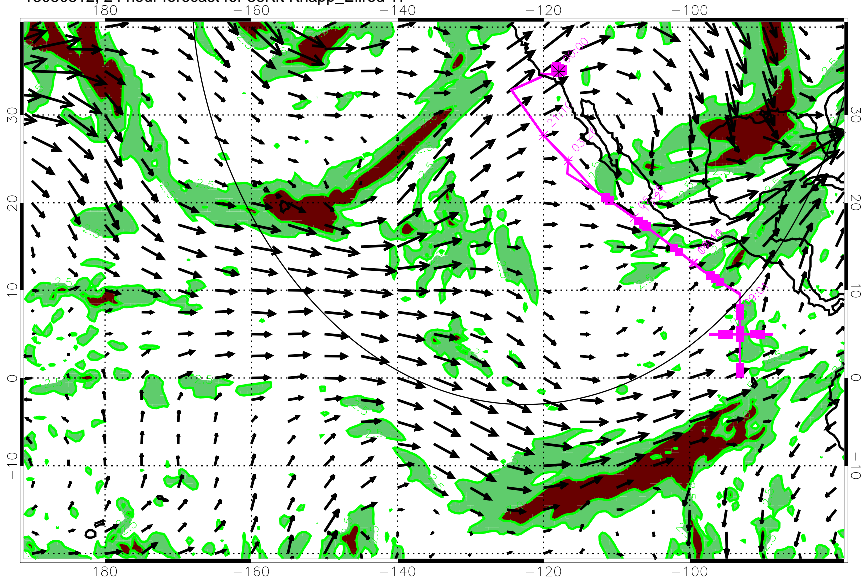
13030312, 24 hour forecast for 36Kft Knapp_Ellrod TI
