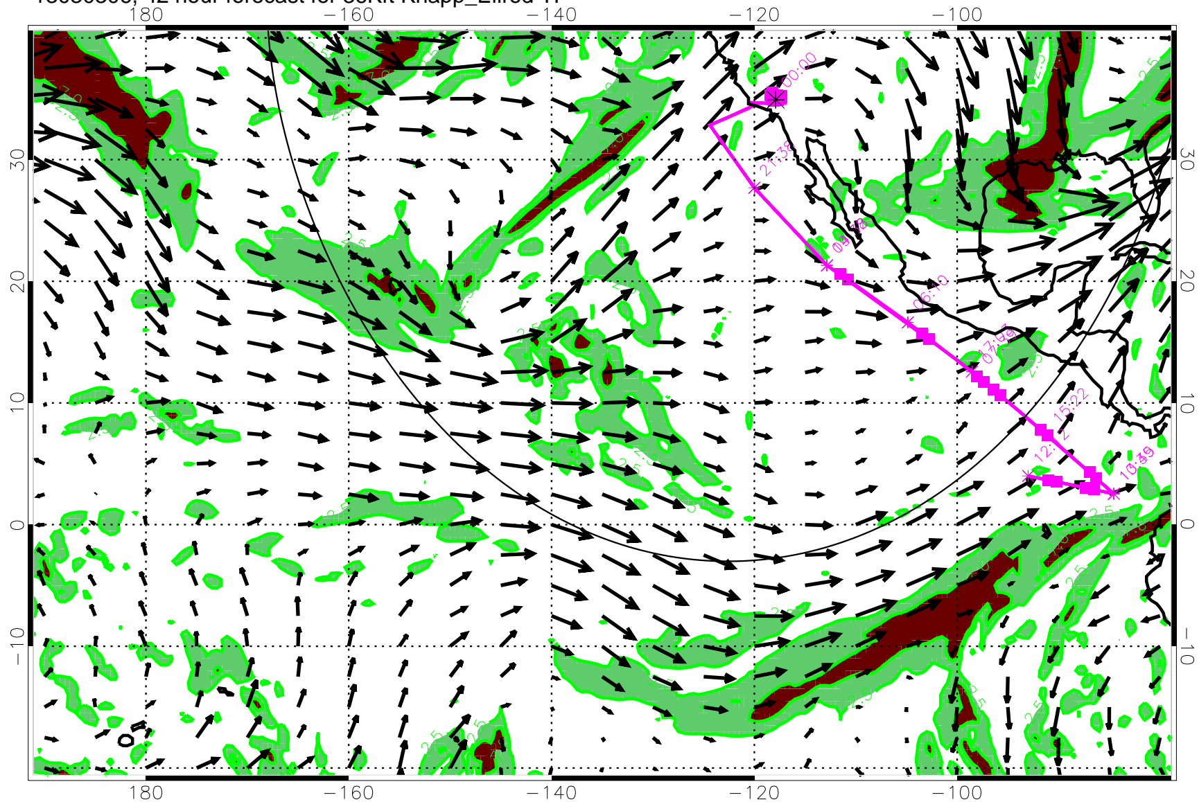
13030306, 42 hour forecast for 36Kft Knapp_Ellrod TI
