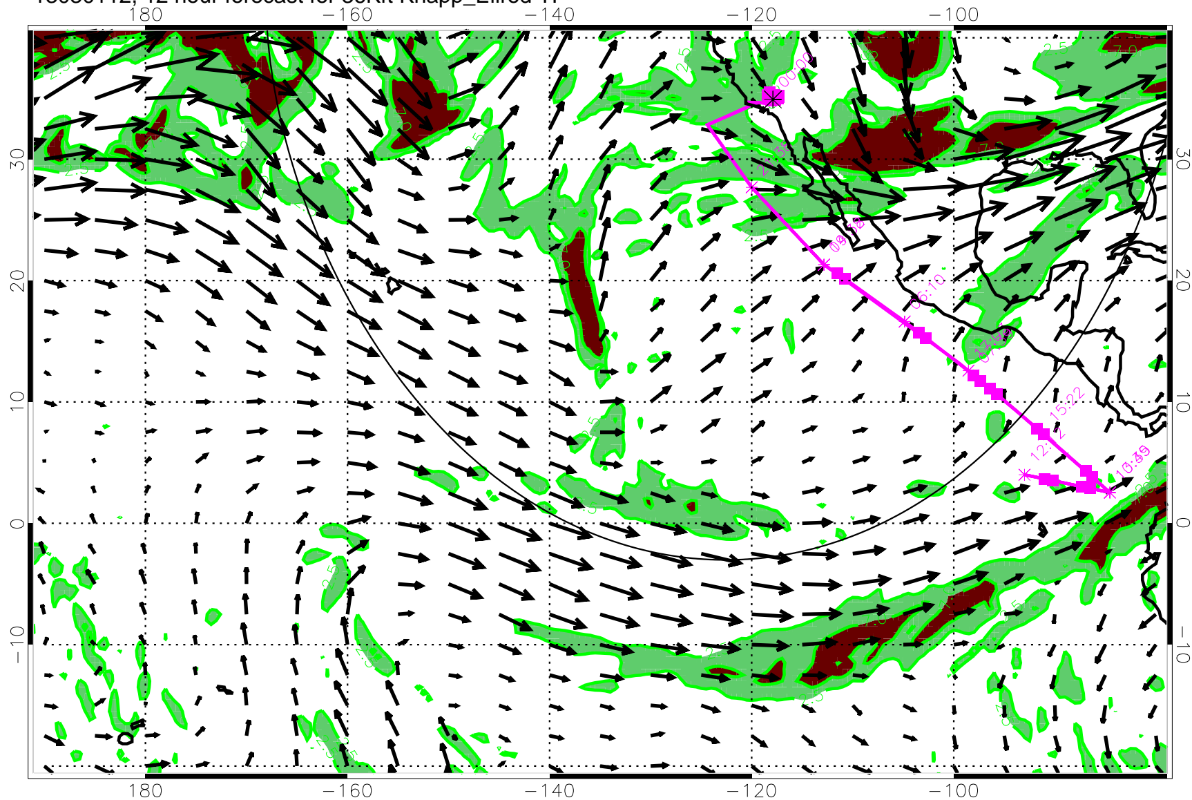
13030112, 12 hour forecast for 36Kft Knapp_Ellrod TI
