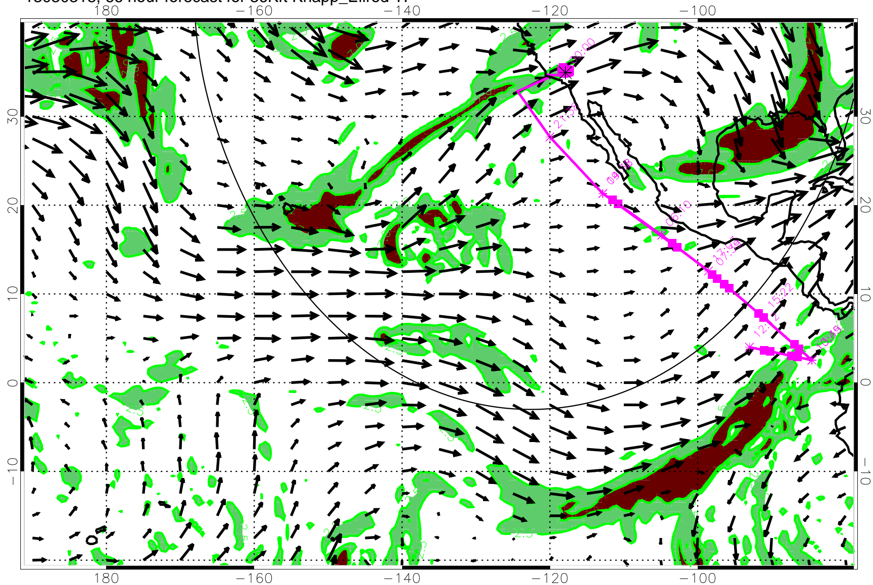
13030318, 66 hour forecast for 36Kft Knapp_Ellrod TI
