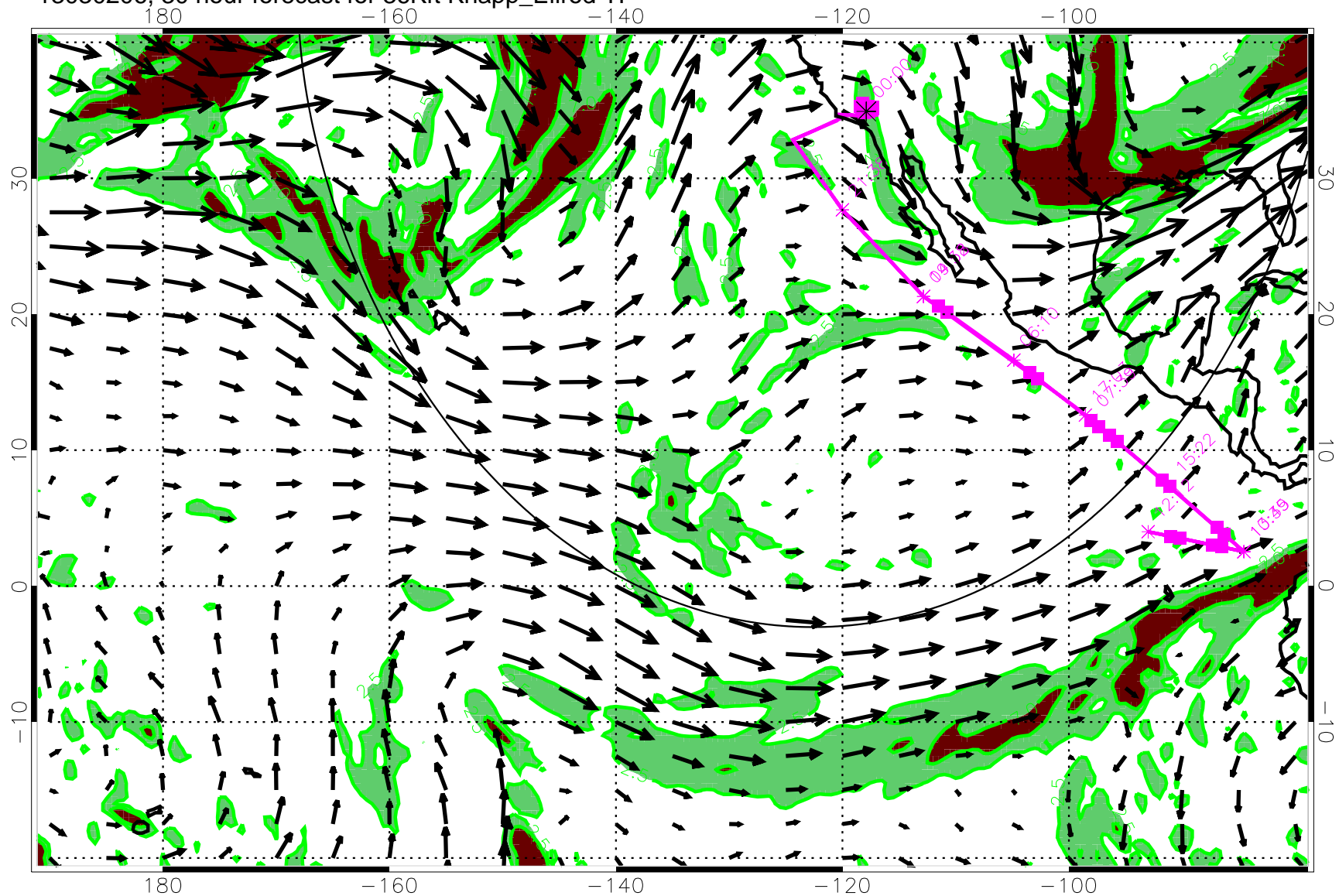
13030206, 30 hour forecast for 36Kft Knapp_Ellrod TI
