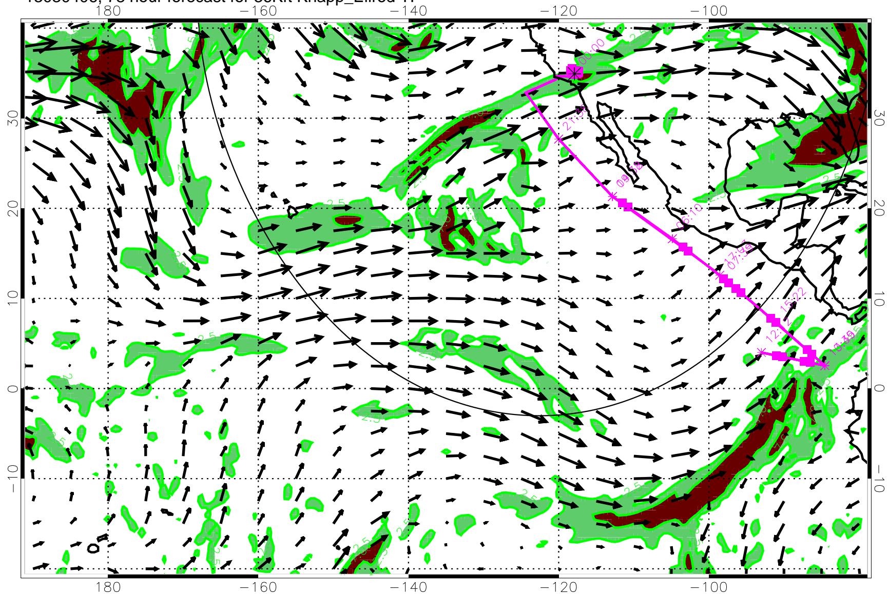
13030406, 78 hour forecast for 36Kft Knapp_Ellrod T1
