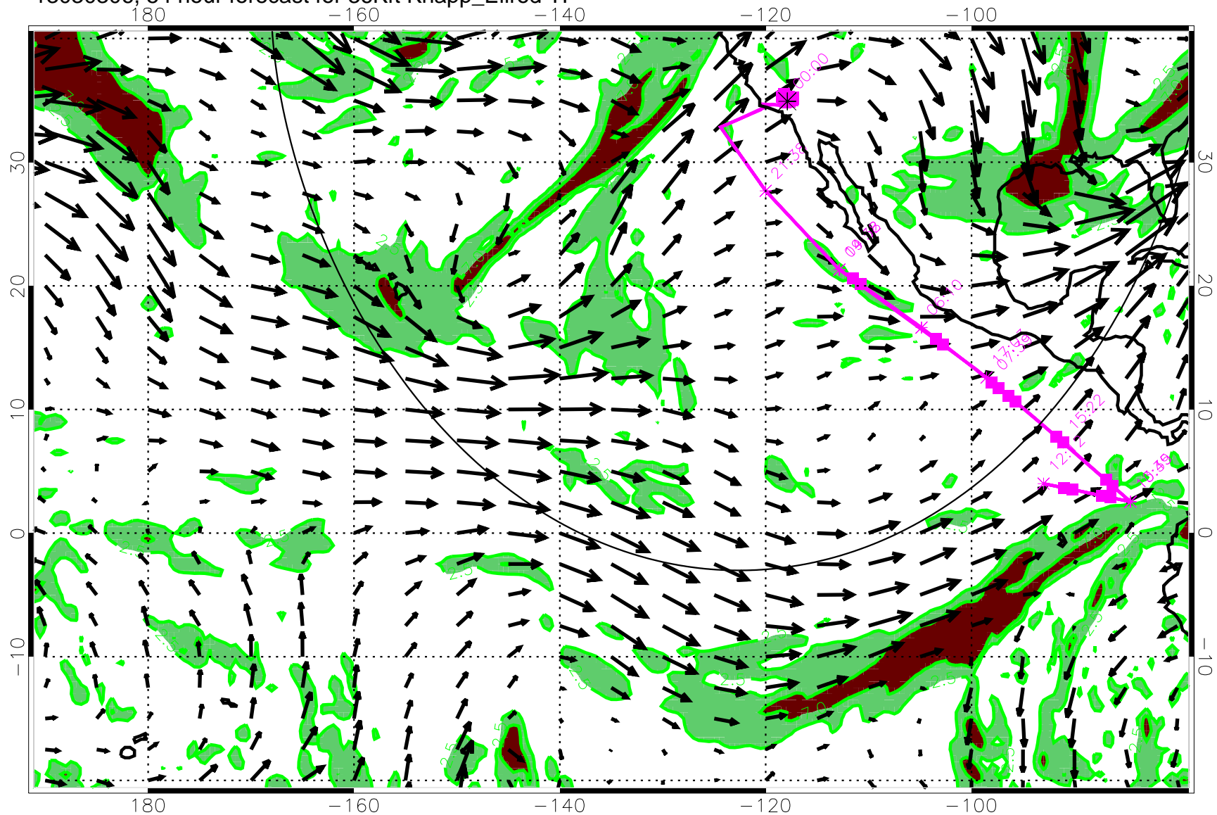
13030306, 54 hour forecast for 36Kft Knapp_Ellrod TI
