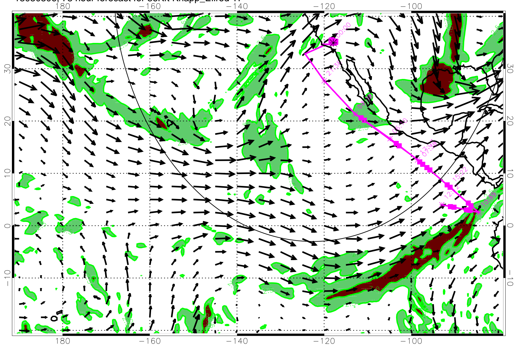
13030306, 78 hour forecast for 36Kft Knapp_Ellrod TI
