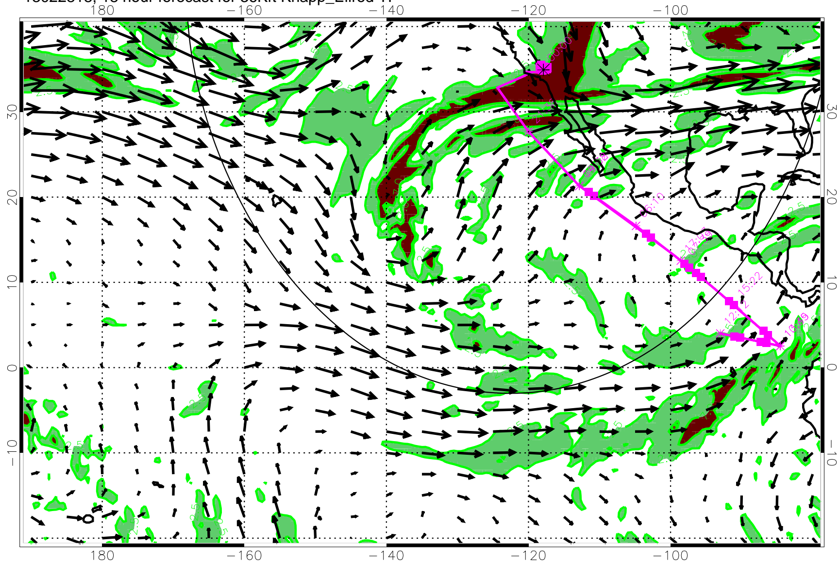
13022818, 18 hour forecast for 36Kft Knapp_Ellrod TI
