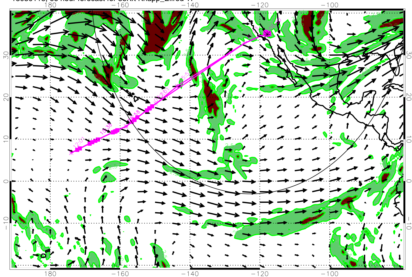
13030118, 66 hour forecast for 36Kft Knapp_Ellrod TI
