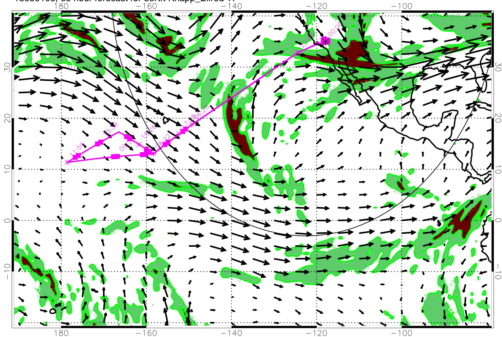
13030106, 66 hour forecast for 36Kft Knapp_Ellrod TI
