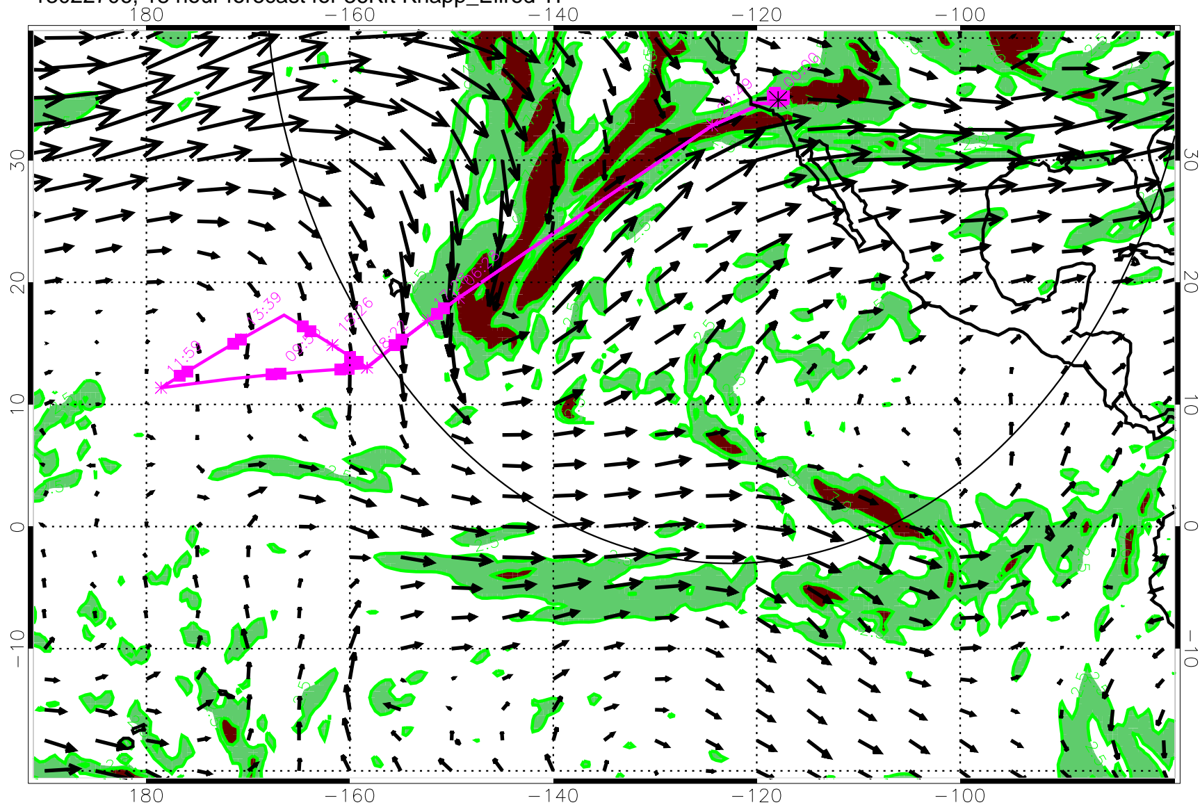
13022706, 18 hour forecast for 36Kft Knapp_Ellrod TI
