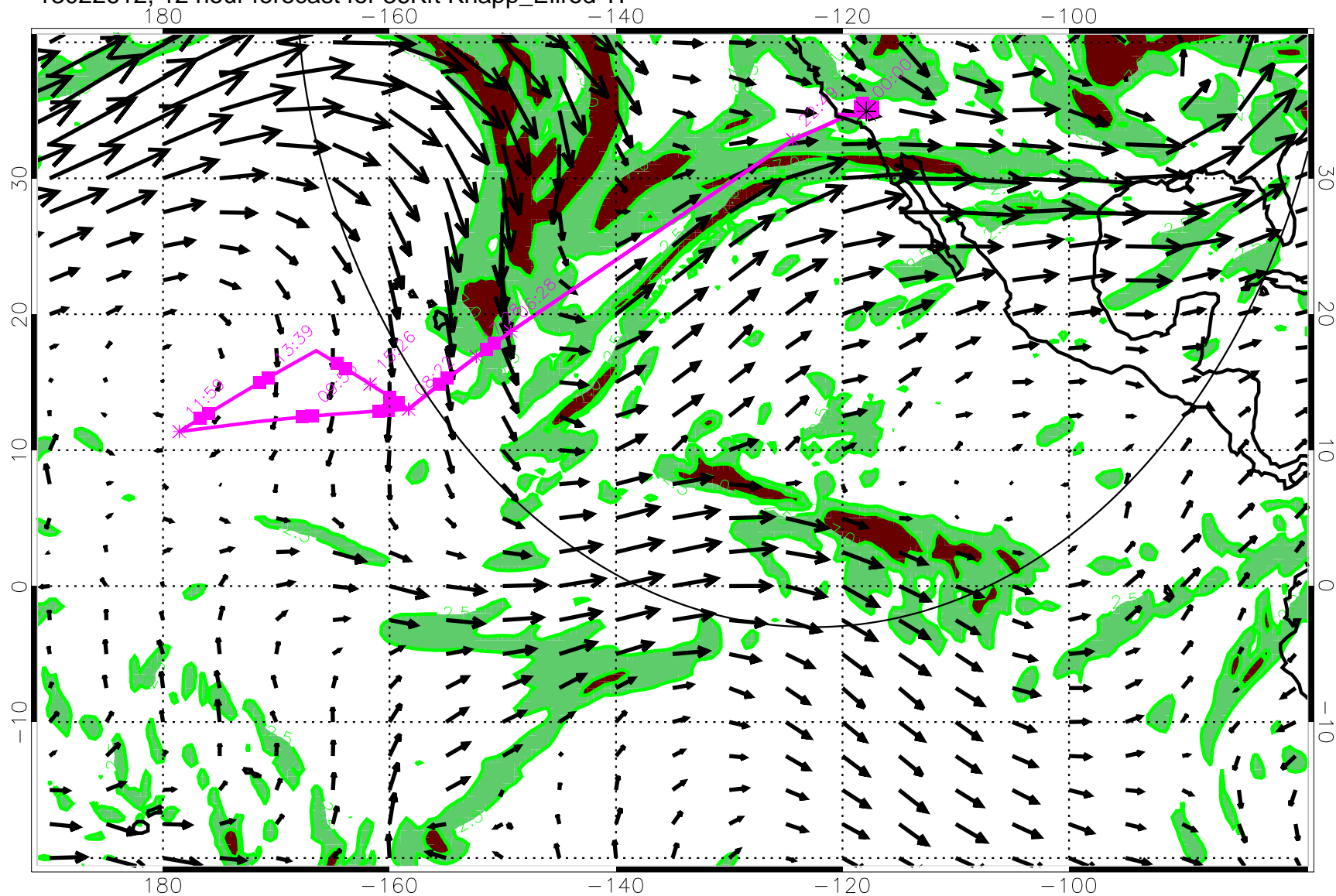
13022612, 12 hour forecast for 36Kft Knapp_Ellrod TI
