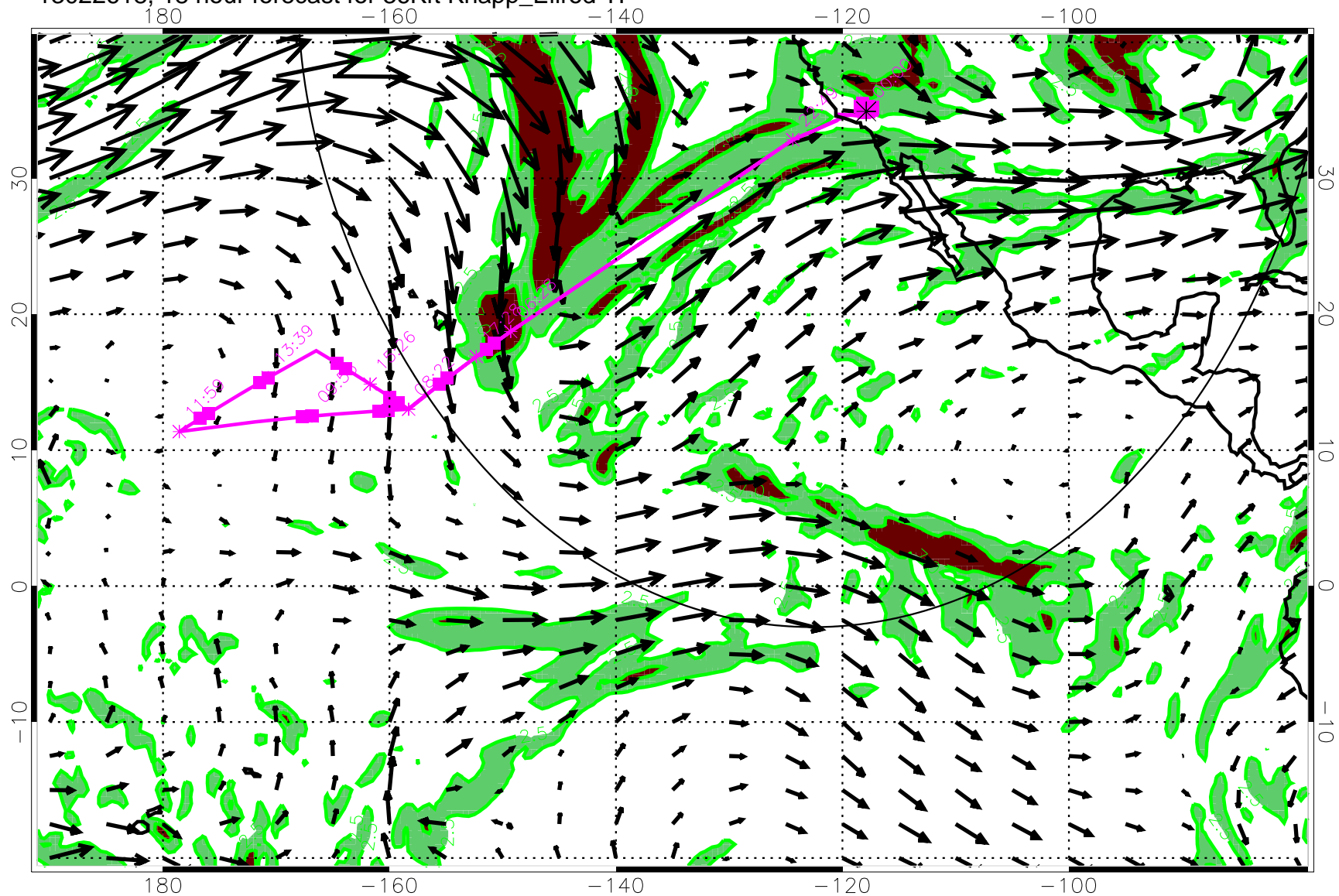
13022618, 18 hour forecast for 36Kft Knapp_Ellrod TI
