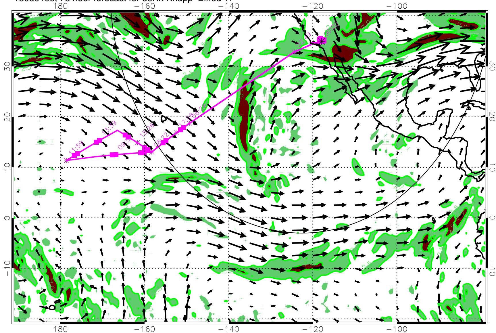
13030106, 78 hour forecast for 36Kft Knapp_Ellrod TI
