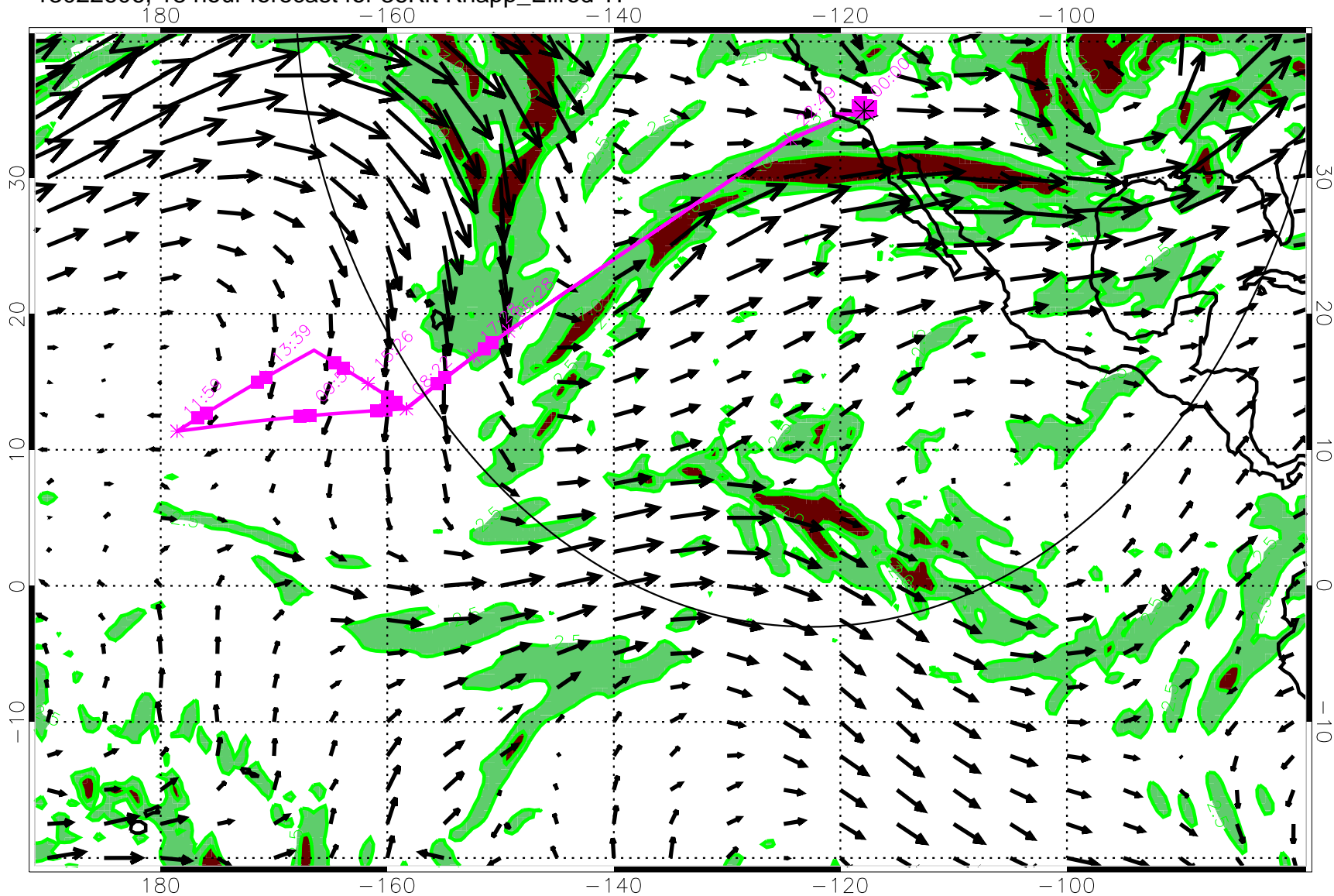
13022606, 18 hour forecast for 36Kft Knapp_Ellrod TI
