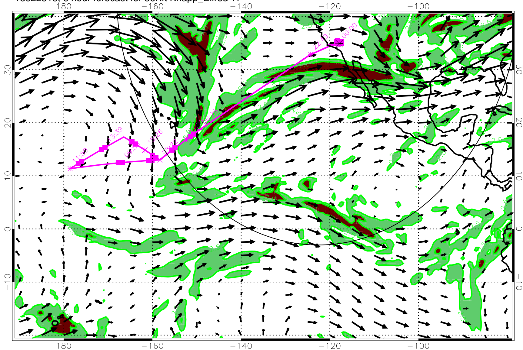
13022518, 6 hour forecast for 36Kft Knapp_Ellrod TI
