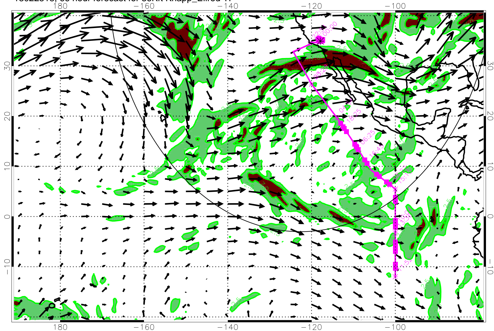
13022518, 66 hour forecast for 36Kft Knapp_Ellrod TI
