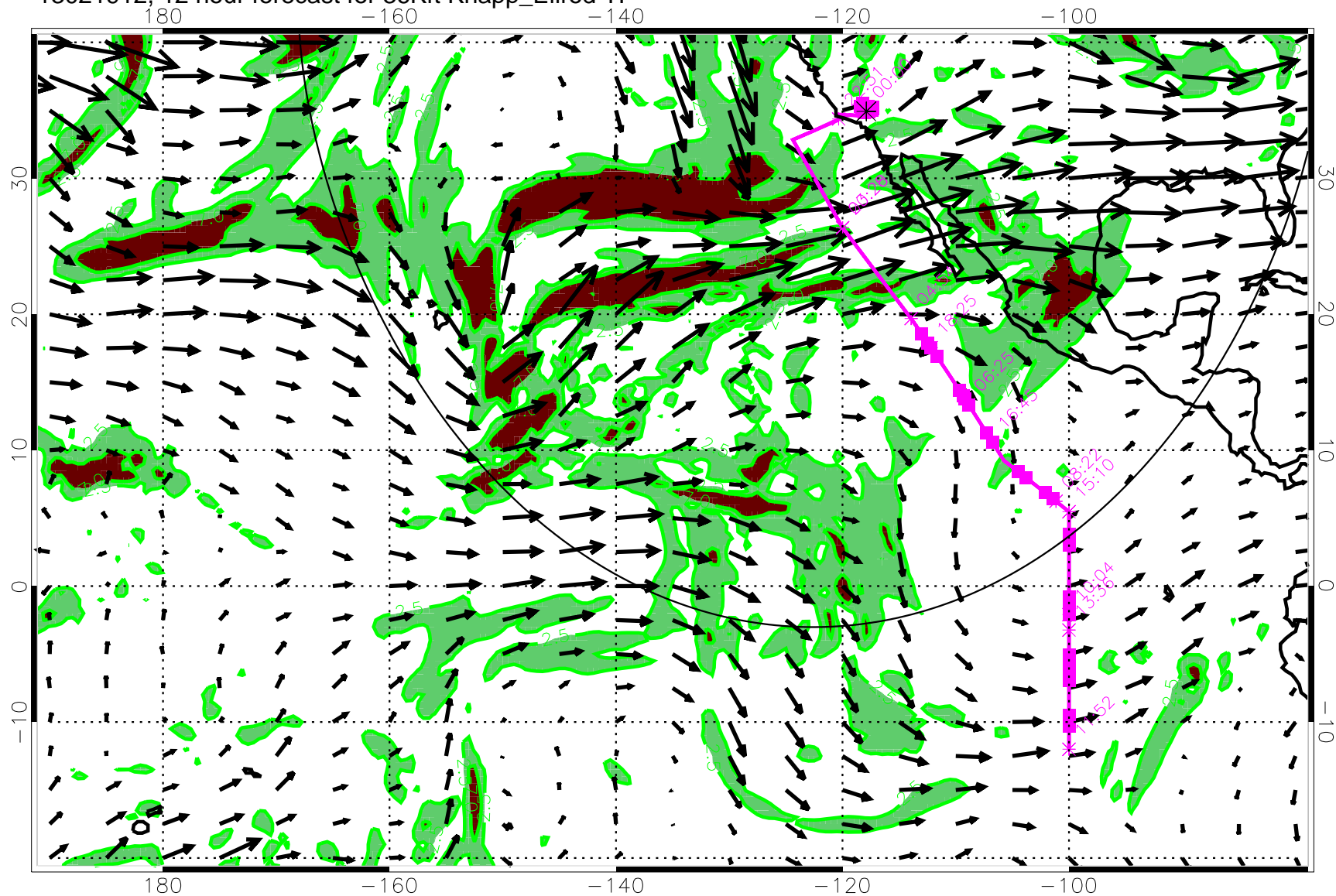
13021912, 12 hour forecast for 36Kft Knapp_Ellrod TI
