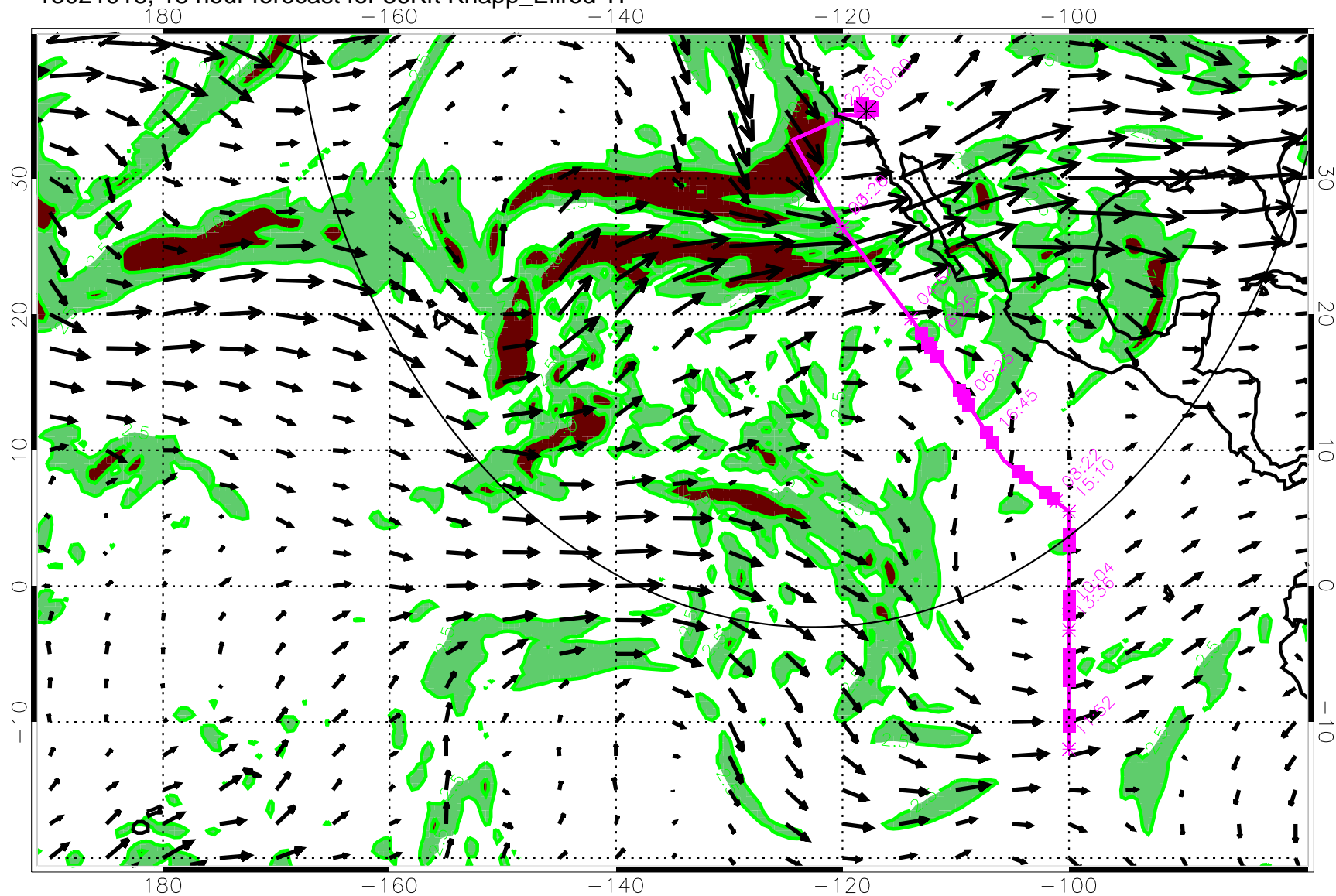
13021918, 18 hour forecast for 36Kft Knapp_Ellrod TI
