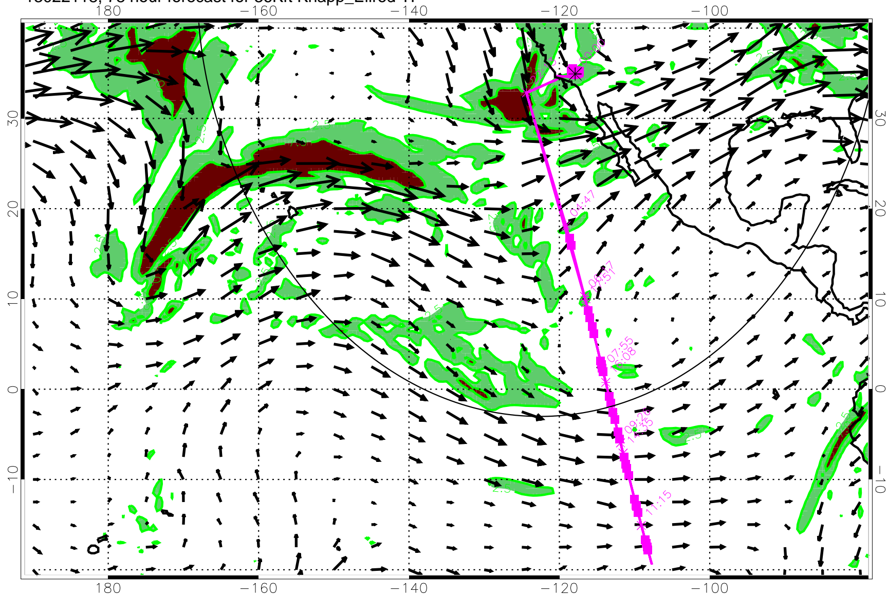
13022118, 78 hour forecast for 36Kft Knapp_Ellrod TI
