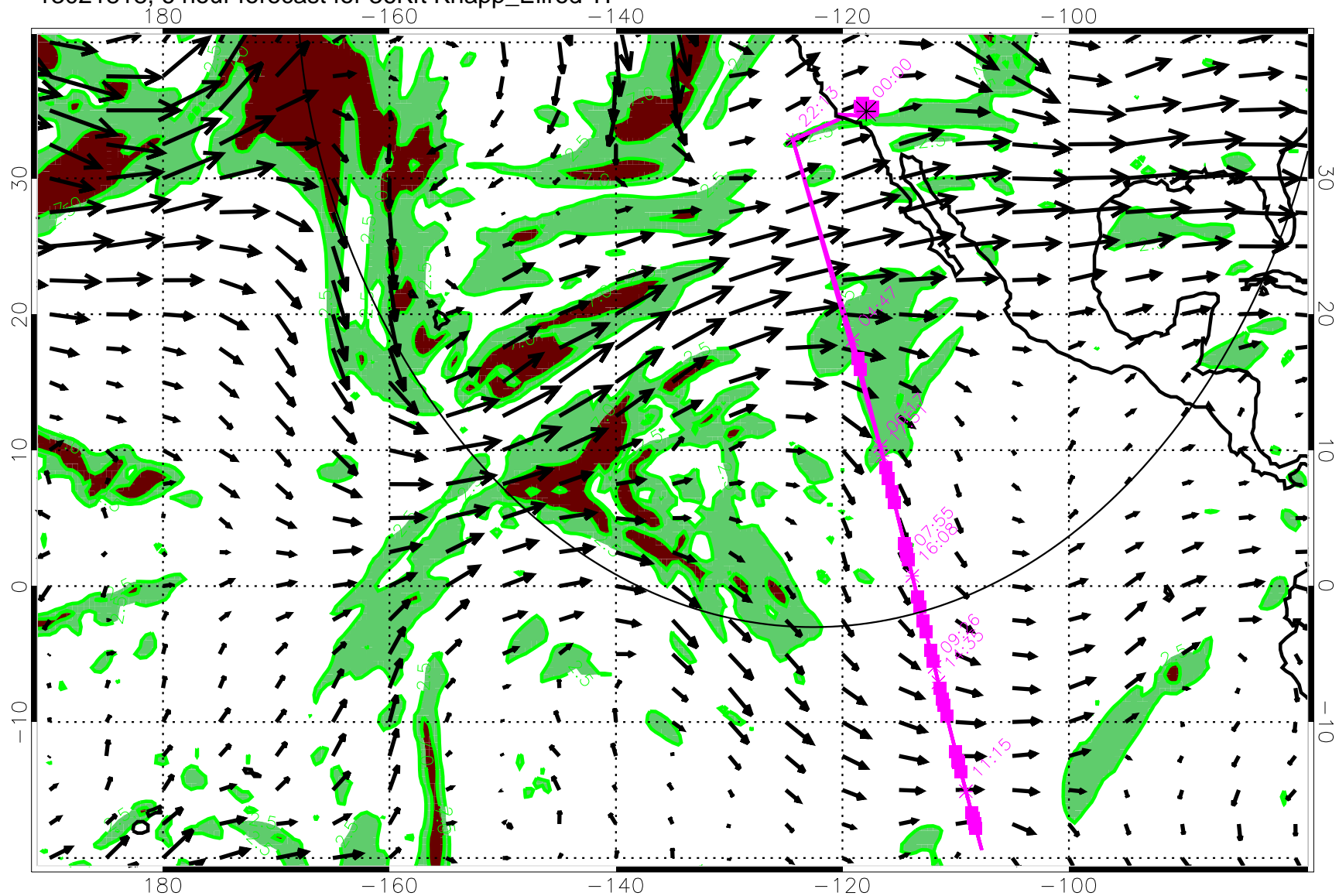
13021818, 6 hour forecast for 36Kft Knapp_Ellrod TI
