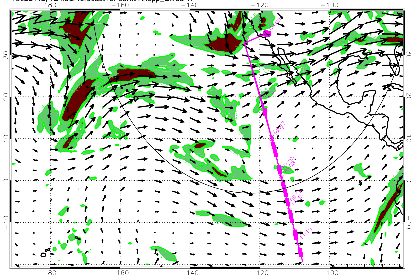
13022112, 72 hour forecast for 36Kft Knapp_Ellrod TI
