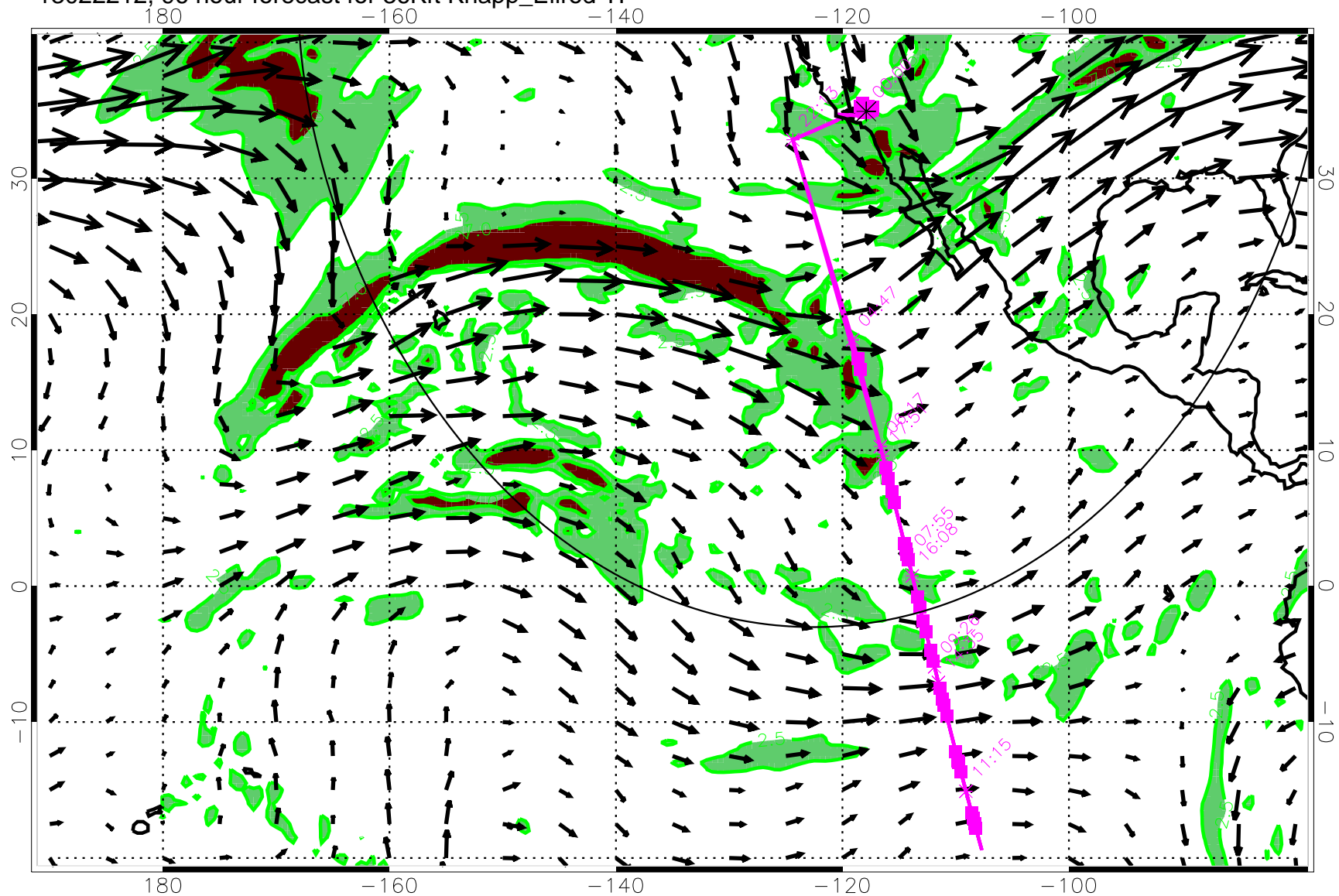
13022212, 96 hour forecast for 36Kft Knapp_Ellrod TI
