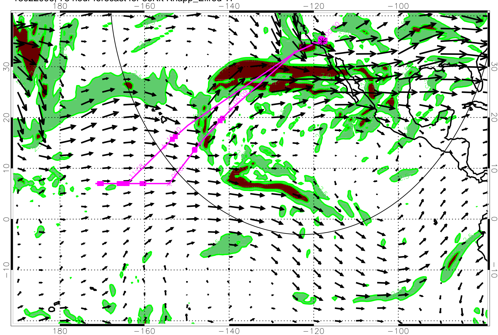
13022006, 78 hour forecast for 36Kft Knapp_Ellrod TI
