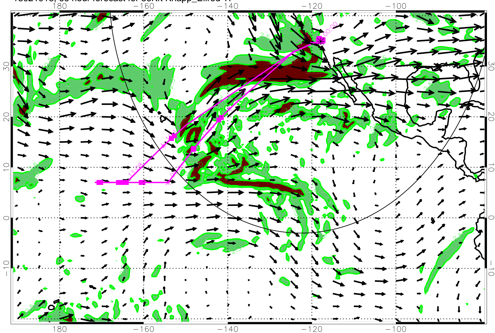
13021918, 66 hour forecast for 36Kft Knapp_Ellrod TI
