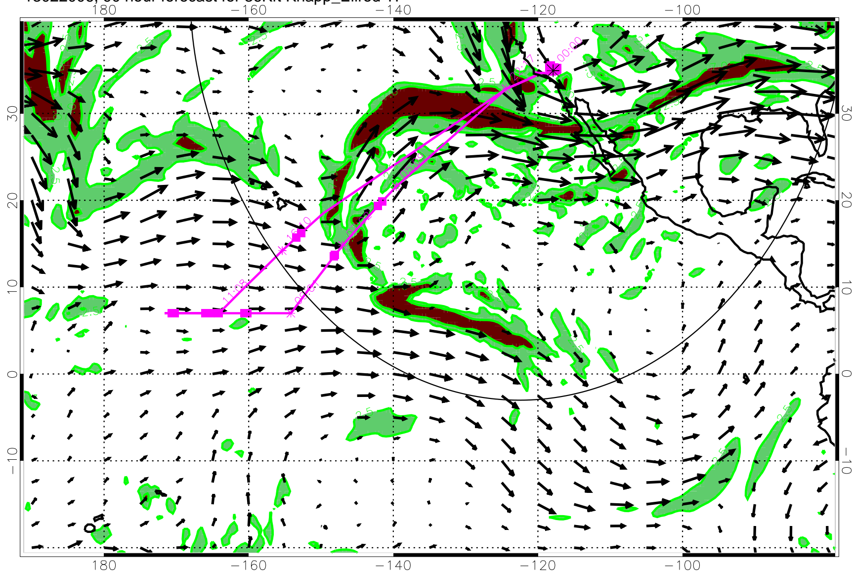
13022006, 90 hour forecast for 36Kft Knapp_Ellrod T1
