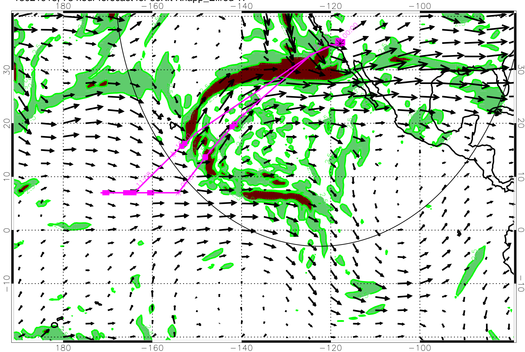
13021918, 78 hour forecast for 36Kft Knapp_Ellrod TI
