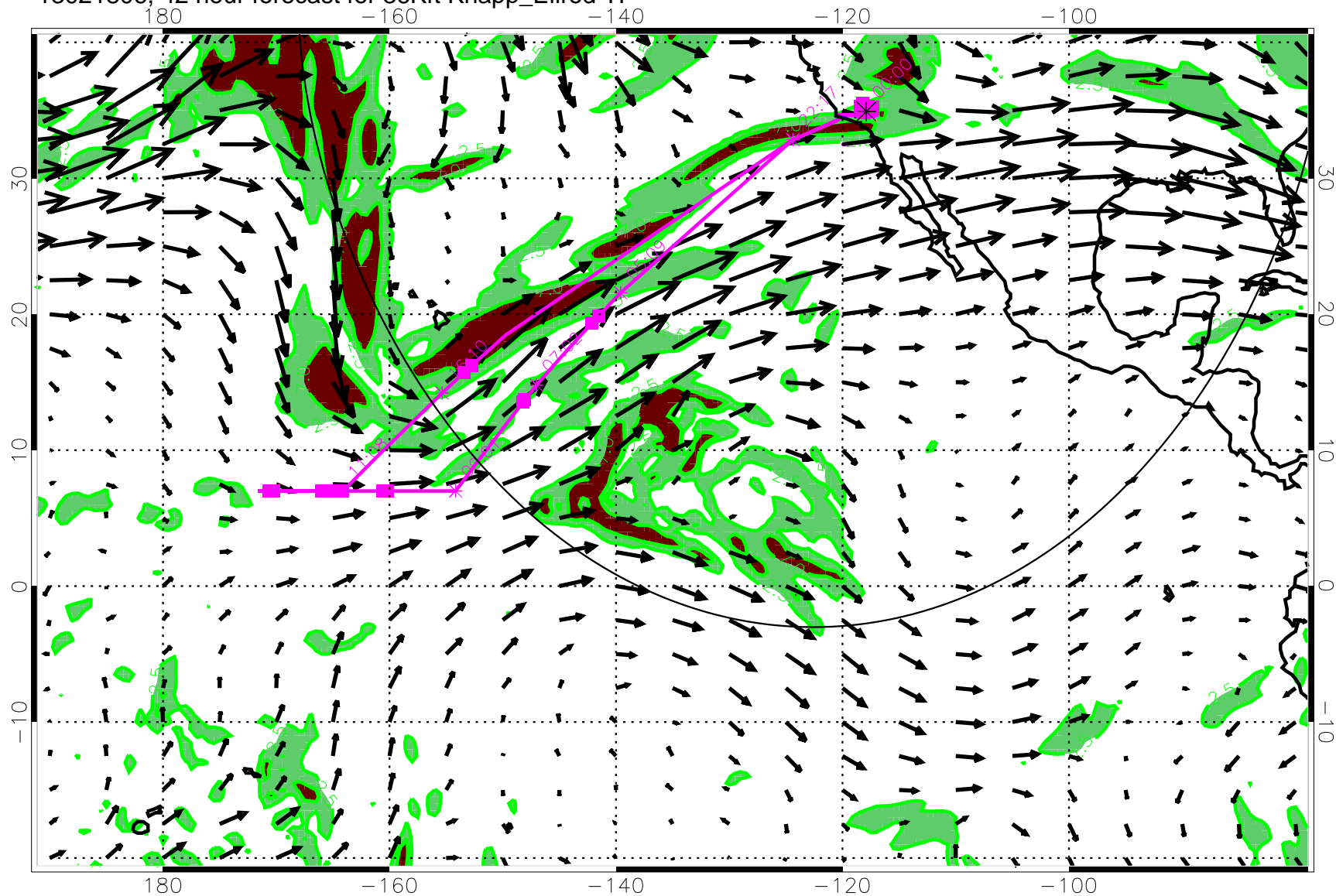
13021806, 42 hour forecast for 36Kft Knapp_Ellrod TI
