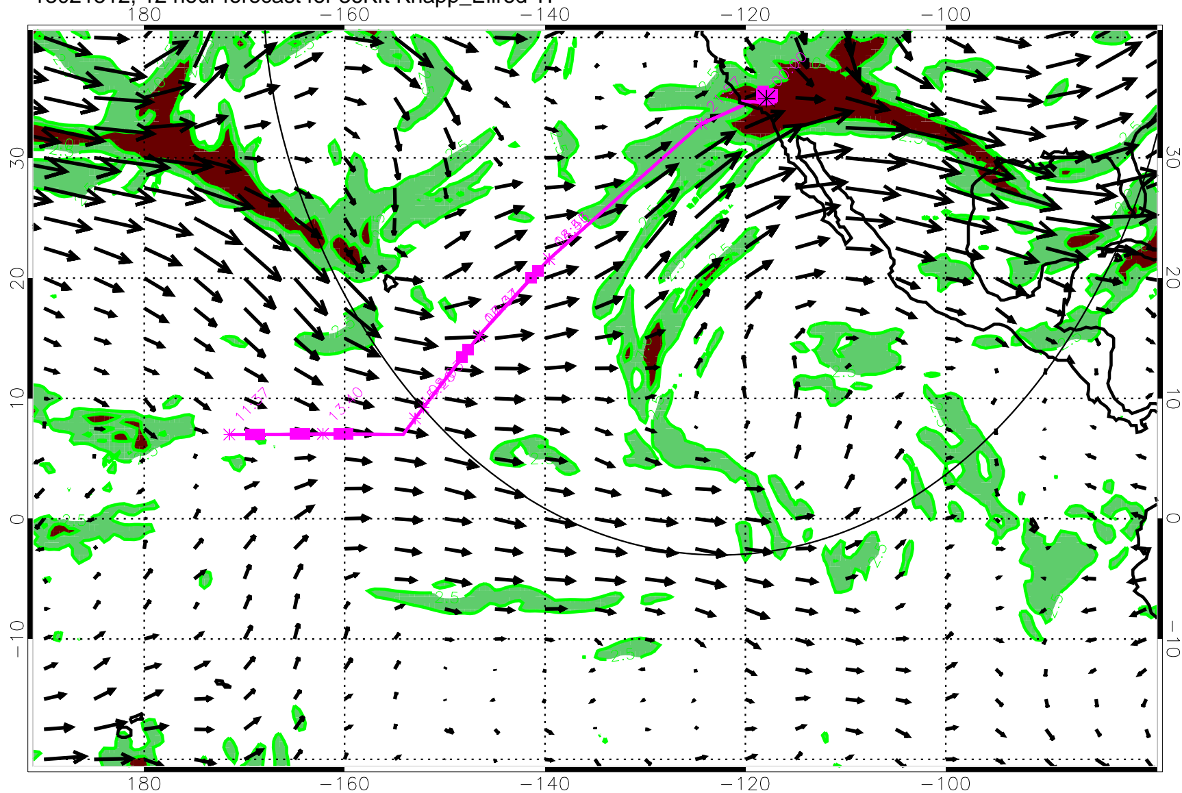
13021512, 12 hour forecast for 36Kft Knapp_Ellrod TI
