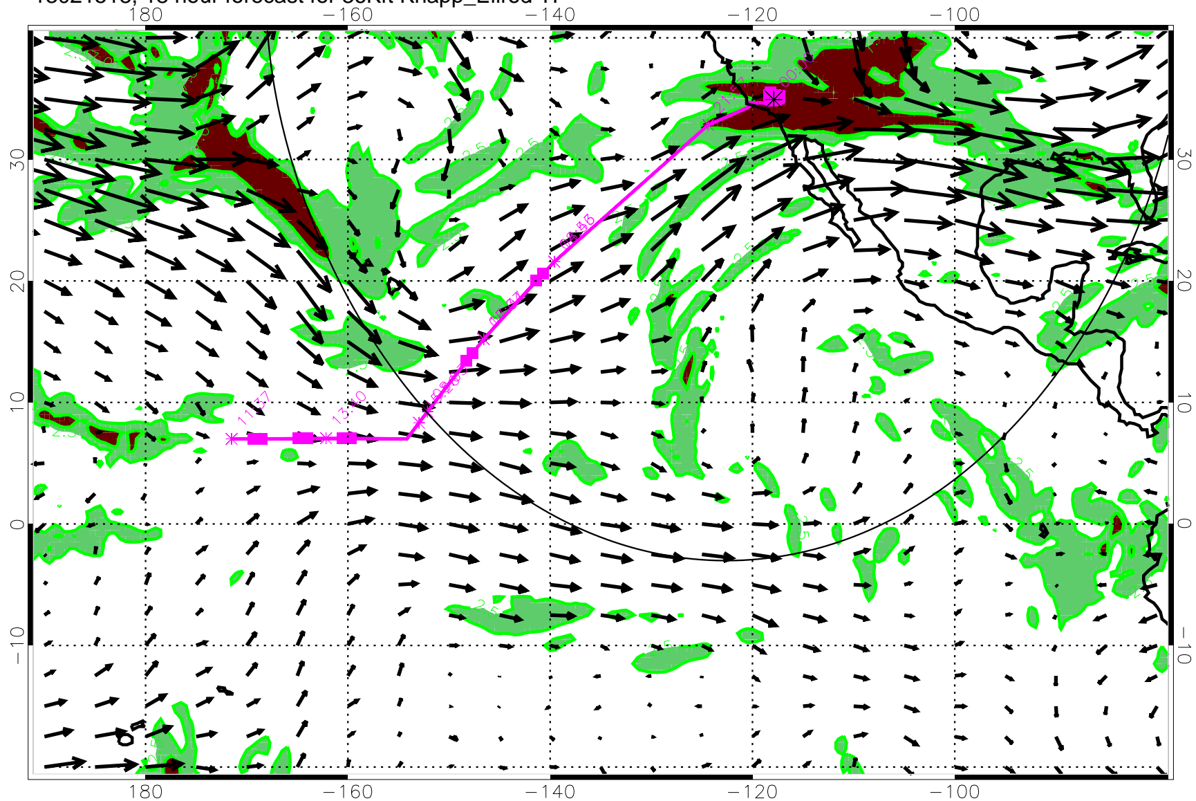
13021518, 18 hour forecast for 36Kft Knapp_Ellrod TI
