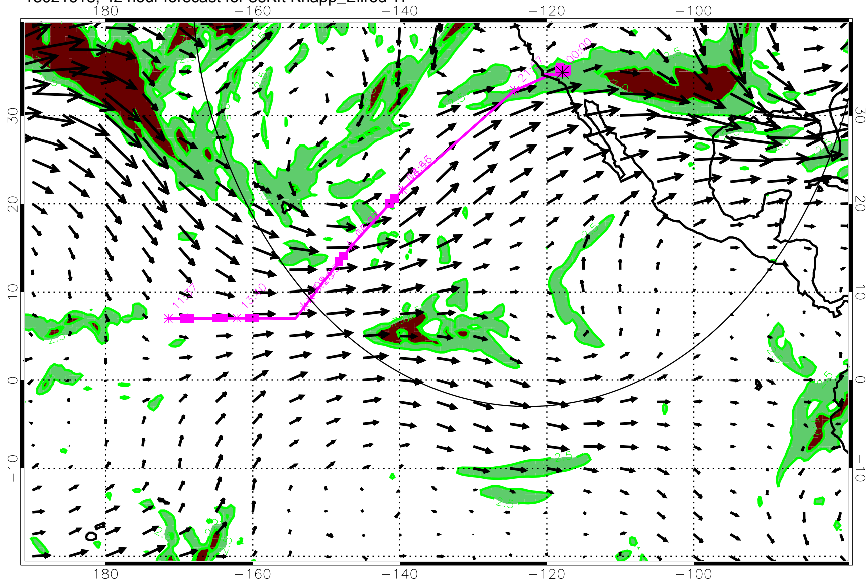
13021618, 42 hour forecast for 36Kft Knapp_Ellrod TI
