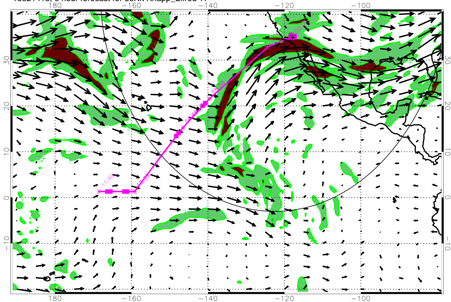
13021418, 6 hour forecast for 36Kft Knapp_Ellrod TI
