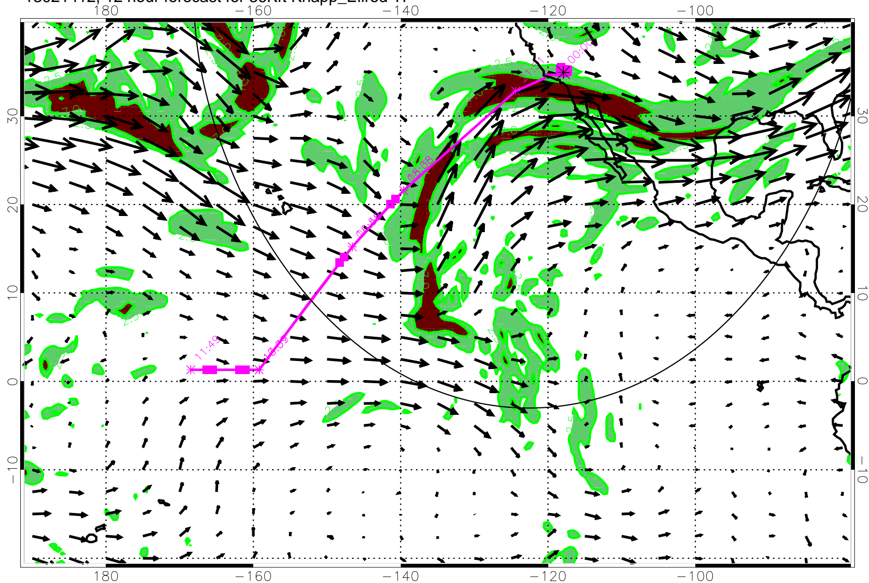
13021412, 12 hour forecast for 36Kft Knapp_Ellrod TI
