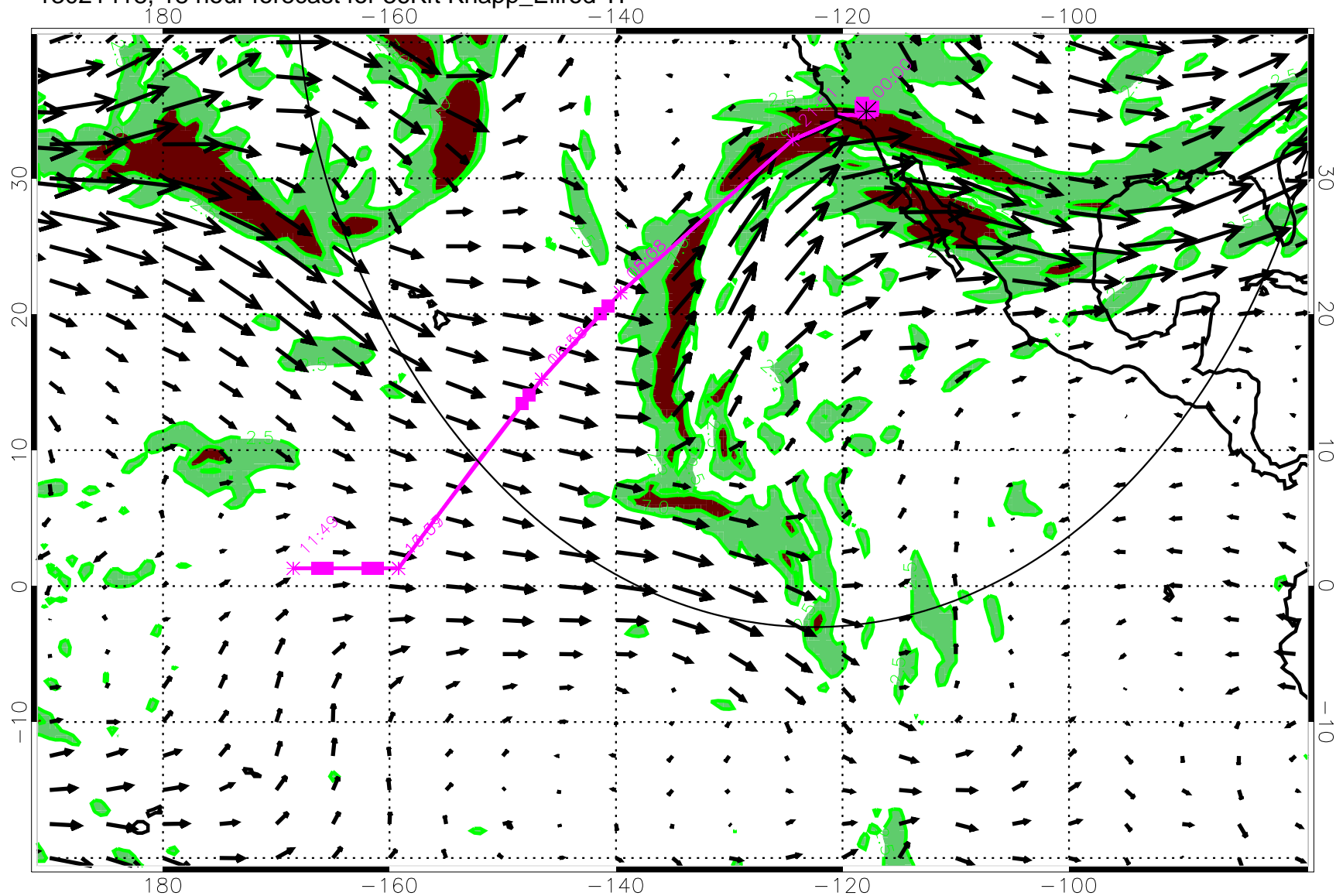
13021418, 18 hour forecast for 36Kft Knapp_Ellrod TI
