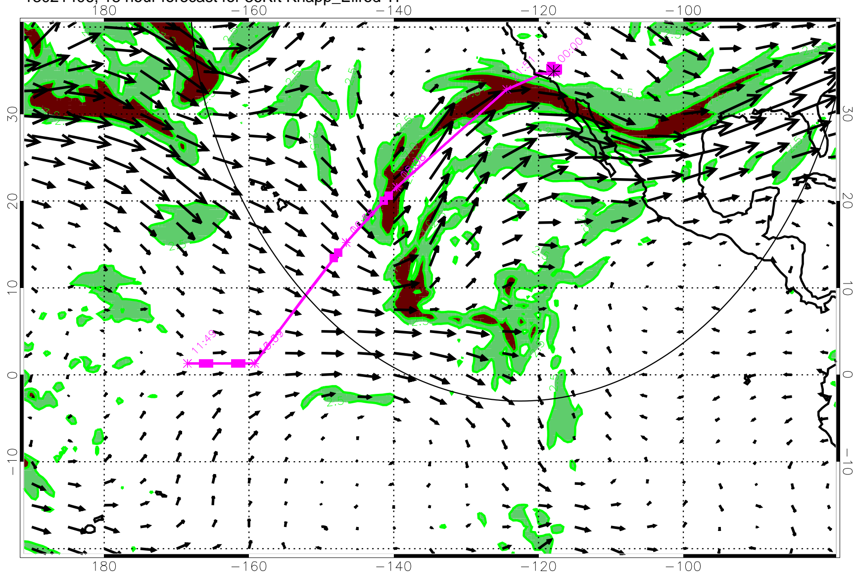
13021406, 18 hour forecast for 36Kft Knapp_Ellrod TI
