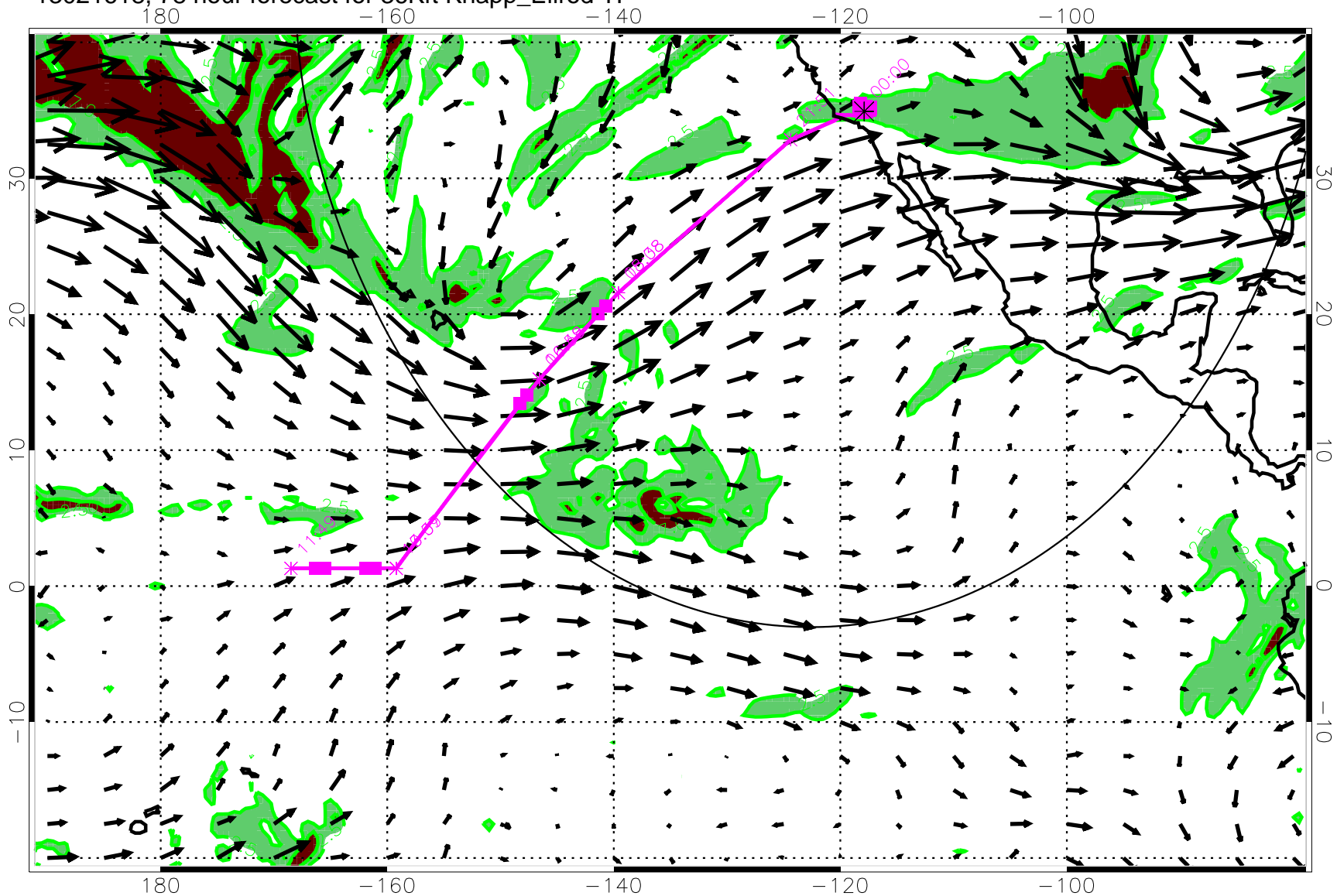
13021618, 78 hour forecast for 36Kft Knapp_Ellrod TI
