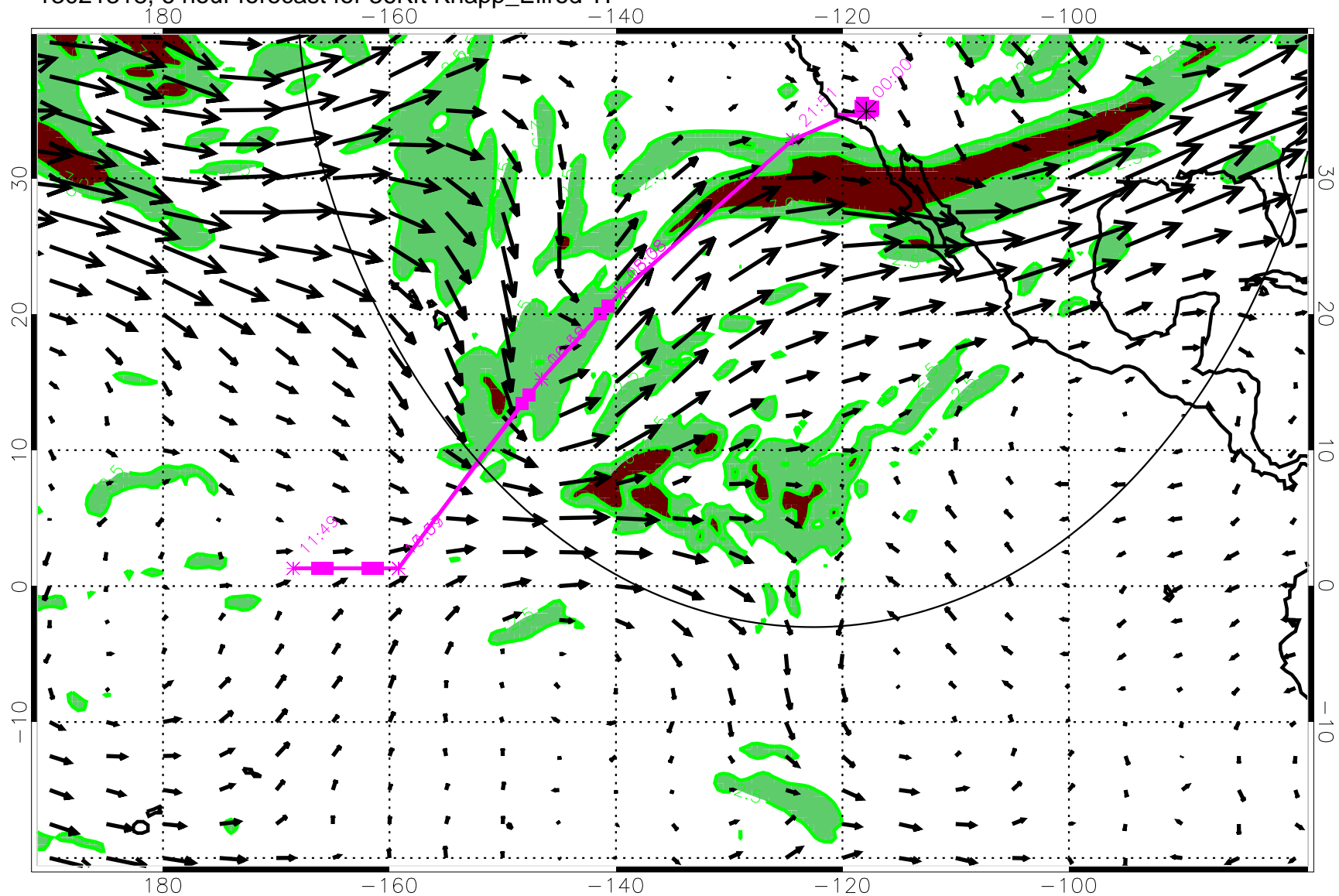
13021318, 6 hour forecast for 36Kft Knapp_Ellrod TI
