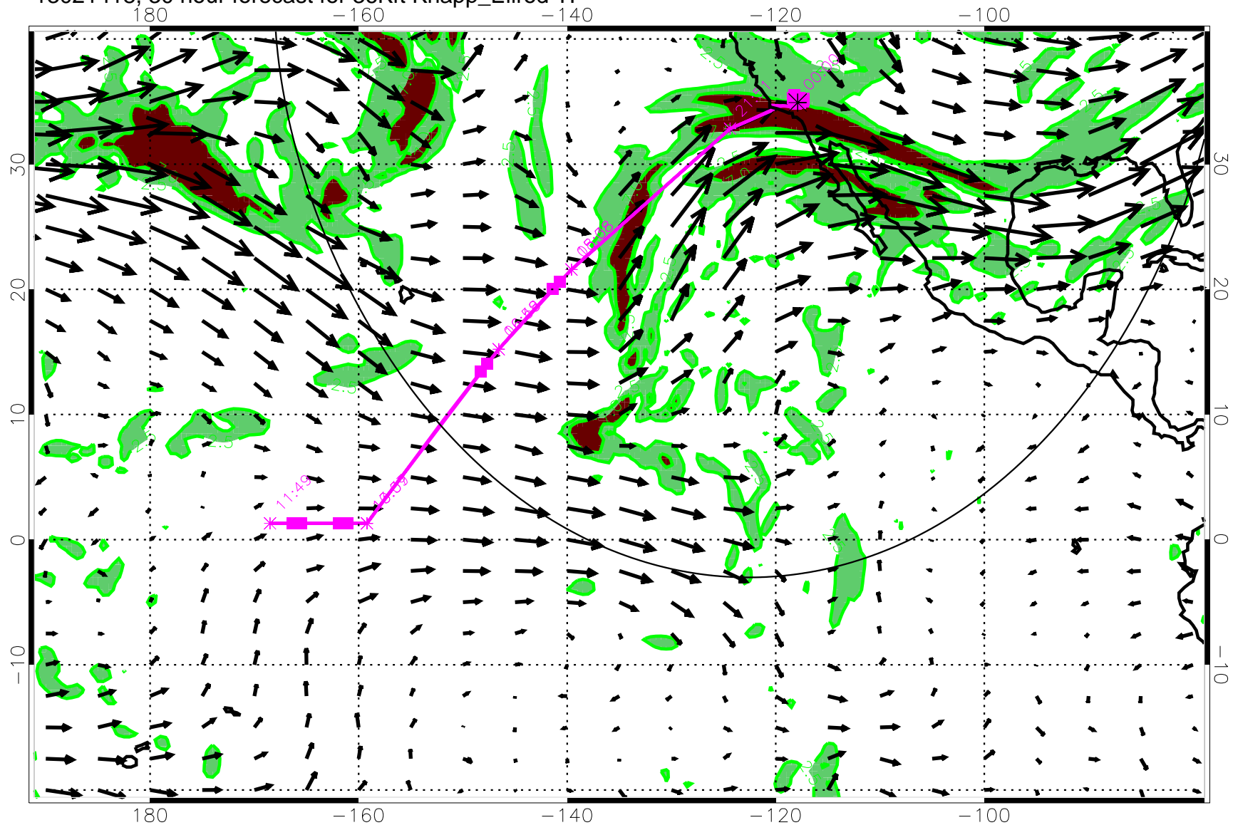
13021418, 30 hour forecast for 36Kft Knapp_Ellrod T1
