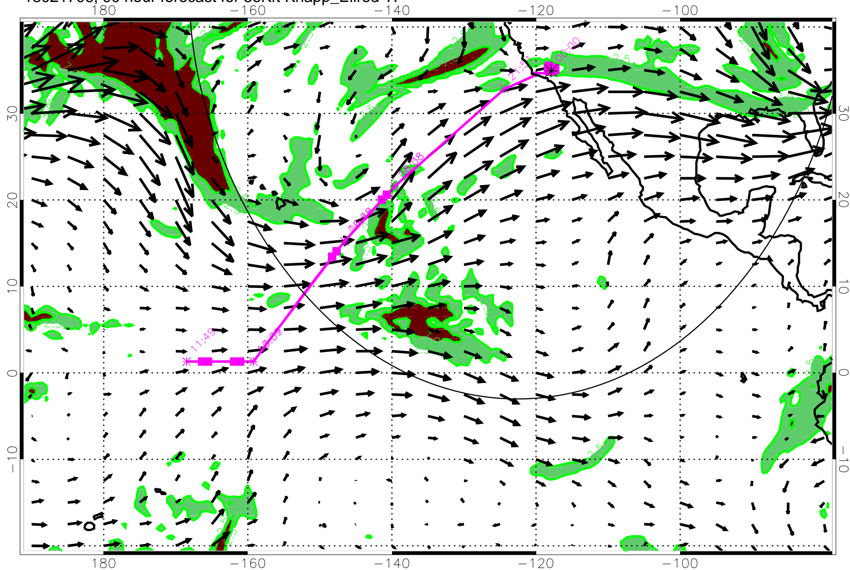
13021706, 90 hour forecast for 36Kft Knapp_Ellrod TI
