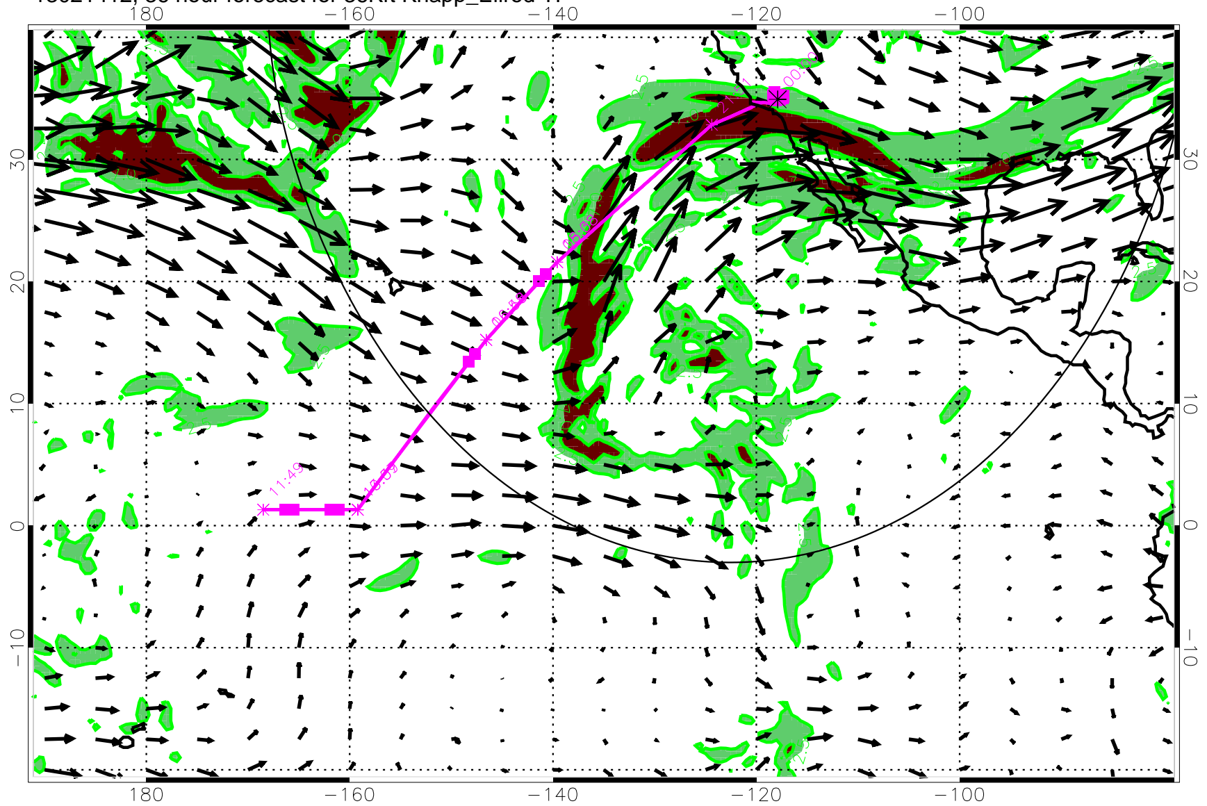
13021412, 36 hour forecast for 36Kft Knapp_Ellrod TI
