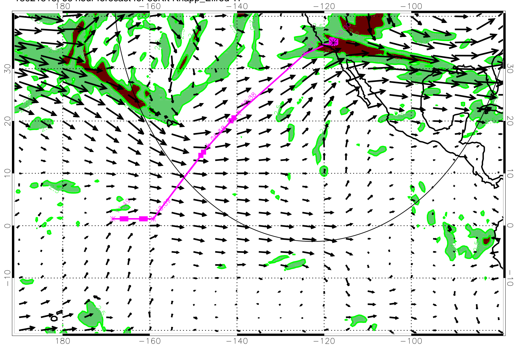
13021518, 66 hour forecast for 36Kft Knapp_Ellrod TI
