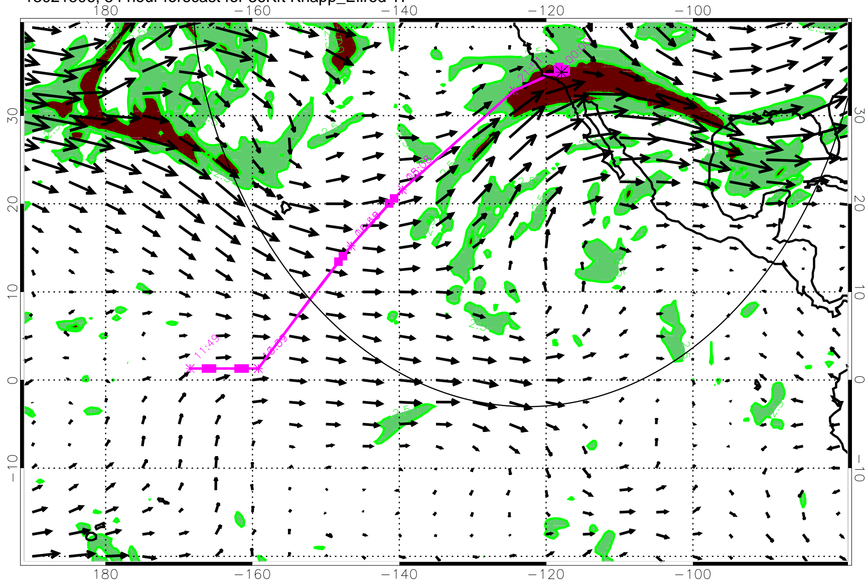
13021506, 54 hour forecast for 36Kft Knapp_Ellrod T1
