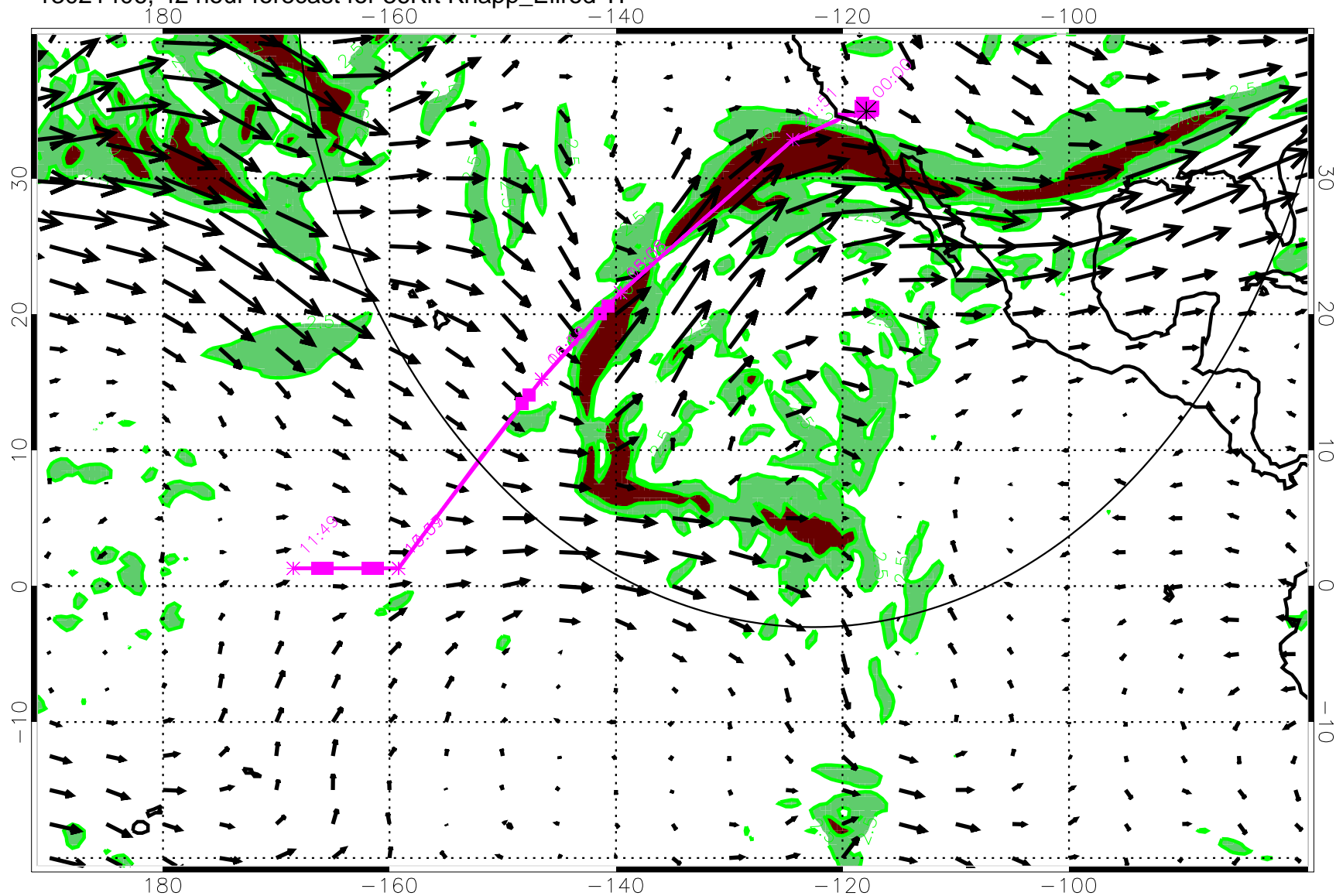
13021406, 42 hour forecast for 36Kft Knapp_Ellrod TI
