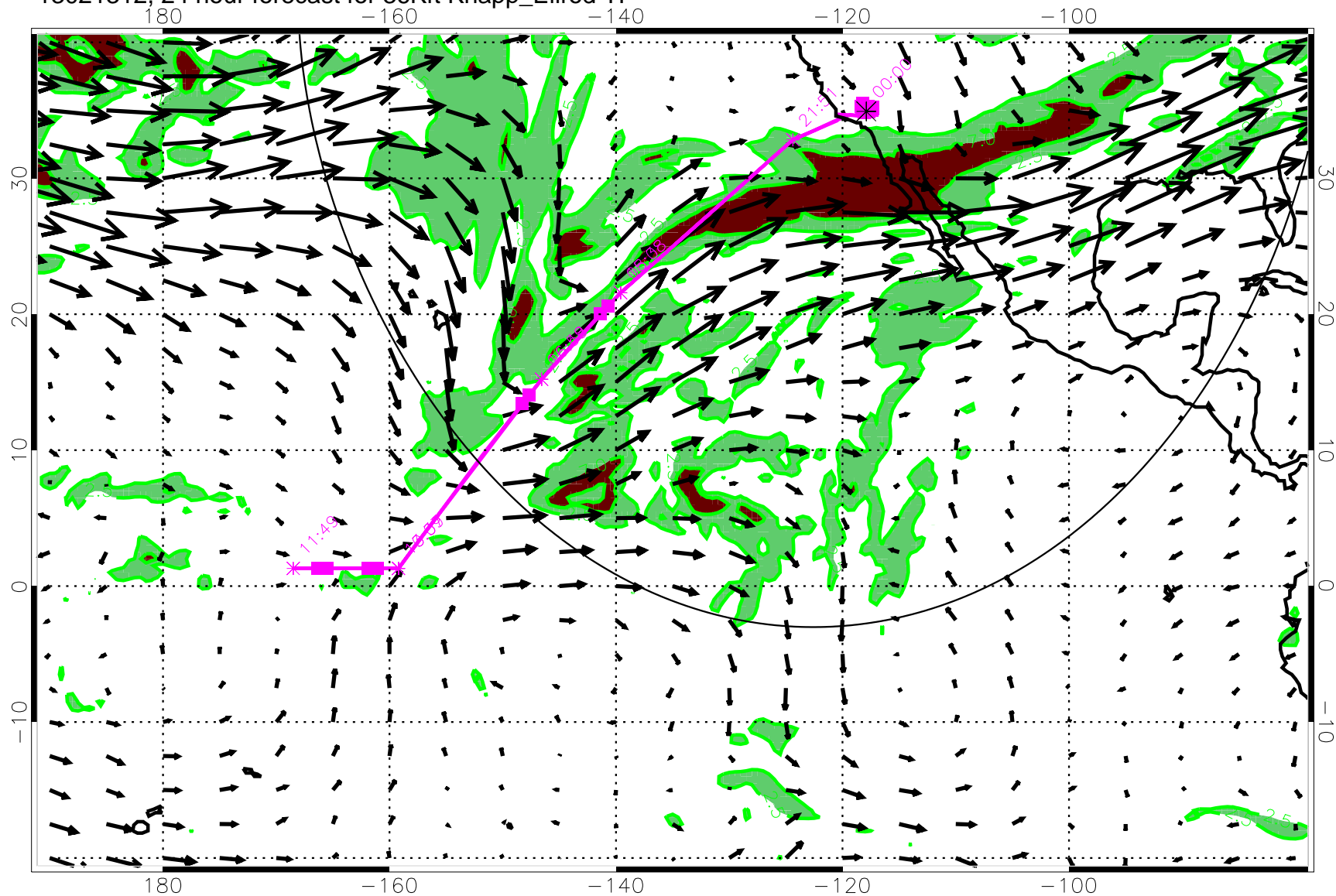
13021312, 24 hour forecast for 36Kft Knapp_Ellrod TI
