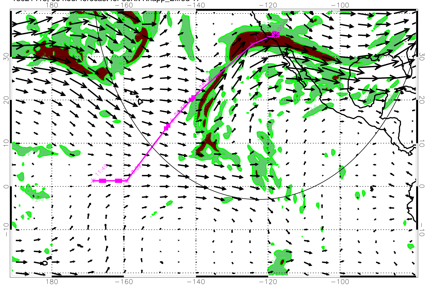
13021418, 66 hour forecast for 36Kft Knapp_Ellrod T1
