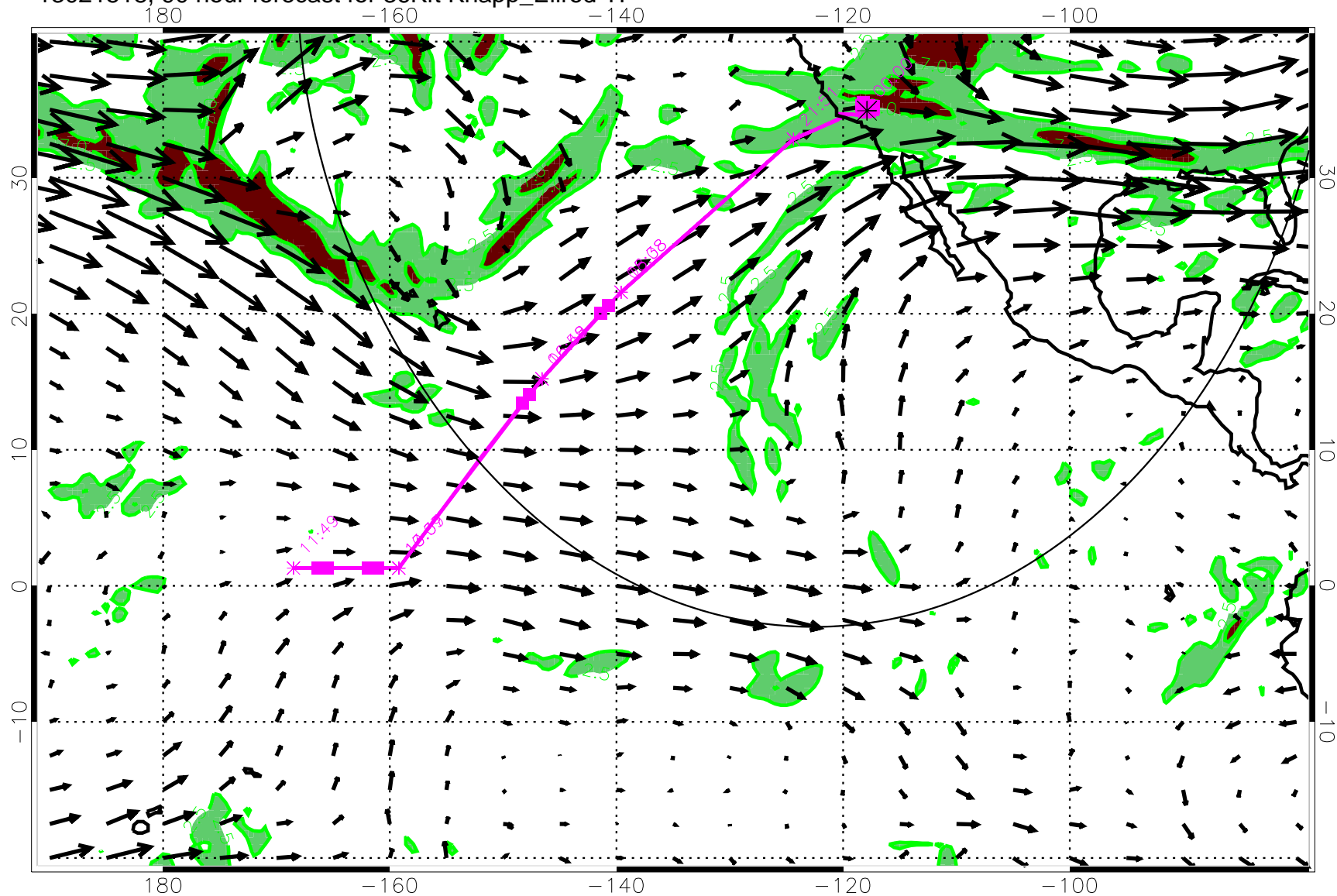
13021518, 90 hour forecast for 36Kft Knapp_Ellrod TI
