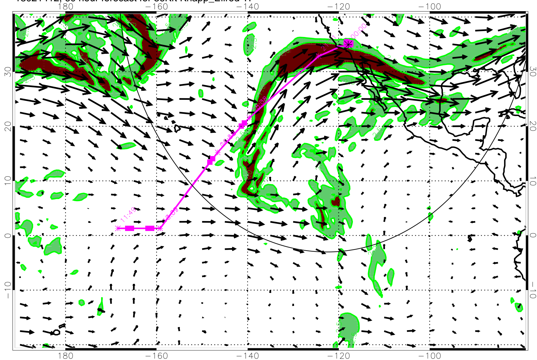
13021412, 60 hour forecast for 36Kft Knapp_Ellrod TI
