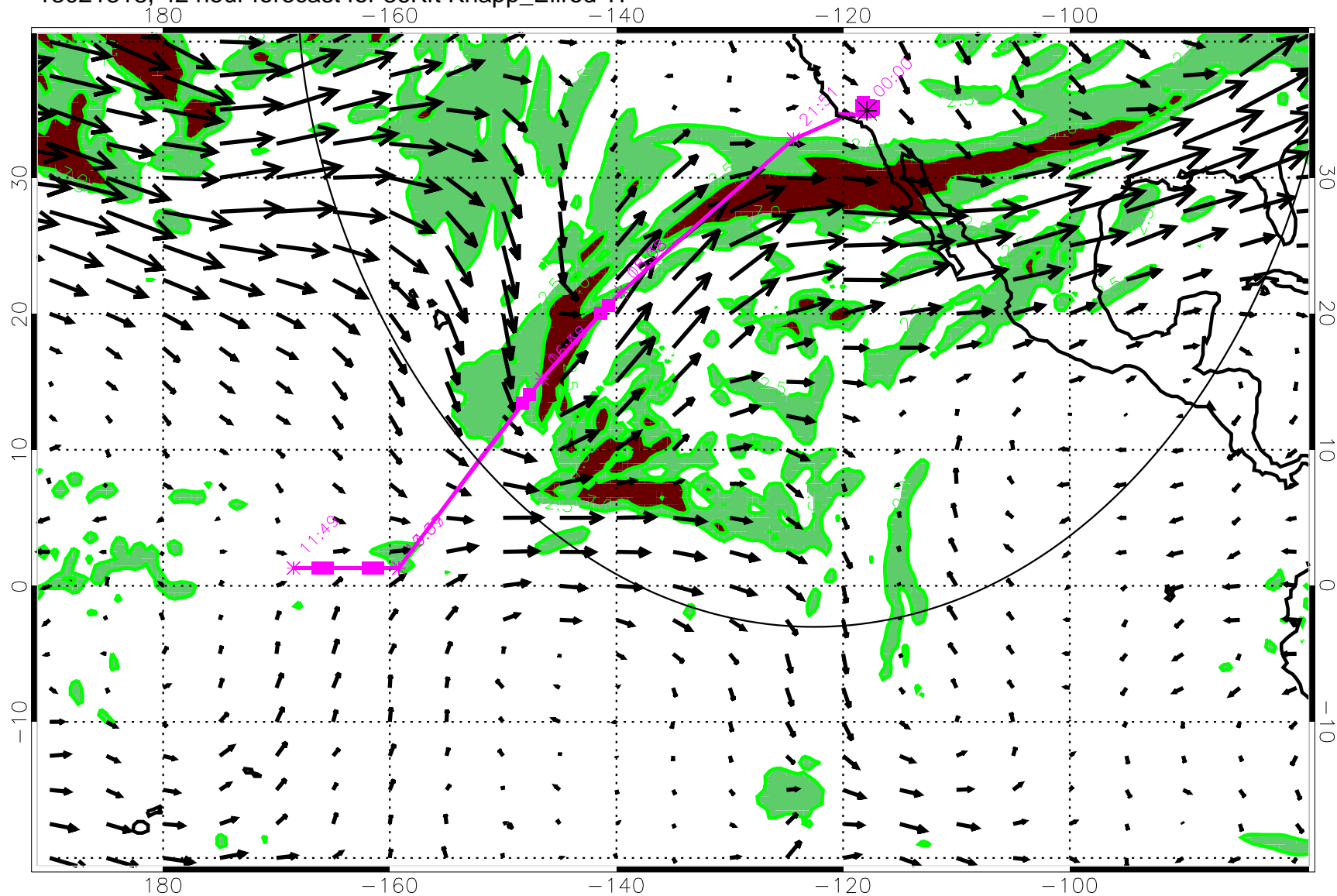
13021318, 42 hour forecast for 36Kft Knapp_Ellrod TI
