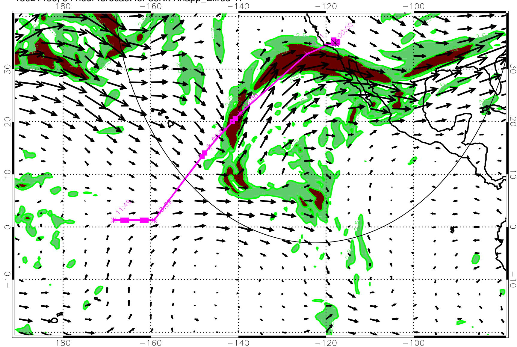
13021406, 54 hour forecast for 36Kft Knapp_Ellrod TI
