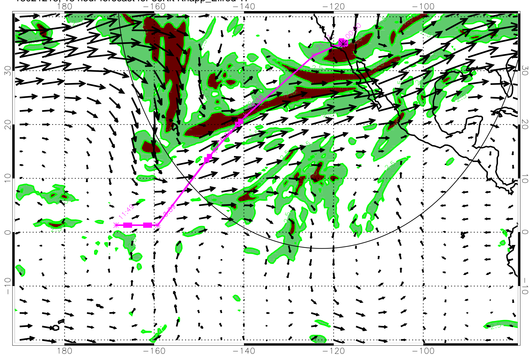
13021218, 18 hour forecast for 36Kft Knapp_Ellrod TI
