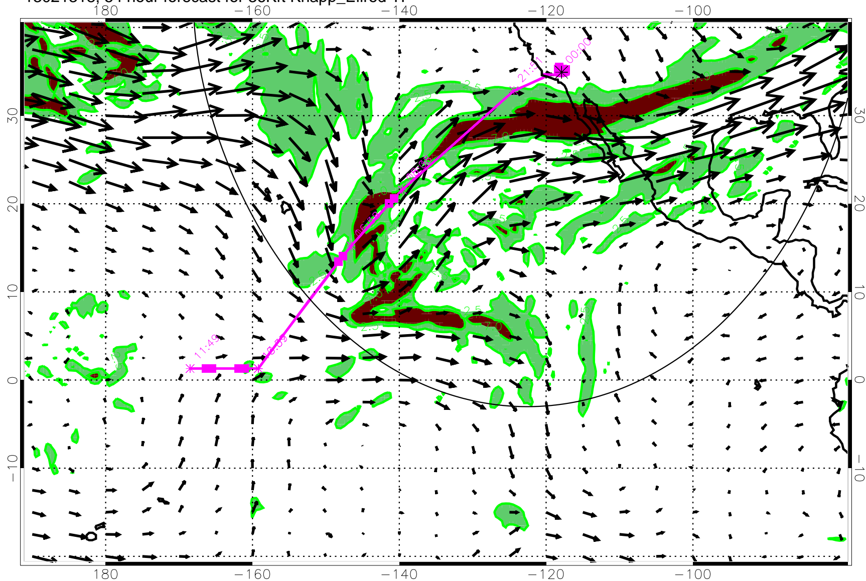
13021318, 54 hour forecast for 36Kft Knapp_Ellrod TI
