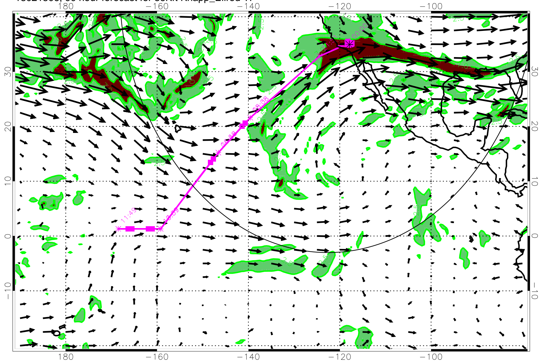
13021506, 90 hour forecast for 36Kft Knapp_Ellrod T1
