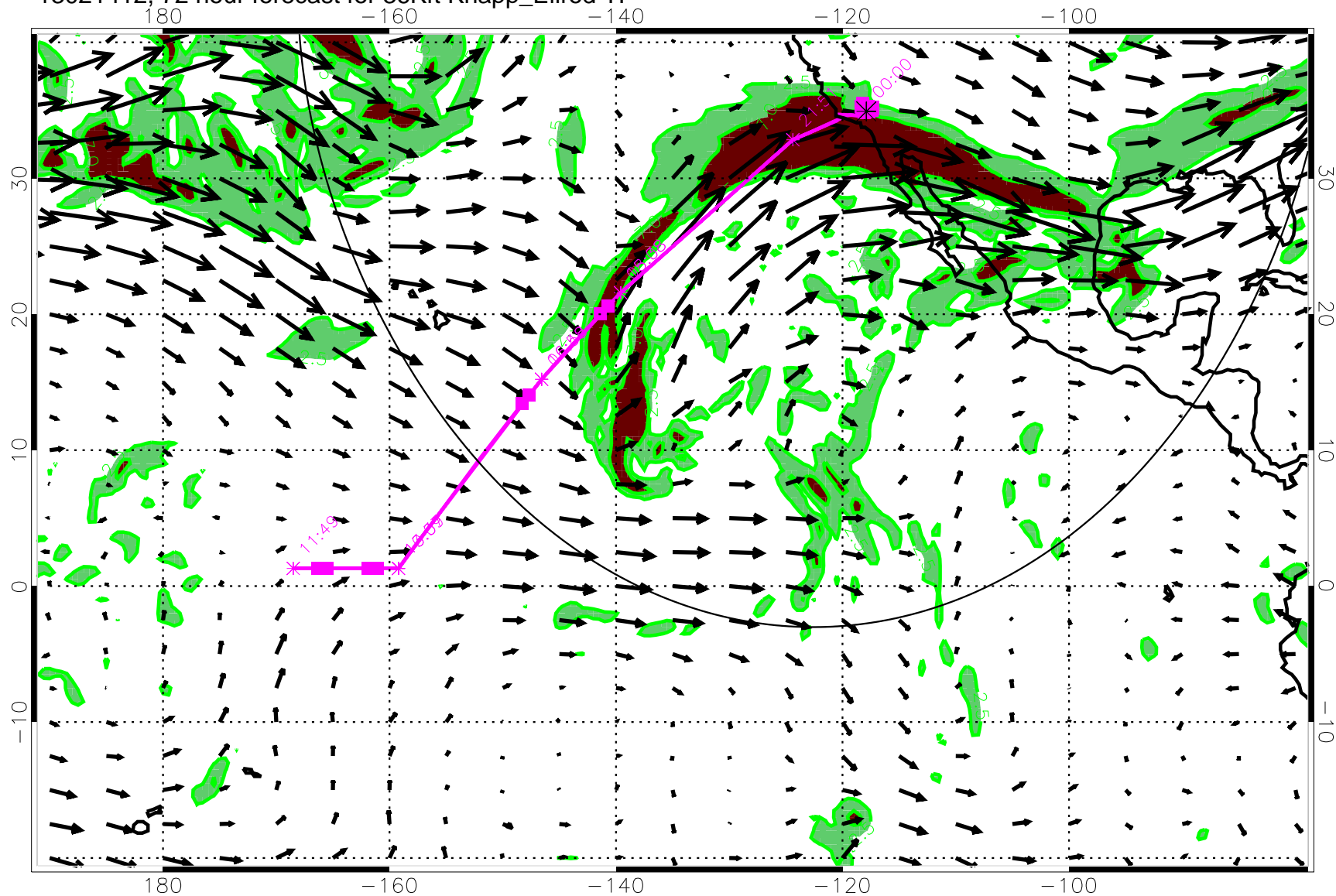
13021412, 72 hour forecast for 36Kft Knapp_Ellrod TI
