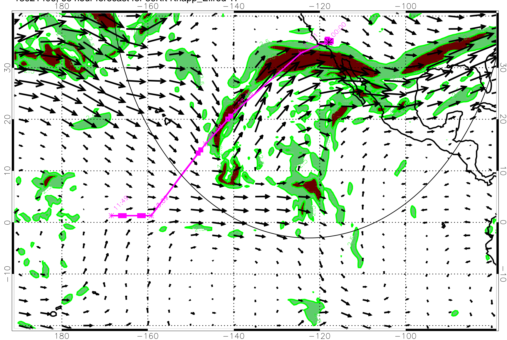
13021406, 66 hour forecast for 36Kft Knapp_Ellrod TI
