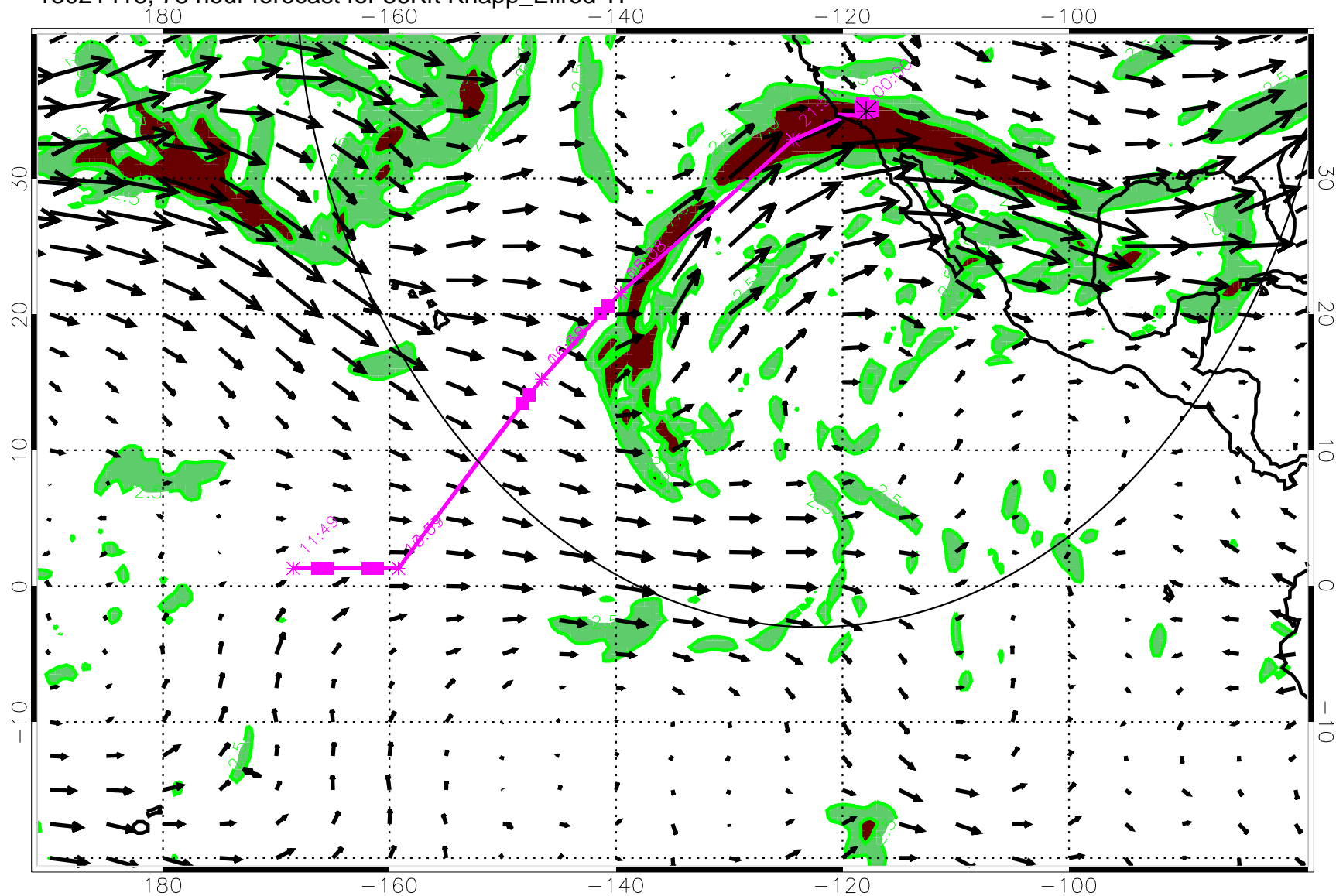
13021418, 78 hour forecast for 36Kft Knapp_Ellrod TI
