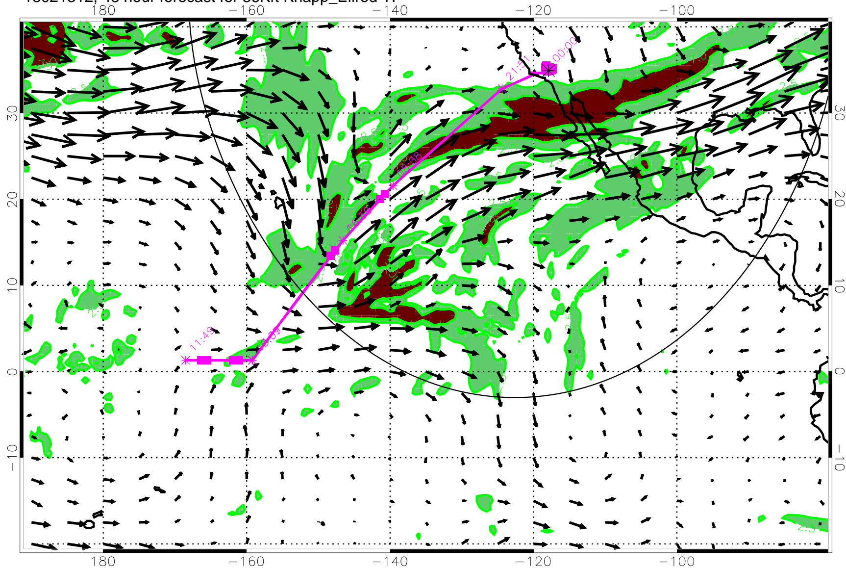
13021312, 48 hour forecast for 36Kft Knapp_Ellrod TI
