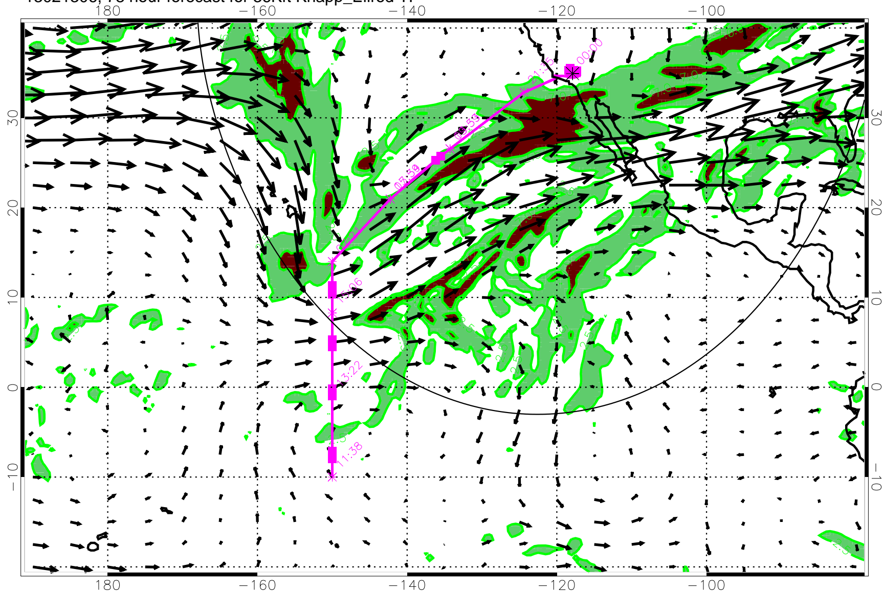
13021306, 78 hour forecast for 36Kft Knapp_Ellrod TI
