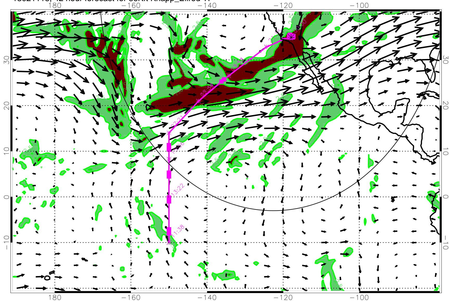
13021118, 42 hour forecast for 36Kft Knapp_Ellrod TI
